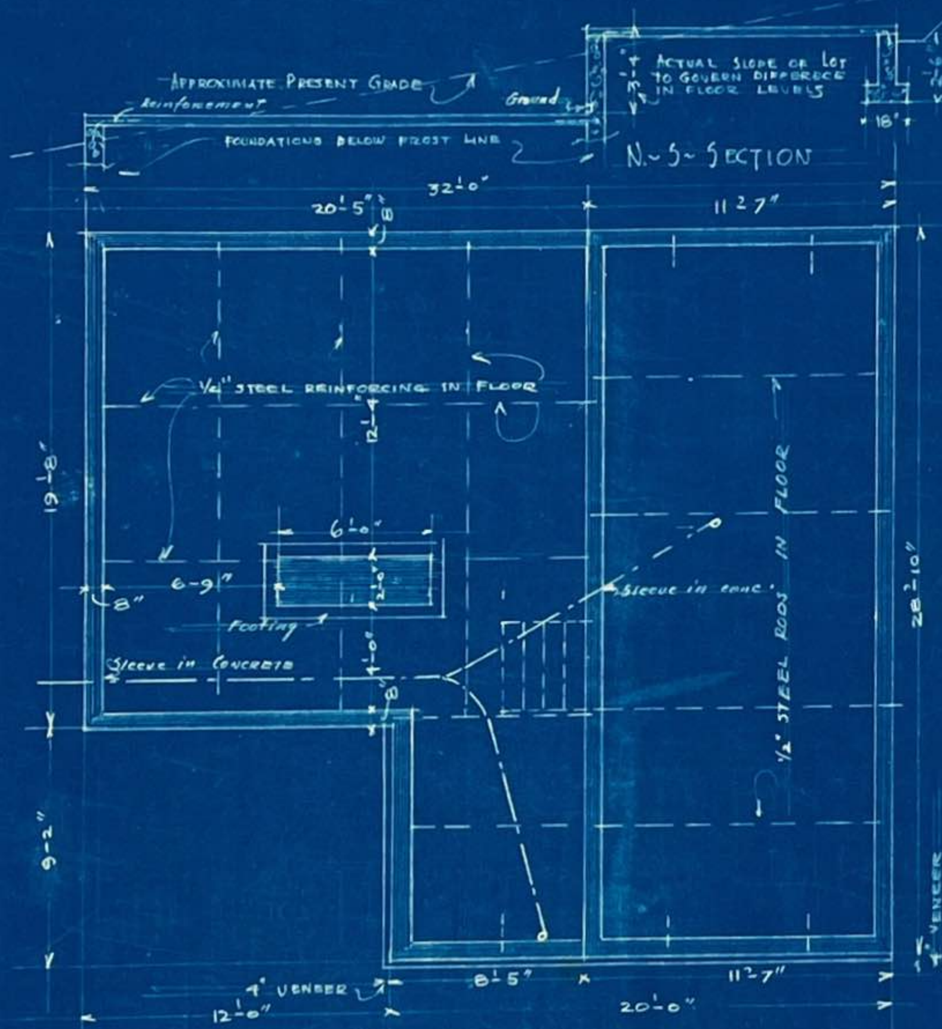
FOUNDATION PLAN
