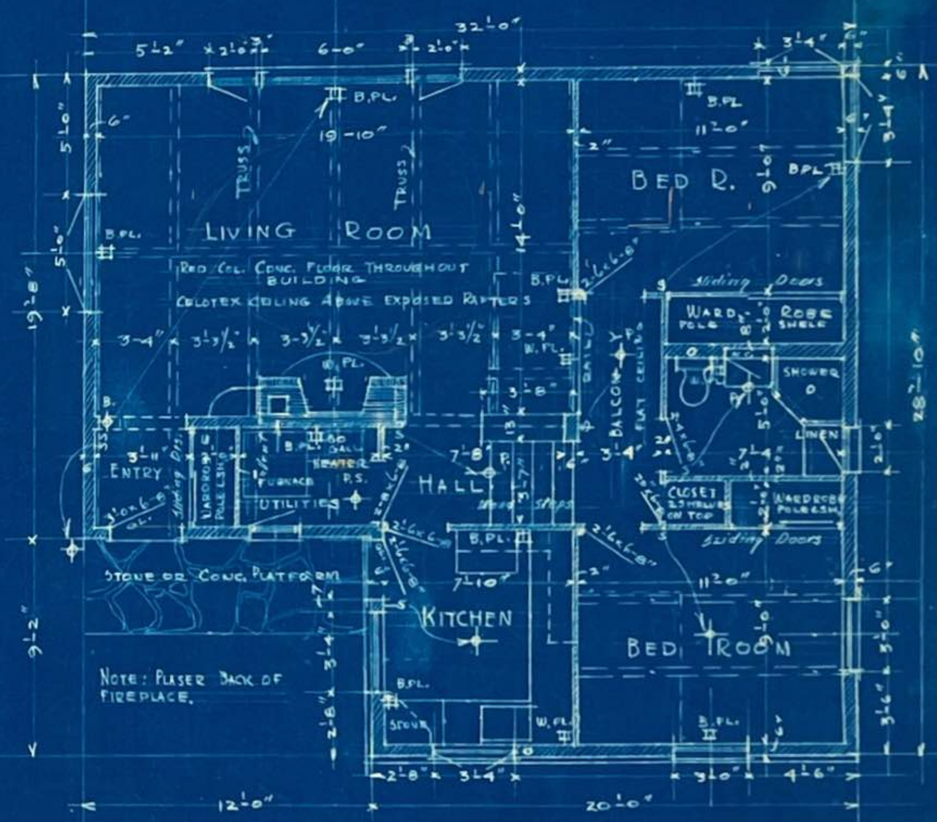
FLOOR PLAN
