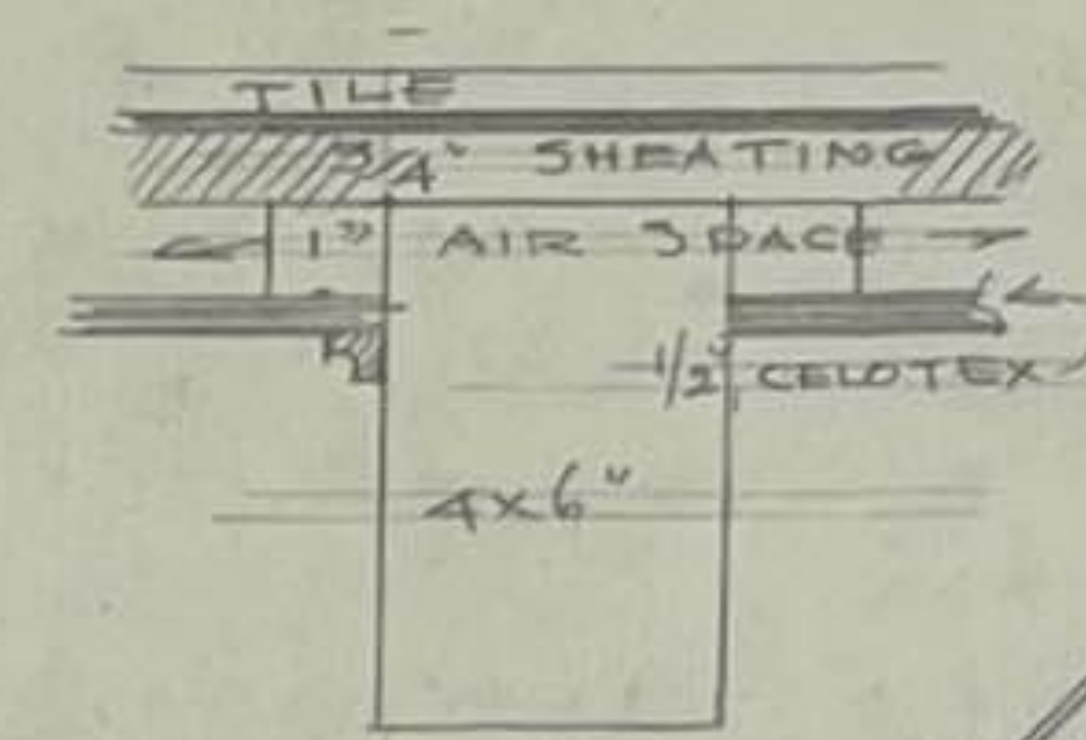
LIVING AND N. BED ROOM ROOF BEAMS
