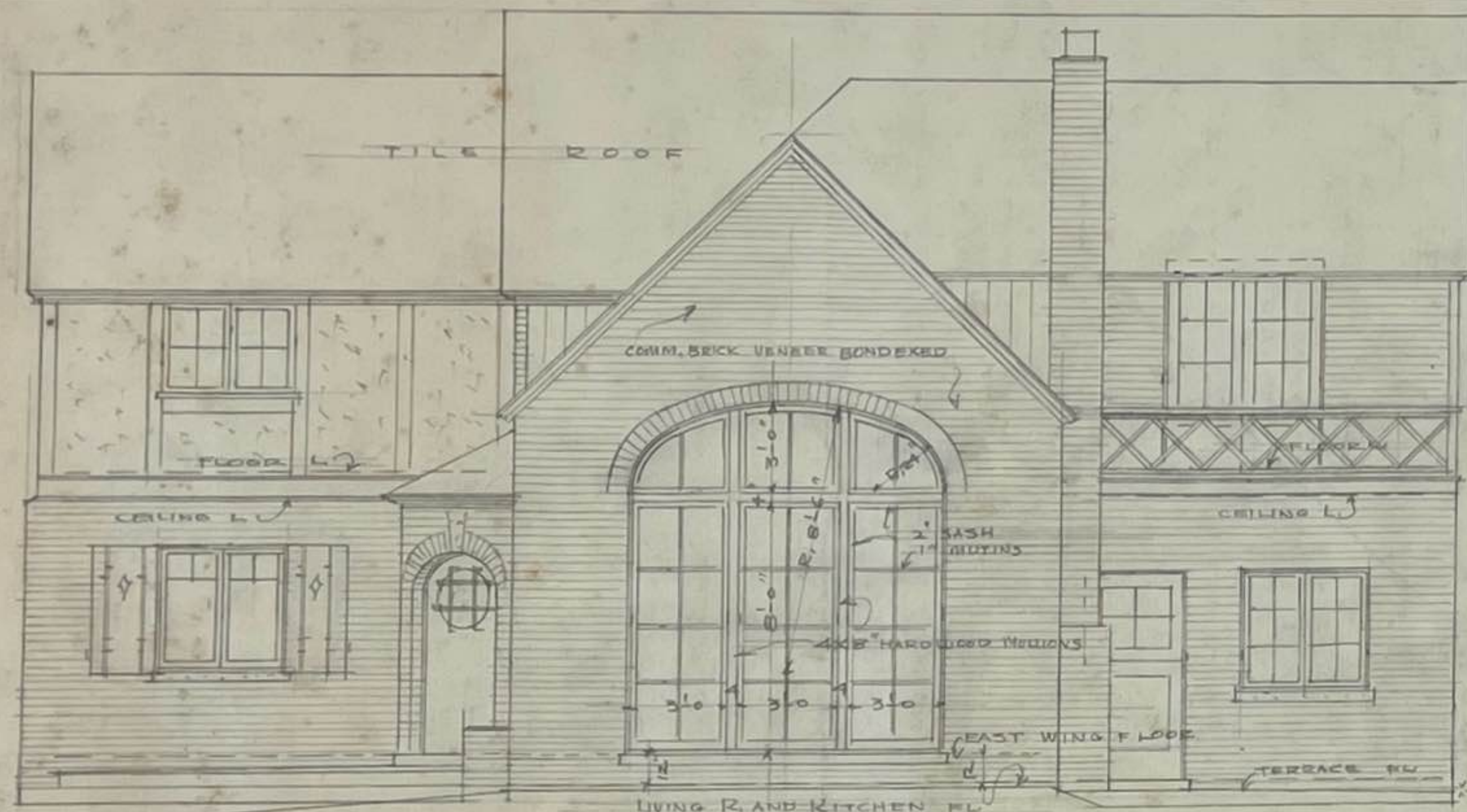
WEST (LAKE FRONT) ELEVATION
