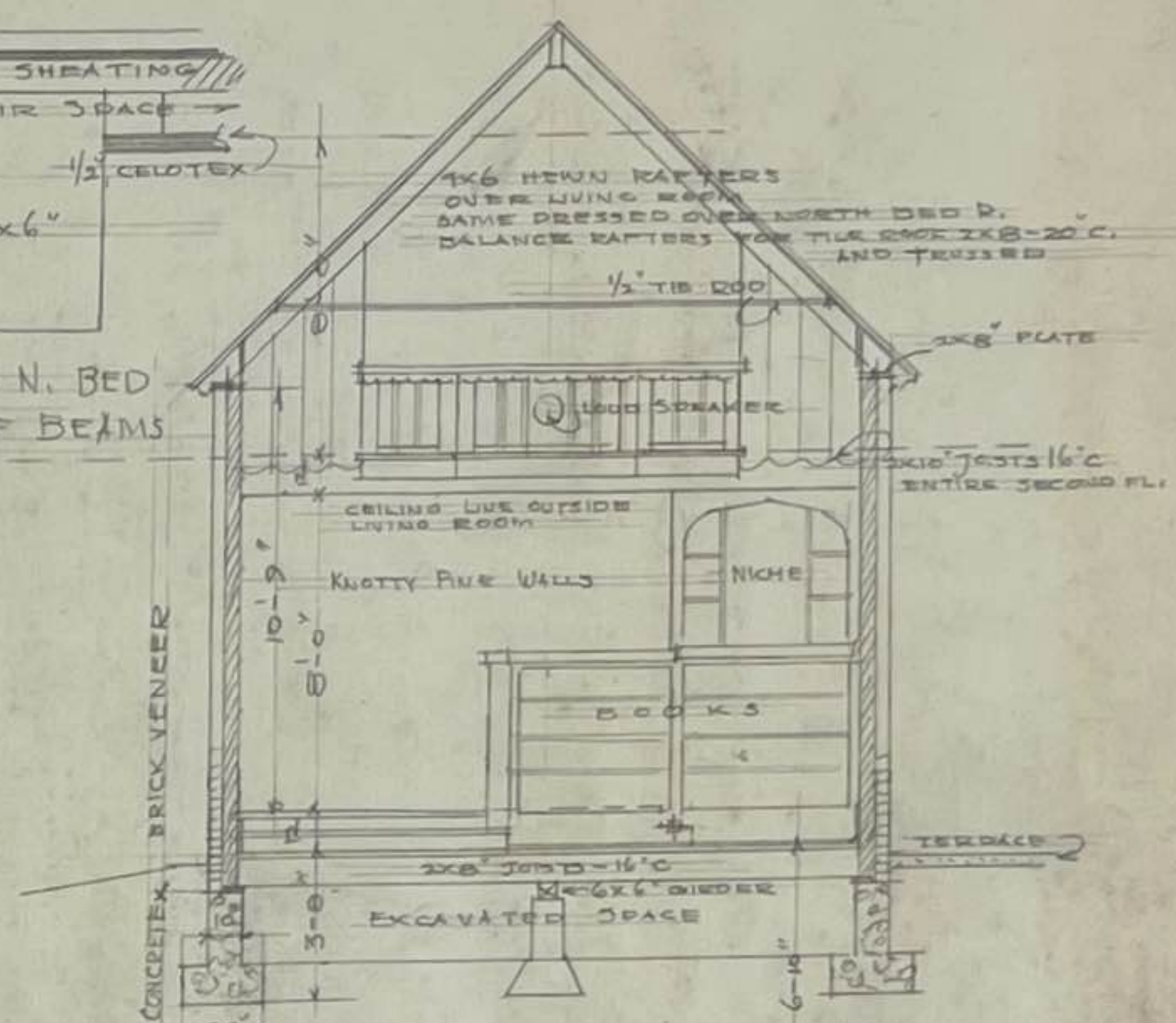
N-S SECTION THRU LIVING R.
