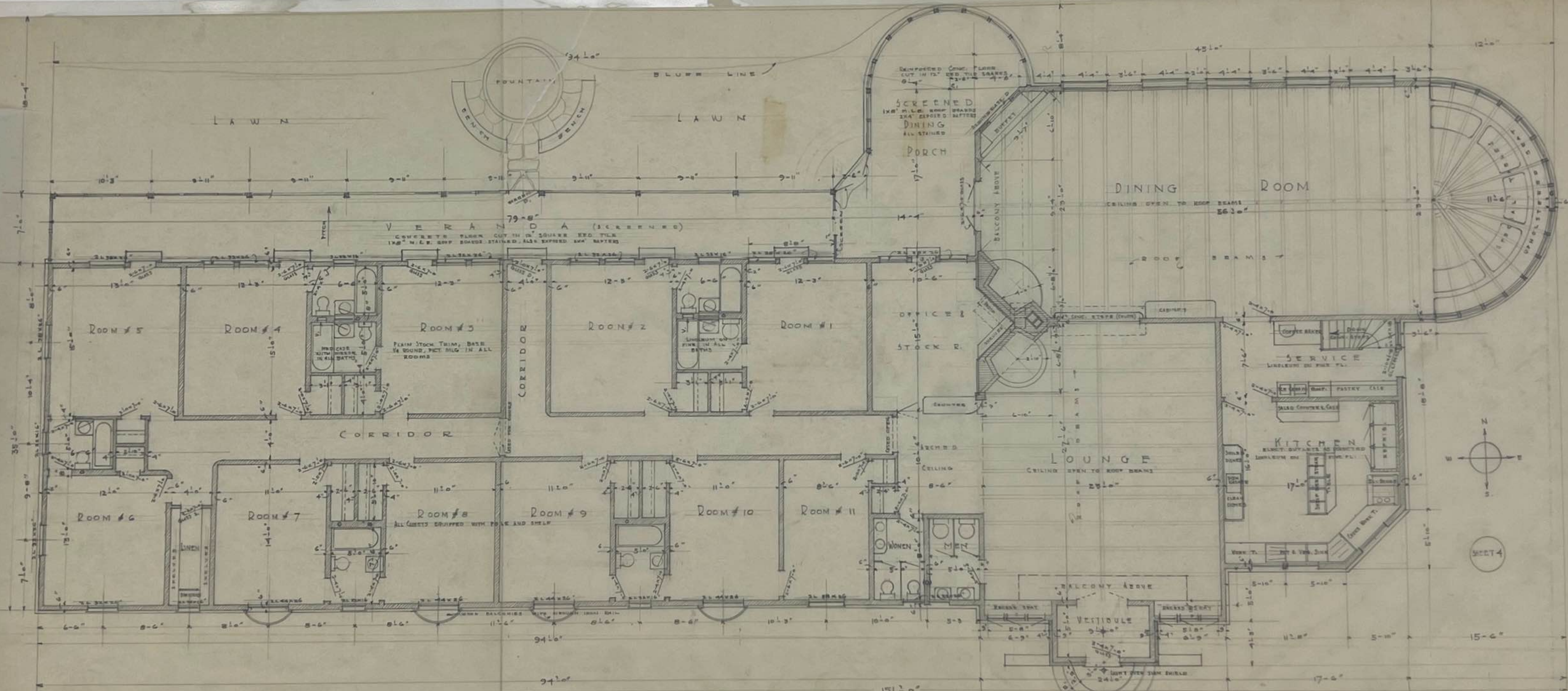
MAIN FLOOR PLAN TYPE OF ALL HARDWOOD FLOORS DETERMINED LATER.
