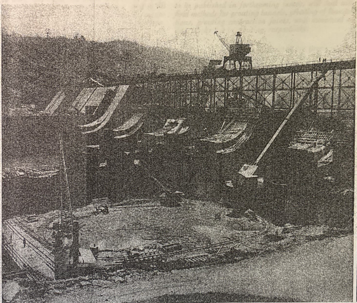
CONSTRUCTING MONOLITHS FOR THE TYGART RIVER DAM, NEAR GRAFTON, W.VA. An Army Engineer Corps Project Designed to Control Floods and Improve Navigation on the Monongahela River
