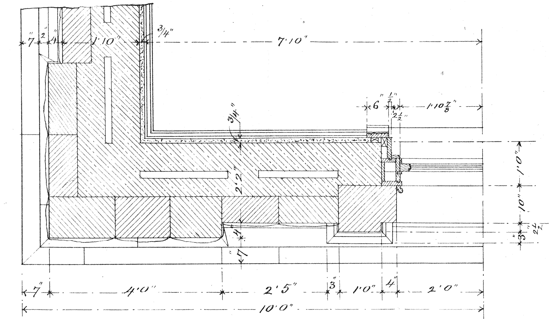
WINDOWS & CORNICE OF TOWER. Scale \frac{3}{4} in = 1 ft. & Full Size.
