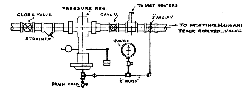
PRESSURE REGULATING VALVE PIPING NOT TO SCALE
