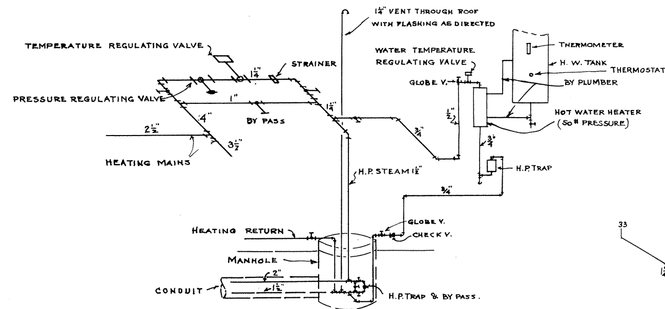
DIAGRAM PIPING CONNECTIONS NEAR MANHOLE NOT TO SCALE
