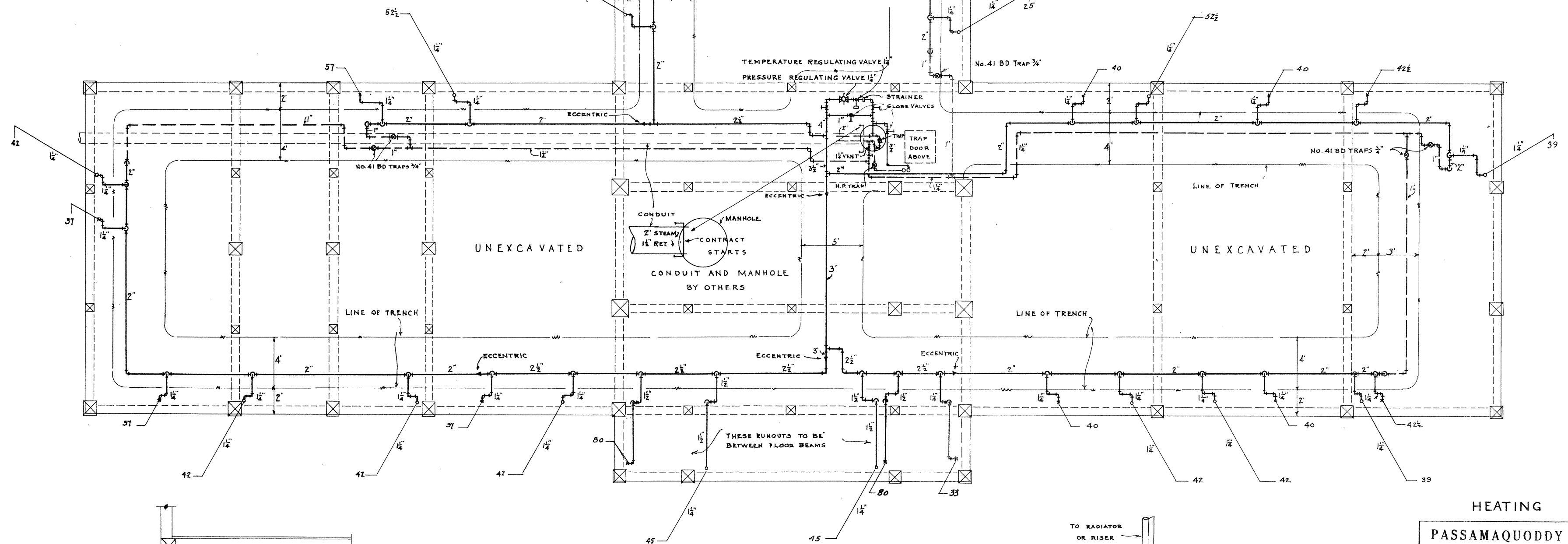
PIPE SPACE BELOW FIRST FLOOR.
