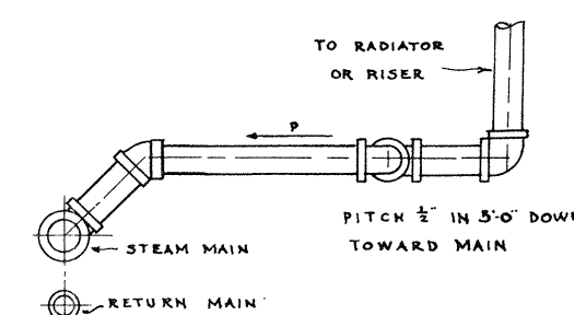
TYPICAL RISER & RADIATOR CONNECTIONS NOT TO SCALE
