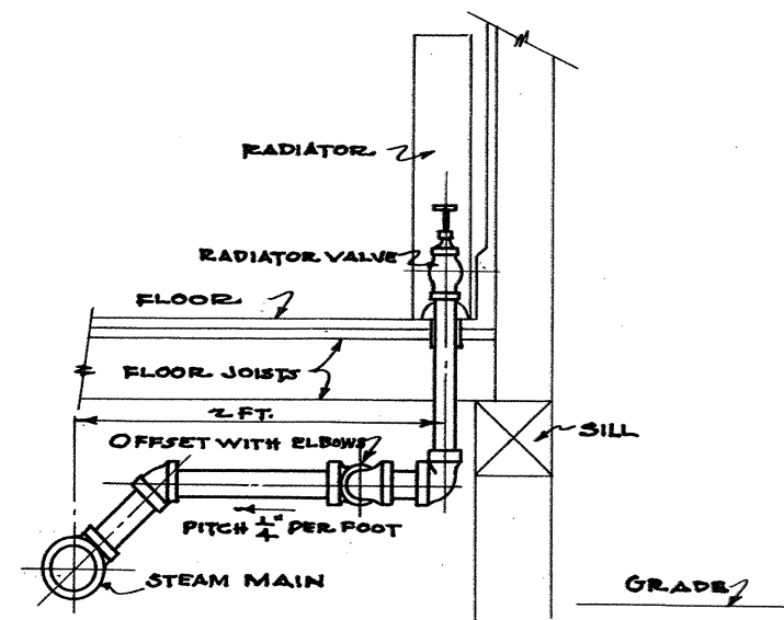
TYPICAL RADIATOR RUNOUT NOT TO SCALE
