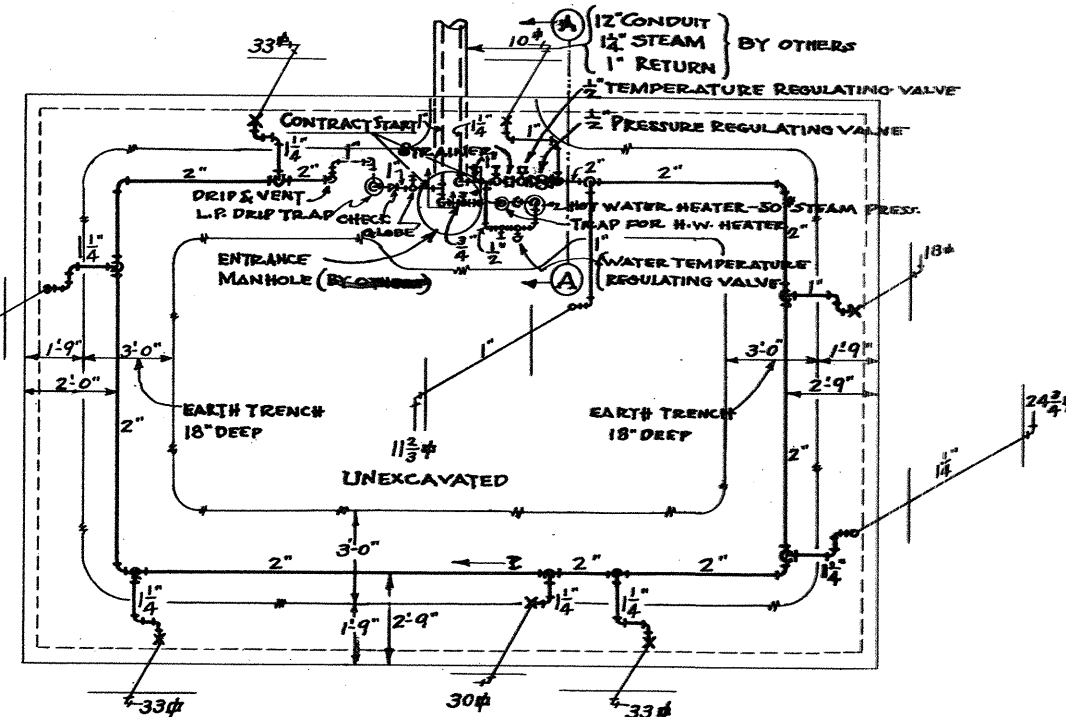
PIPE SPACE BELOW FIRST FLOOR
