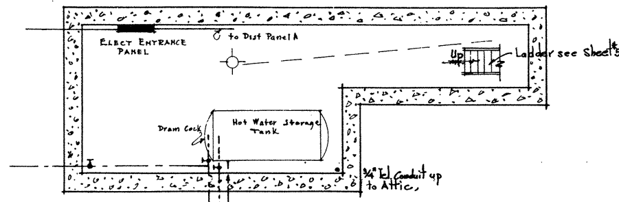
PLAN OF APP. ROOM Scale 1/4" = 1'-0"
