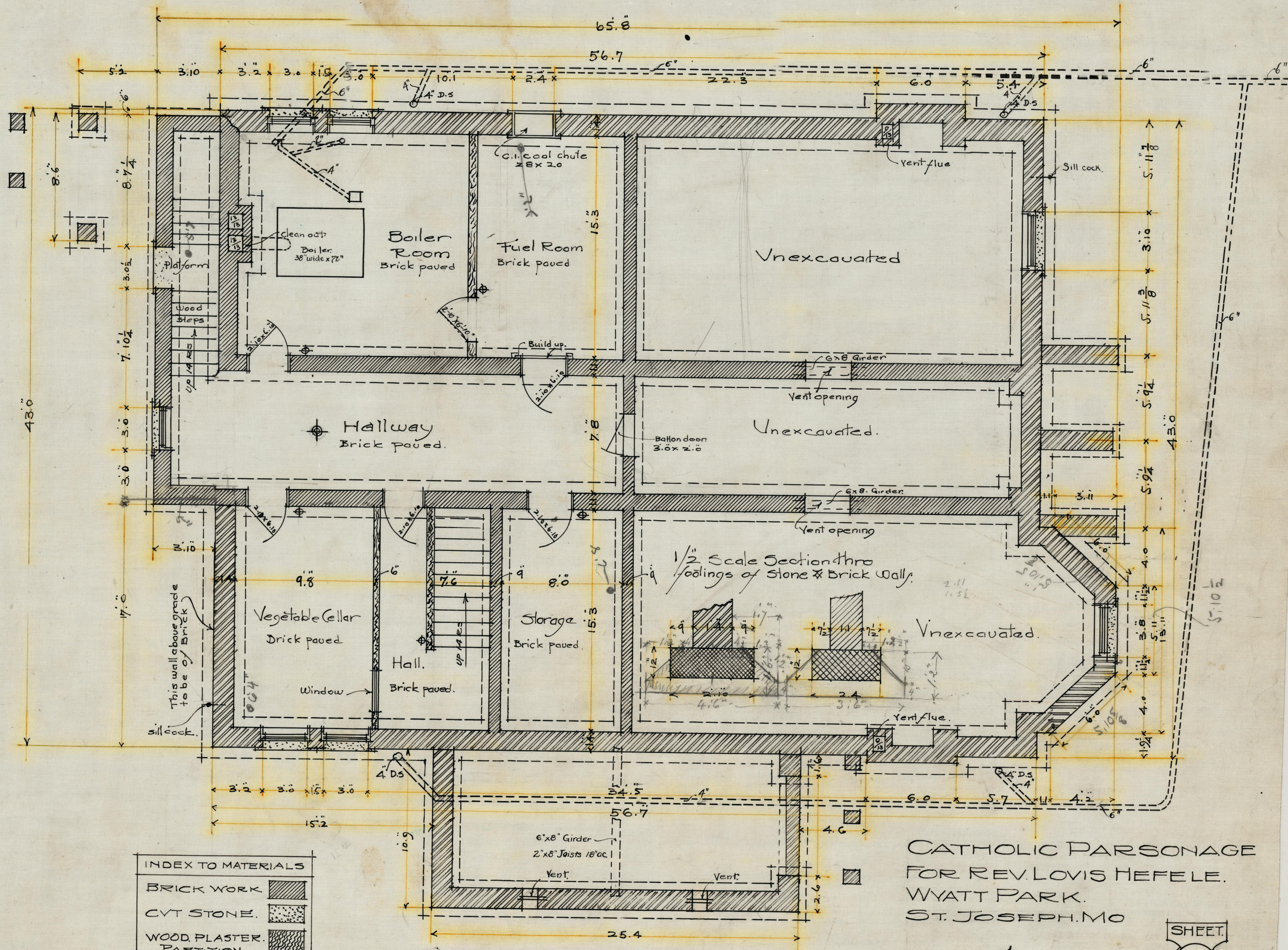
PLAN OF BASEMENT. SCALE \frac{1}{4}'' = 1 FOOT.
