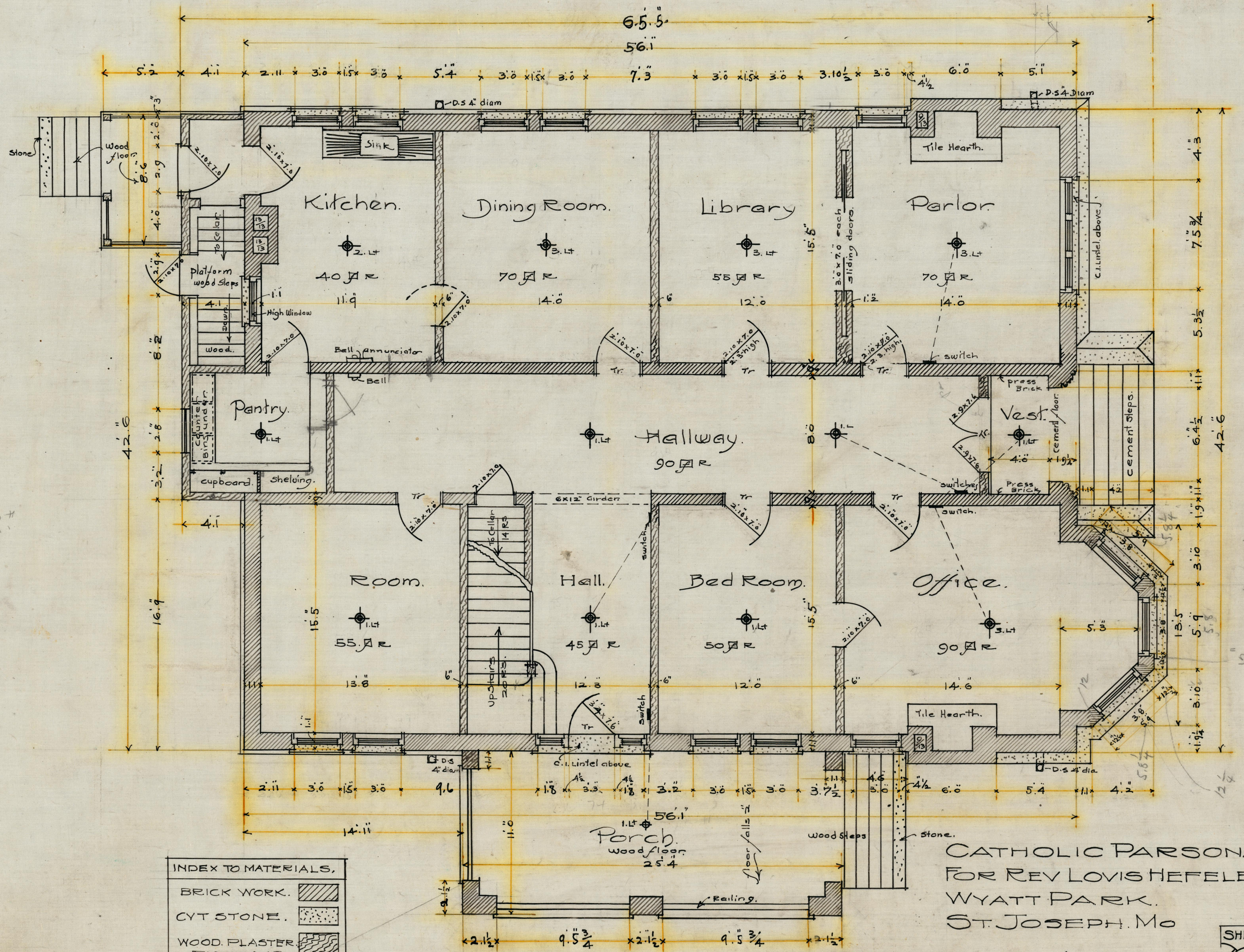
PLAN OF FIRST STORY SCALE \frac{1}{4}" = 1 \text{ FOOT.}
