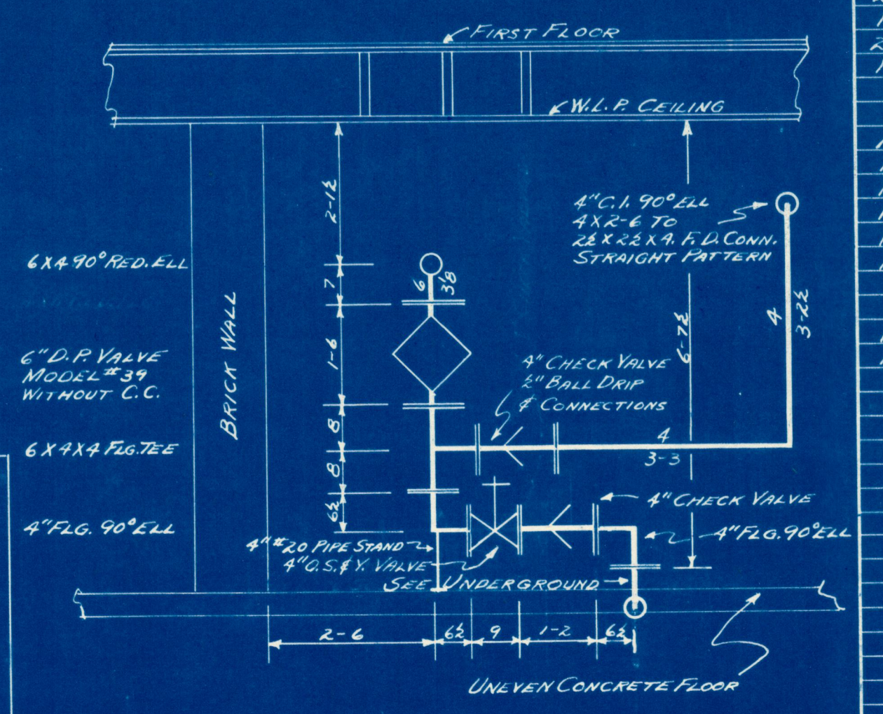
VALVE SECTION LOOKING AT FACE OF VALVE SCALE 2"=1'-0"
