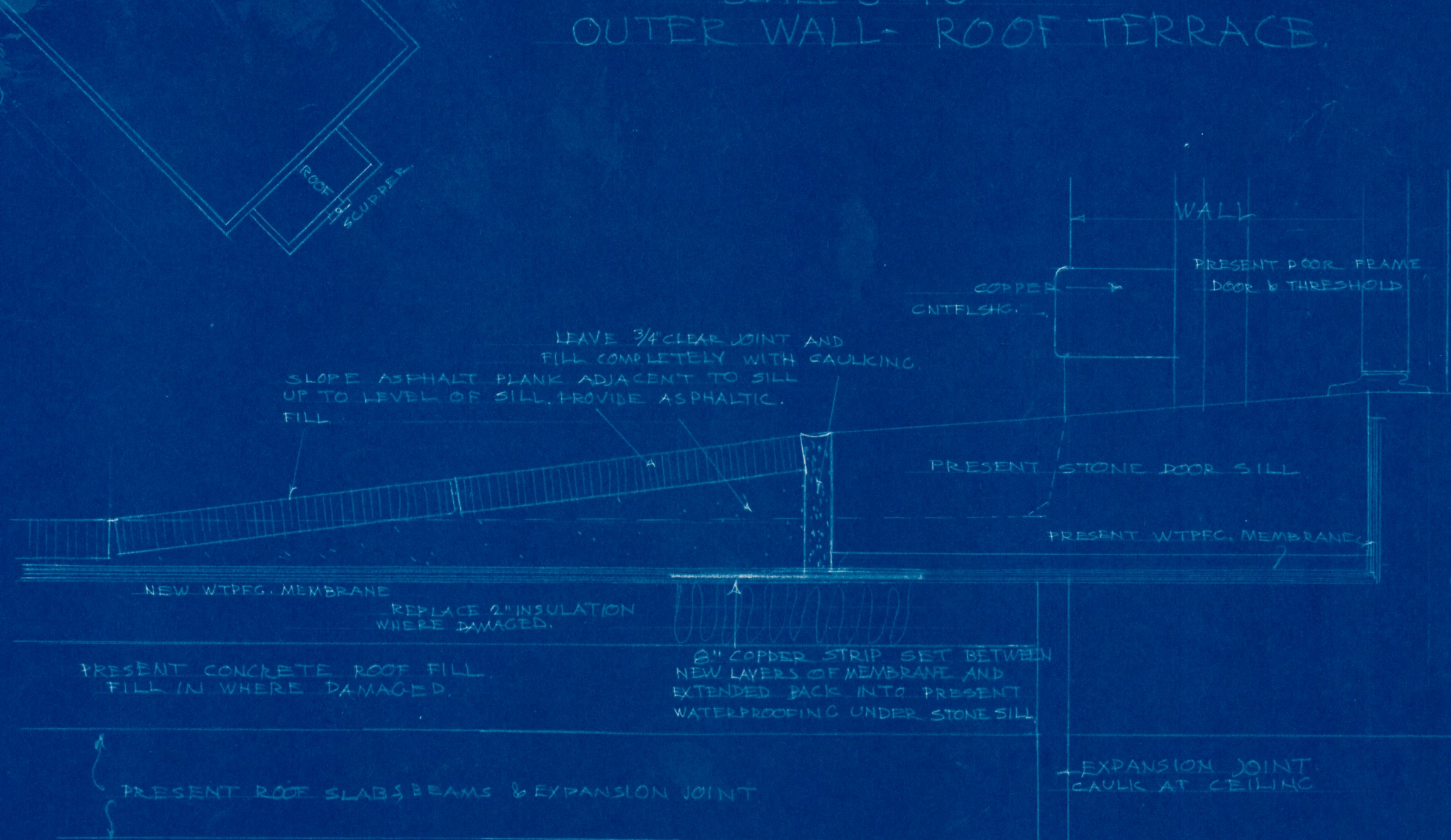
SCALE 3/4"=1'-0" SECTION-DOOR SILL TO ROOF TERRACE
