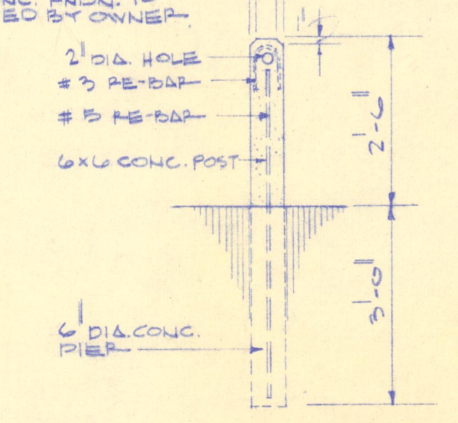
TYPICAL POST DETAIL SCALE: 1/2" = 1'-0"
