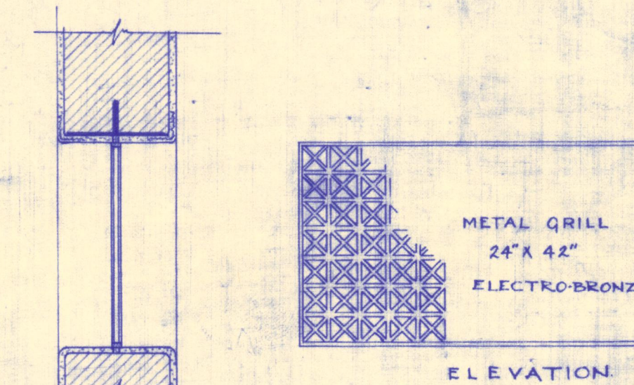
SECT. 3/4\"/>
