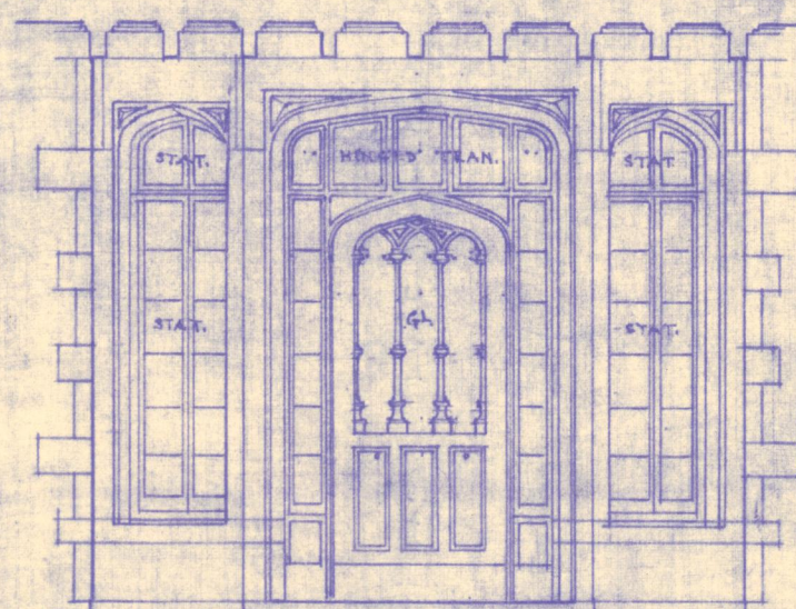
OUTSIDE ELEVATION OF MAIN ENTRANCE - SOUTH SIDE
