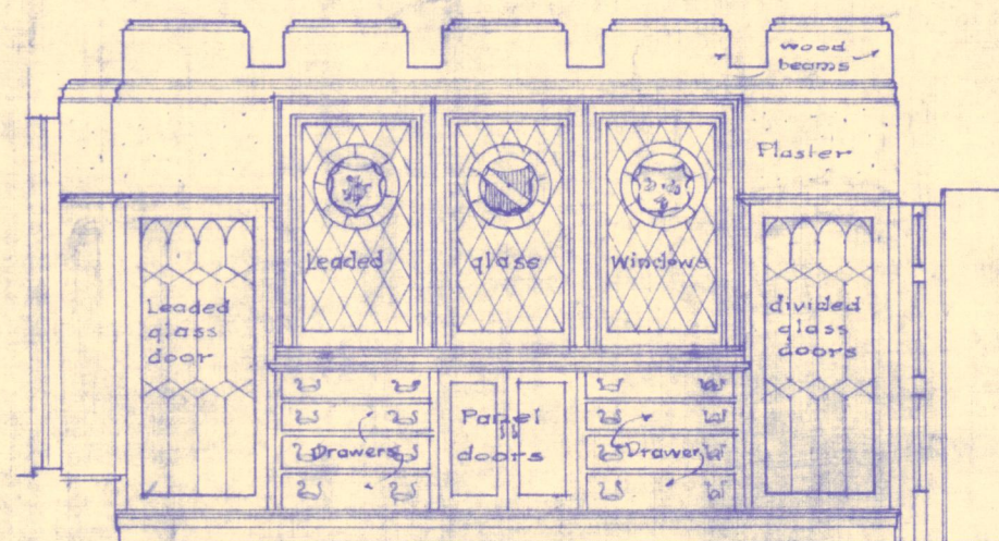
NORTH ELEVATION DINING ROOM SHOWING SIDESBOARD AND CASES
