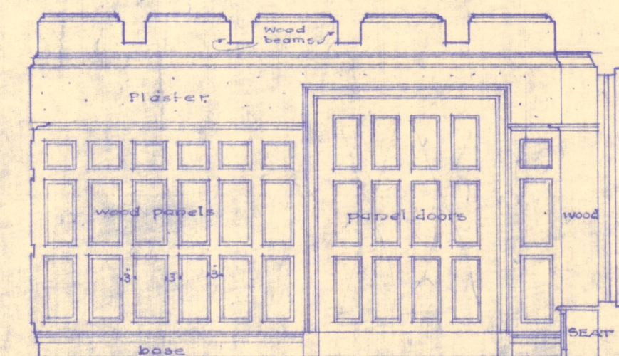
ELEVATION SOUTH END DINING ROOM
