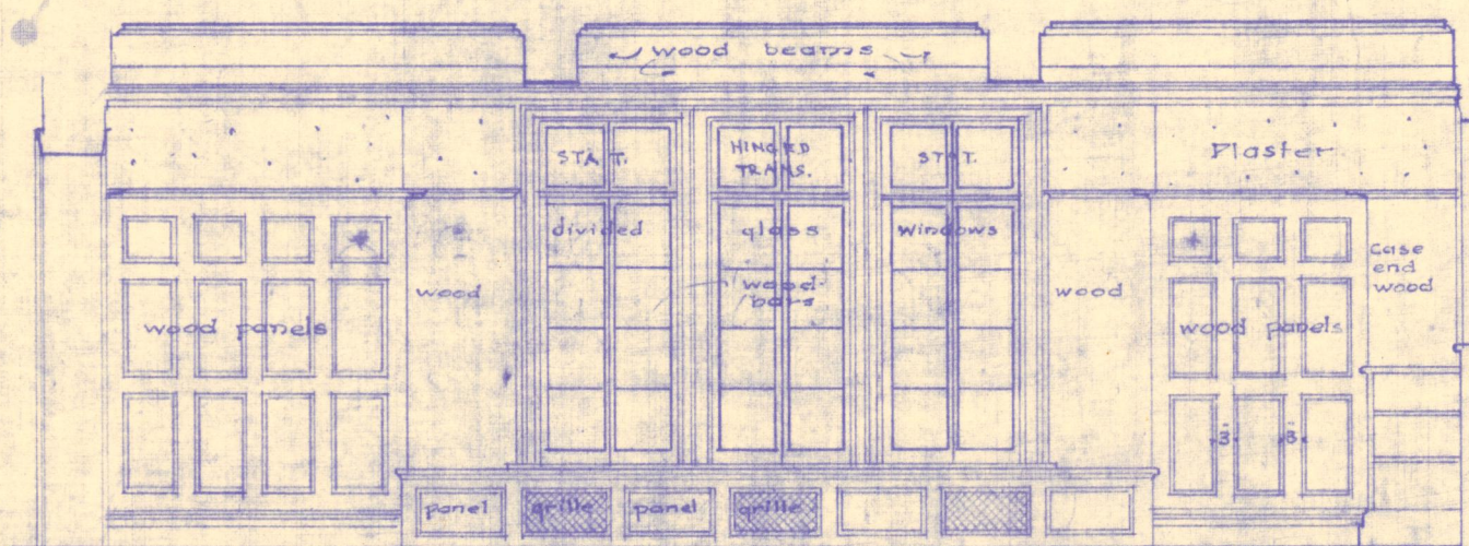
ELEVATION WEST SIDE DINING ROOM
