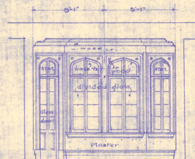
ELEVATION DAY WINDOW IN SITTING RM. END FLOOR
