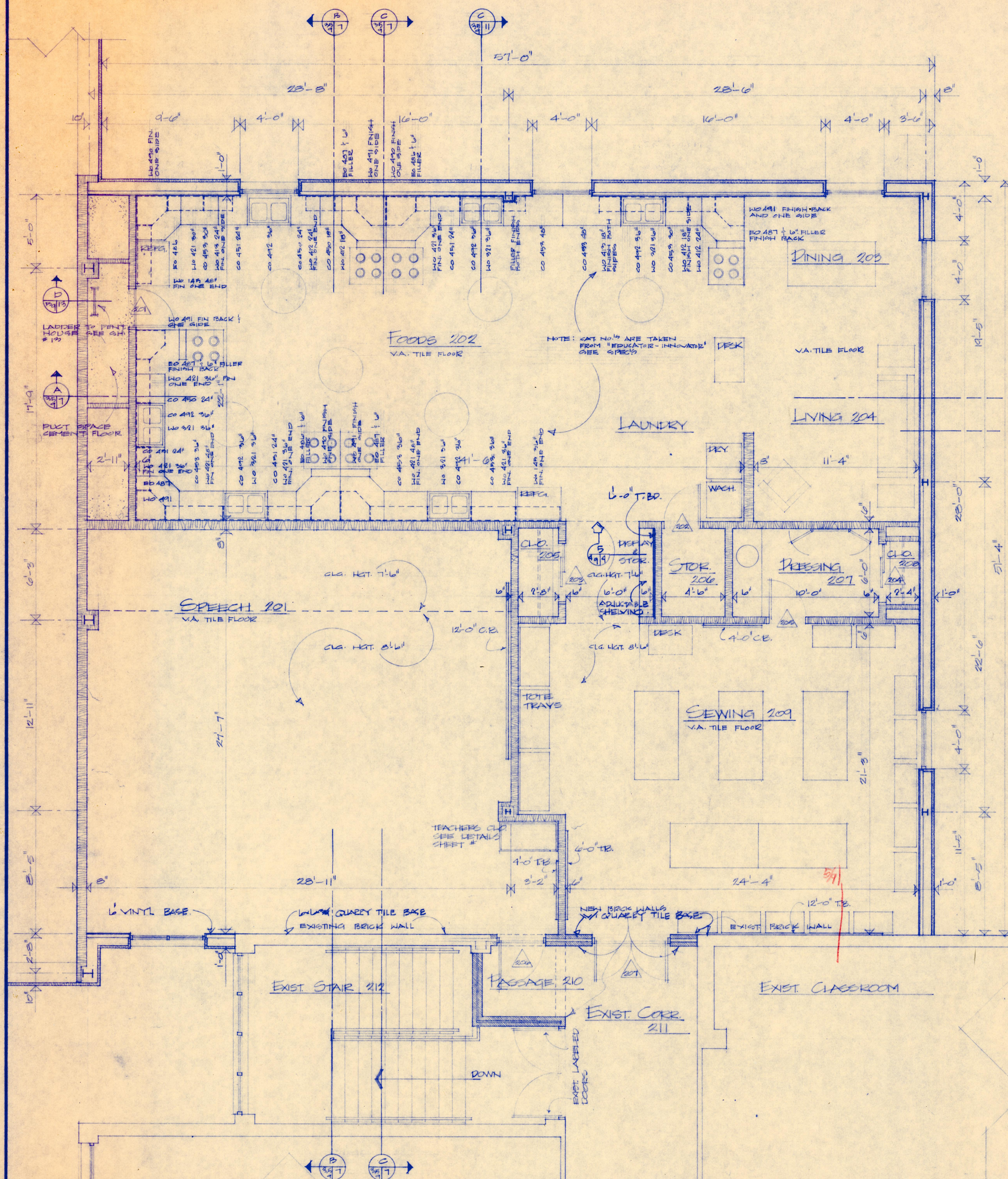
PARTIAL PLAN - SECOND FLOOR SCALE: 1/4" = 1'-0"
