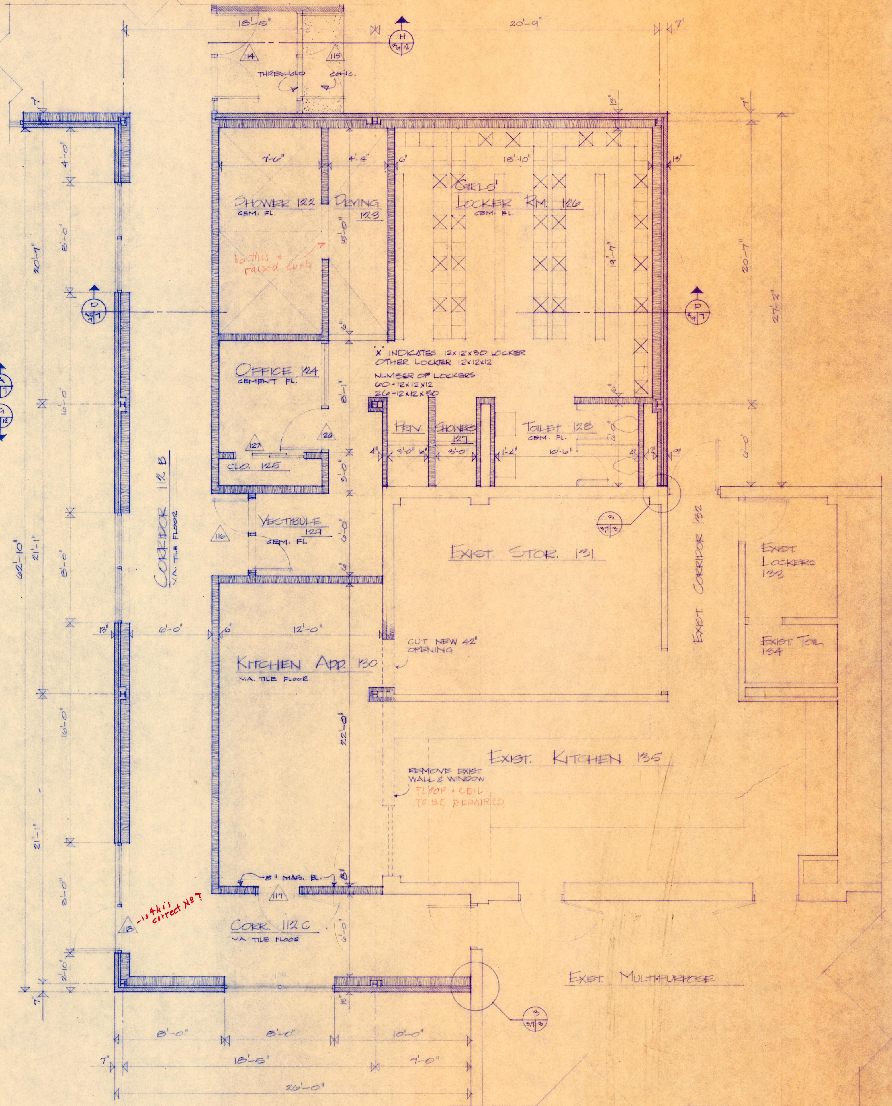
PARTIAL PLAN - FIRST FLOOR SCALE: 1/4" = 1'-0"
