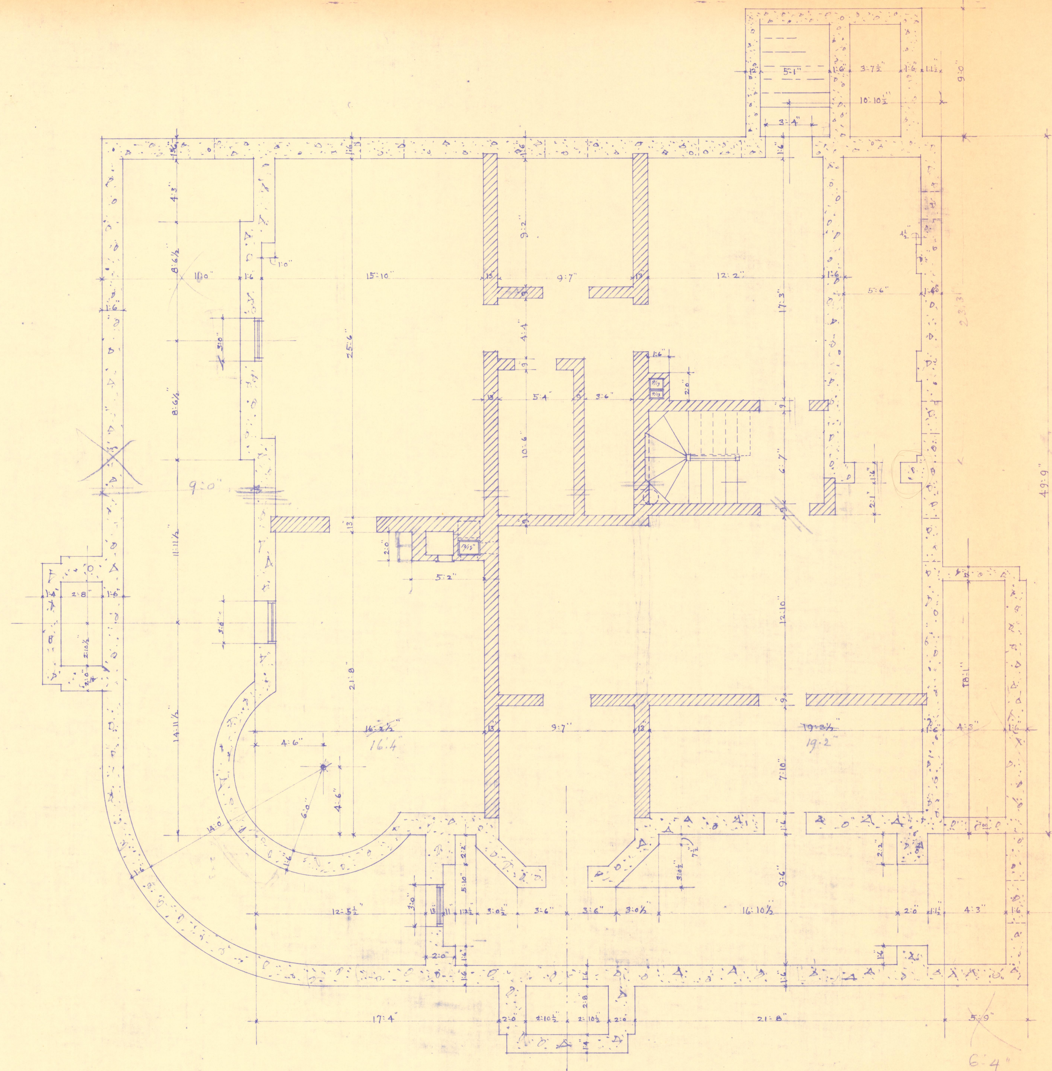
PLAN SHOWING CONCRETE WALLS SCALE \frac{1}{4}'' = 1'-0''
