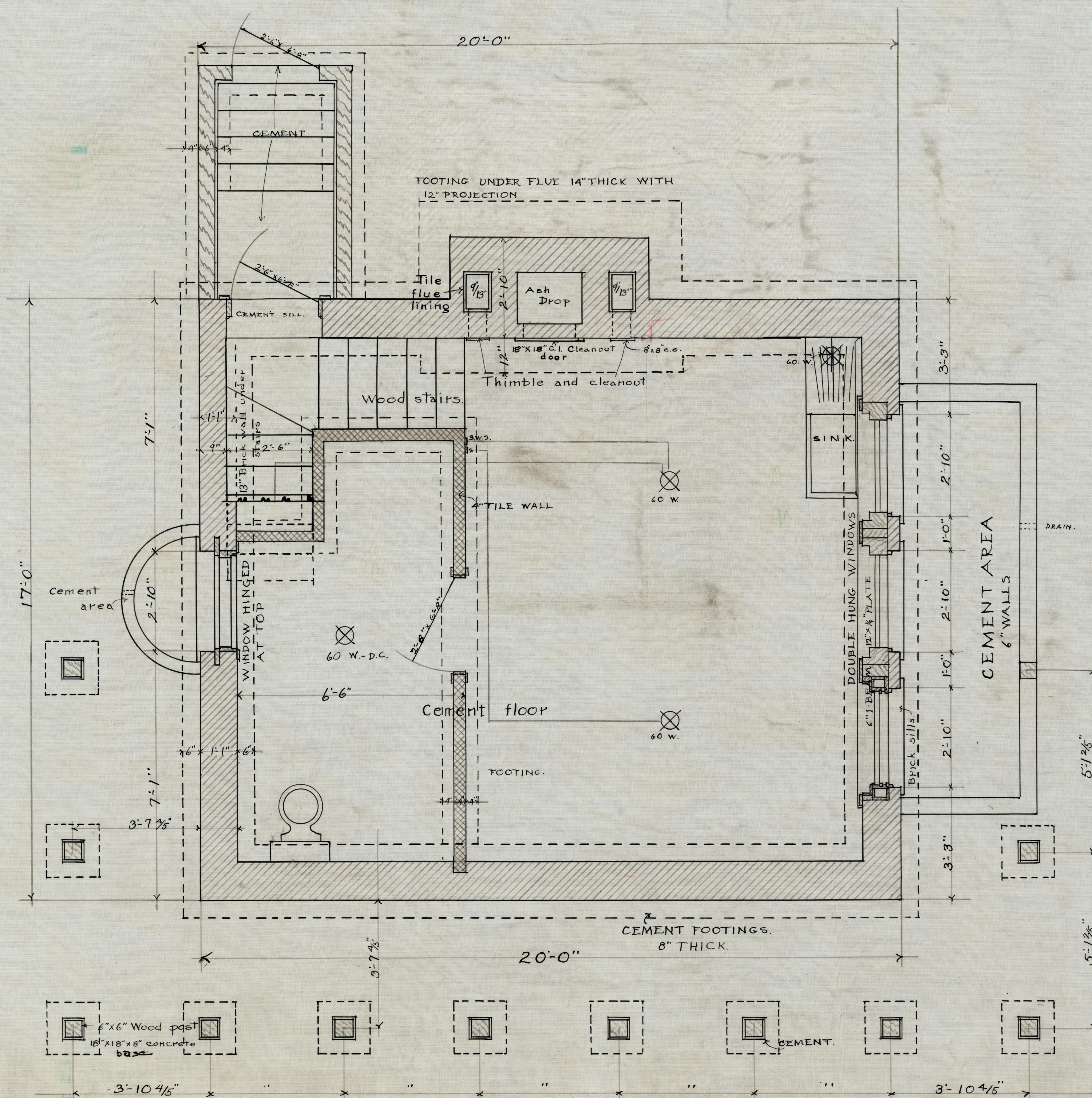
SCALE \frac{1}{2}'' = 1'-0 BASEMENT PLAN
