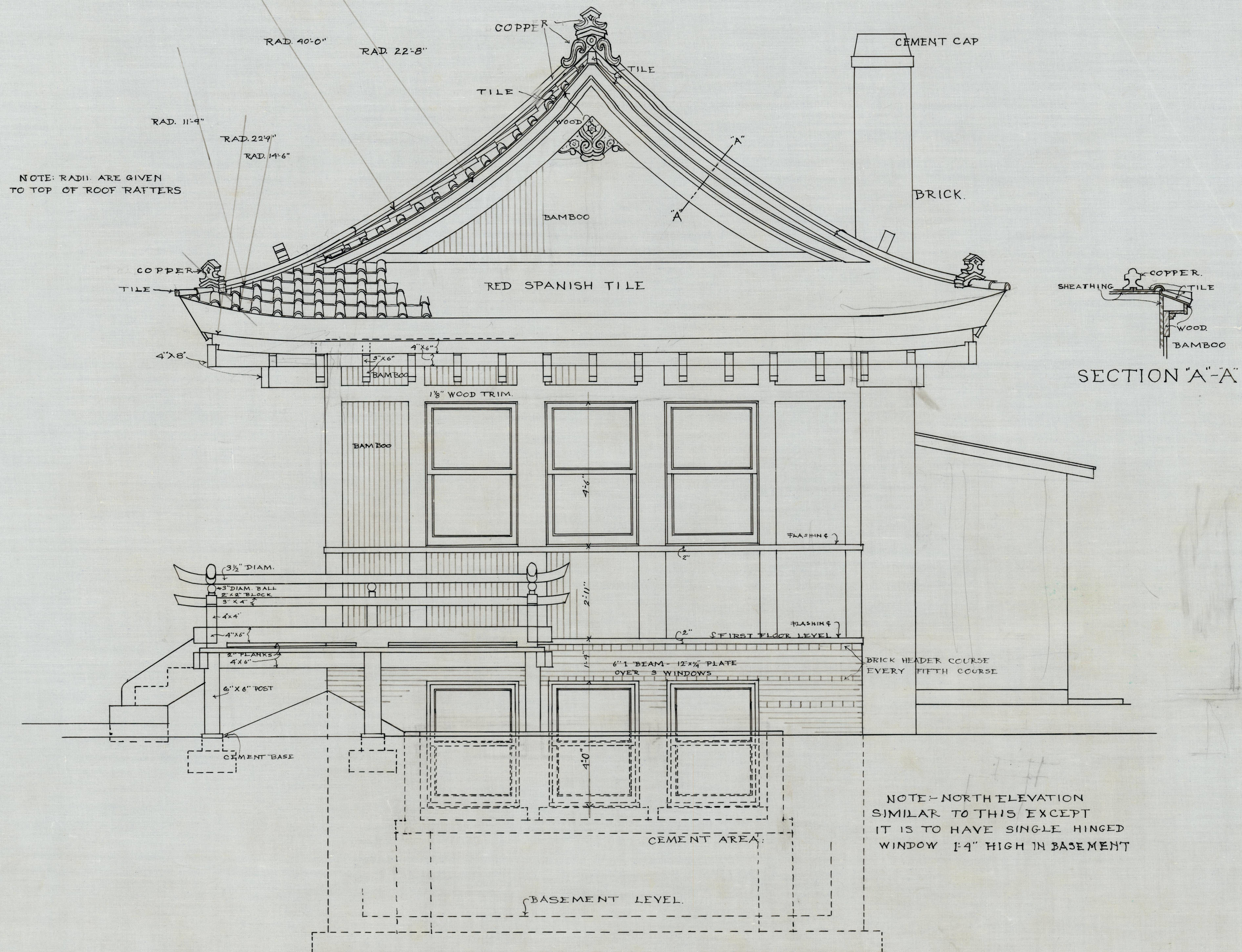
SOUTH ELEVATION
