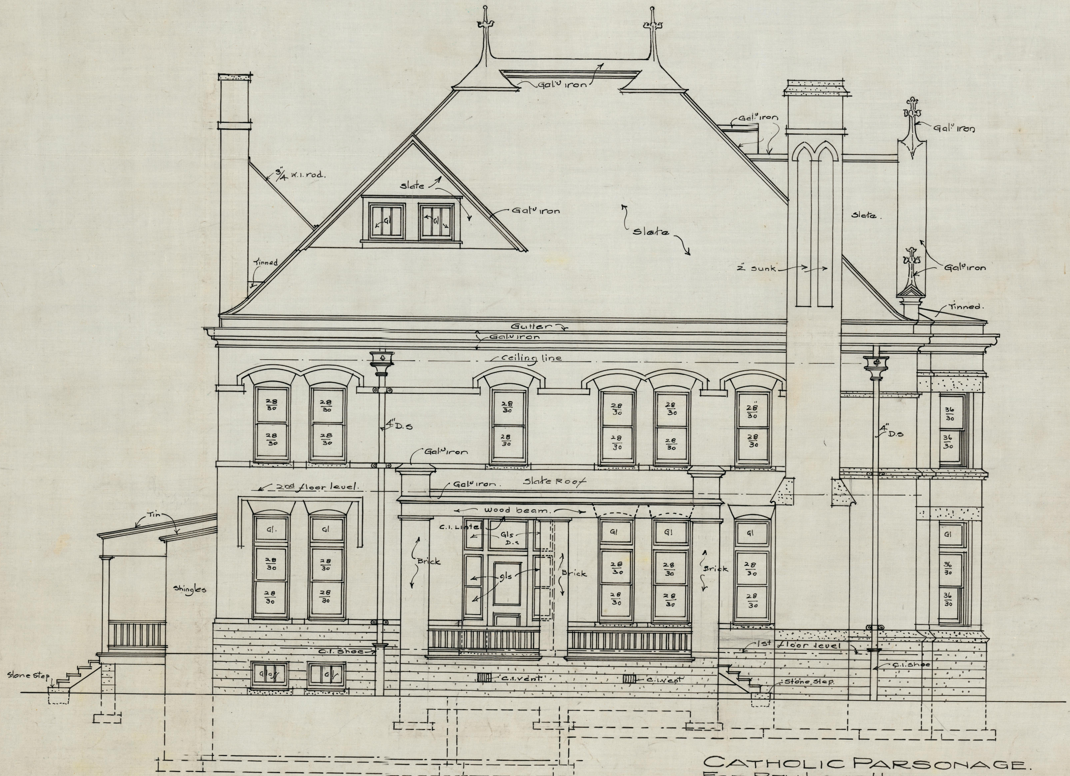
• SIDE ELEVATION. • SCALE 1/4" = 1. FOOT.
