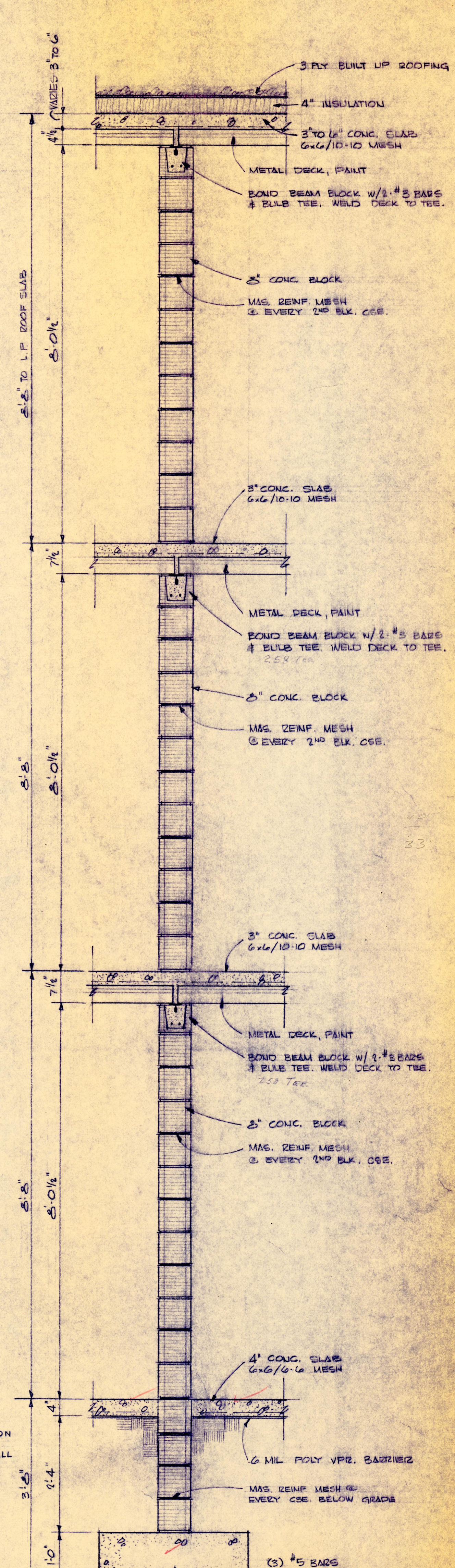
SECTION (E) SCALE \frac{3}{4}" = 1'-0" SECTION (F) SIM. EXCEPT BLOCK WALLS 6" TH.
