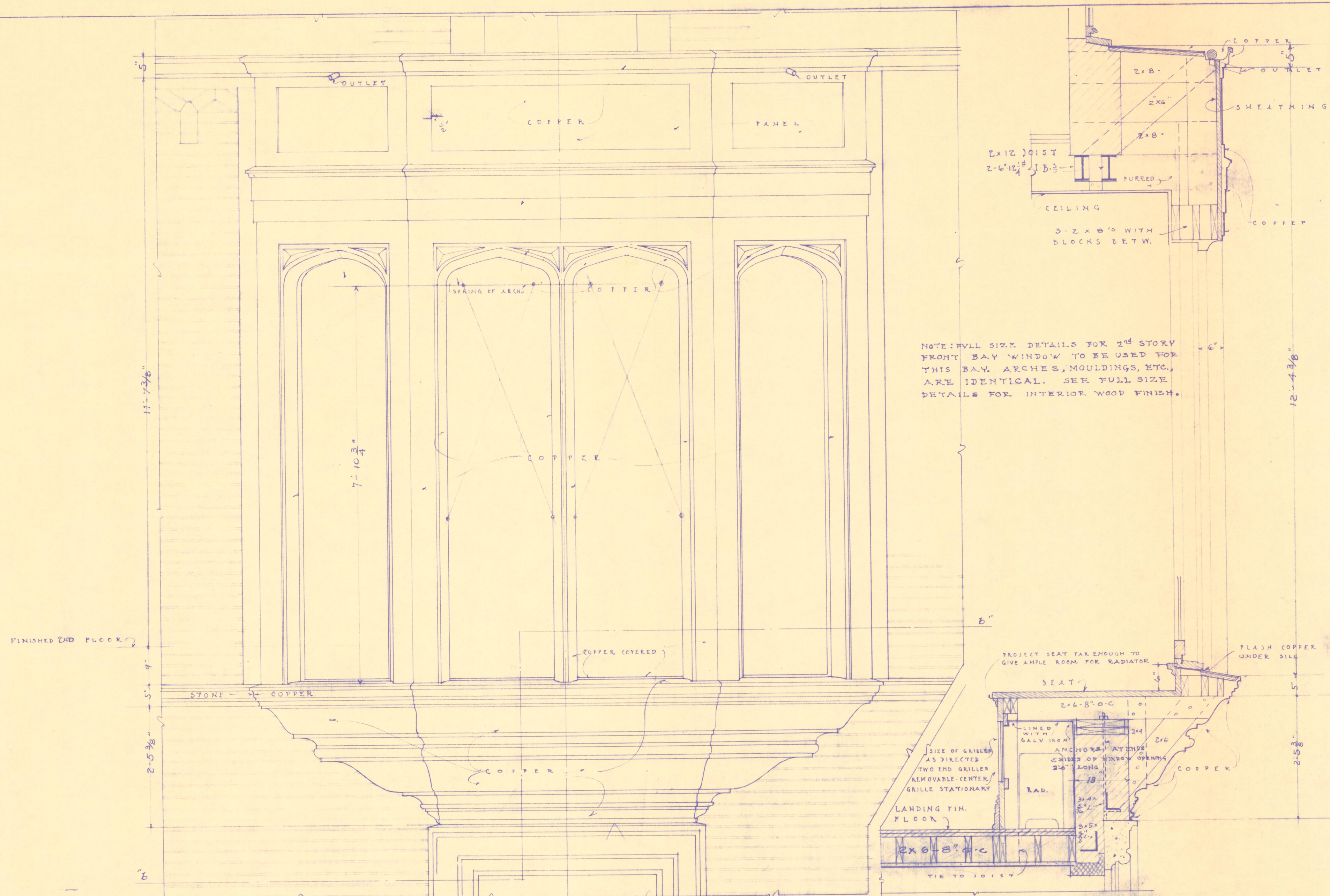
EXTERIOR ELEVATION OF 2ND STORY BAY NORTH SIDE
