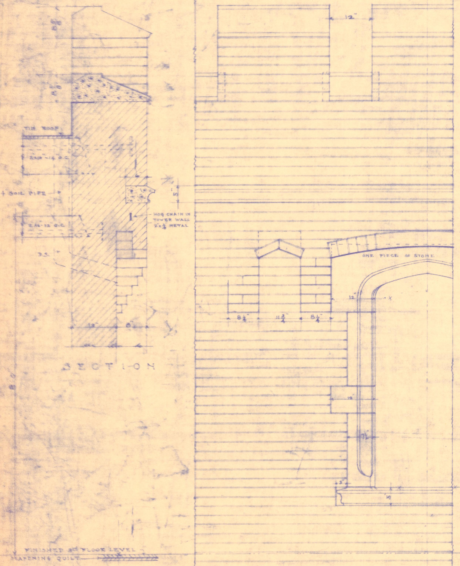
DETAILS OF TOWER CRENNELLATIONS AND UPPER WINDOWS ETC.
