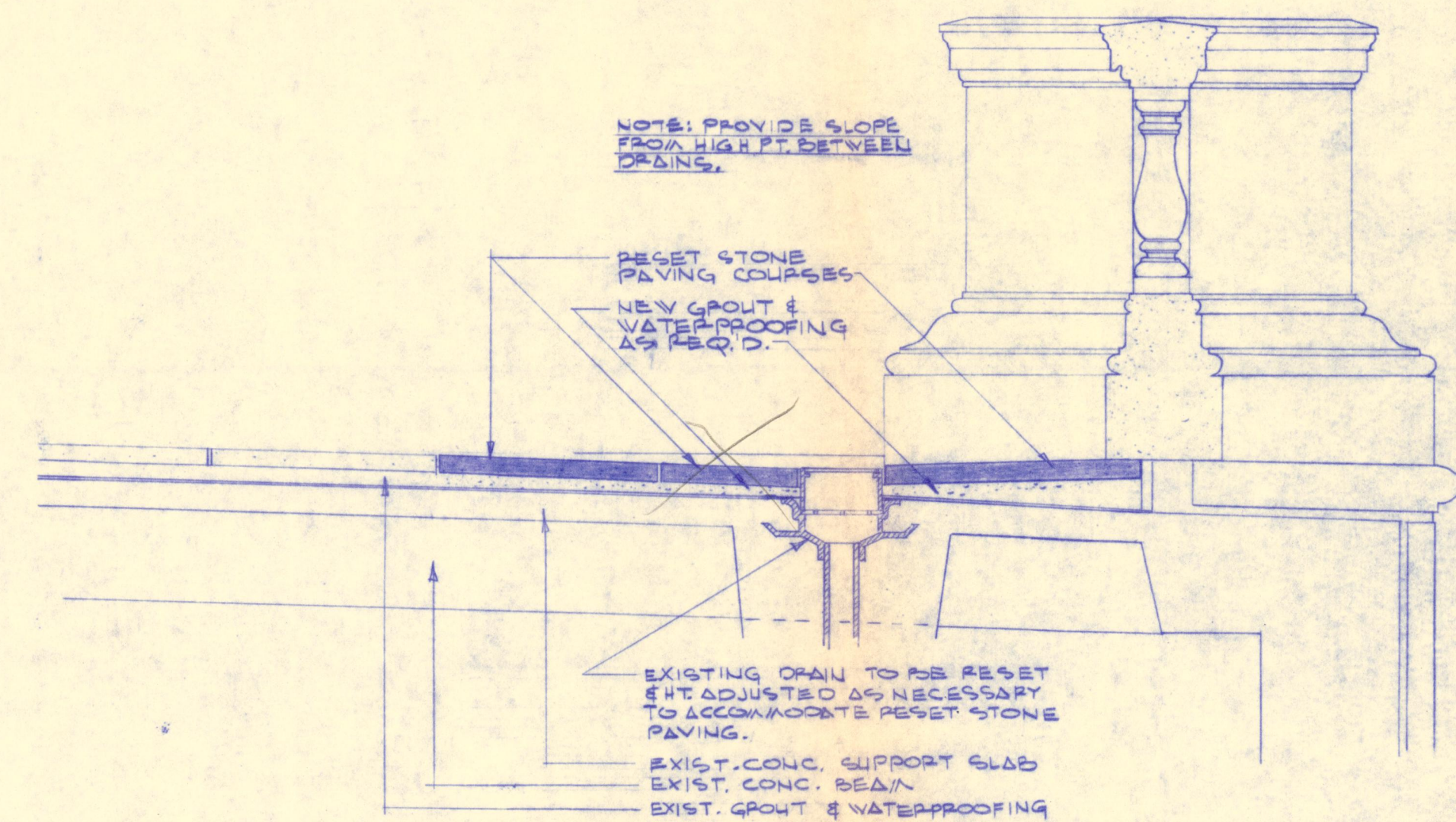
STONE PAVING RESETTING DETAIL - ALT. BID#2 SCALE: 3/4" = 1'-0"
