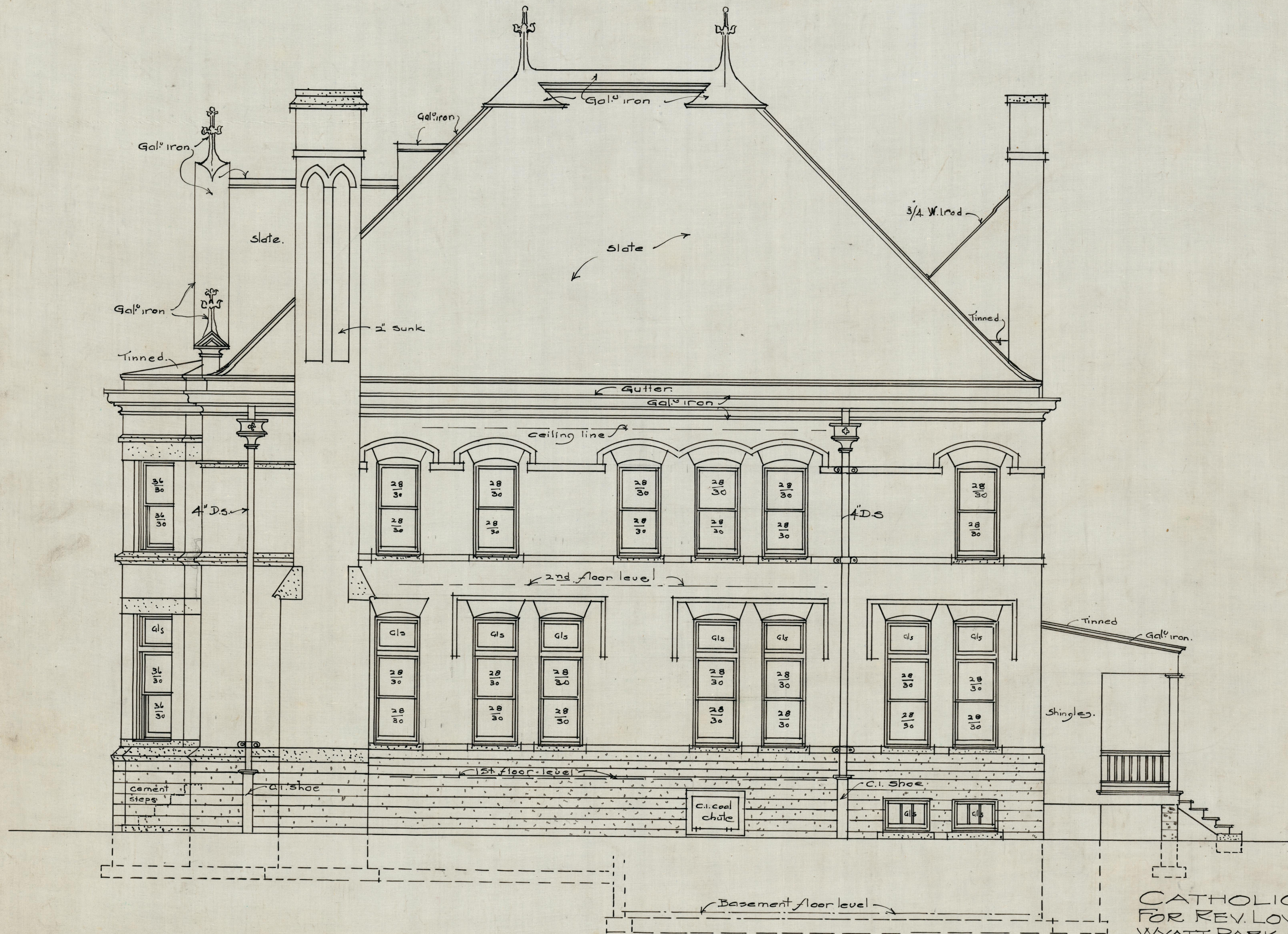
· SIDE ELEVATION. · SCALE \frac{1}{4} " = 1. FOOT.
