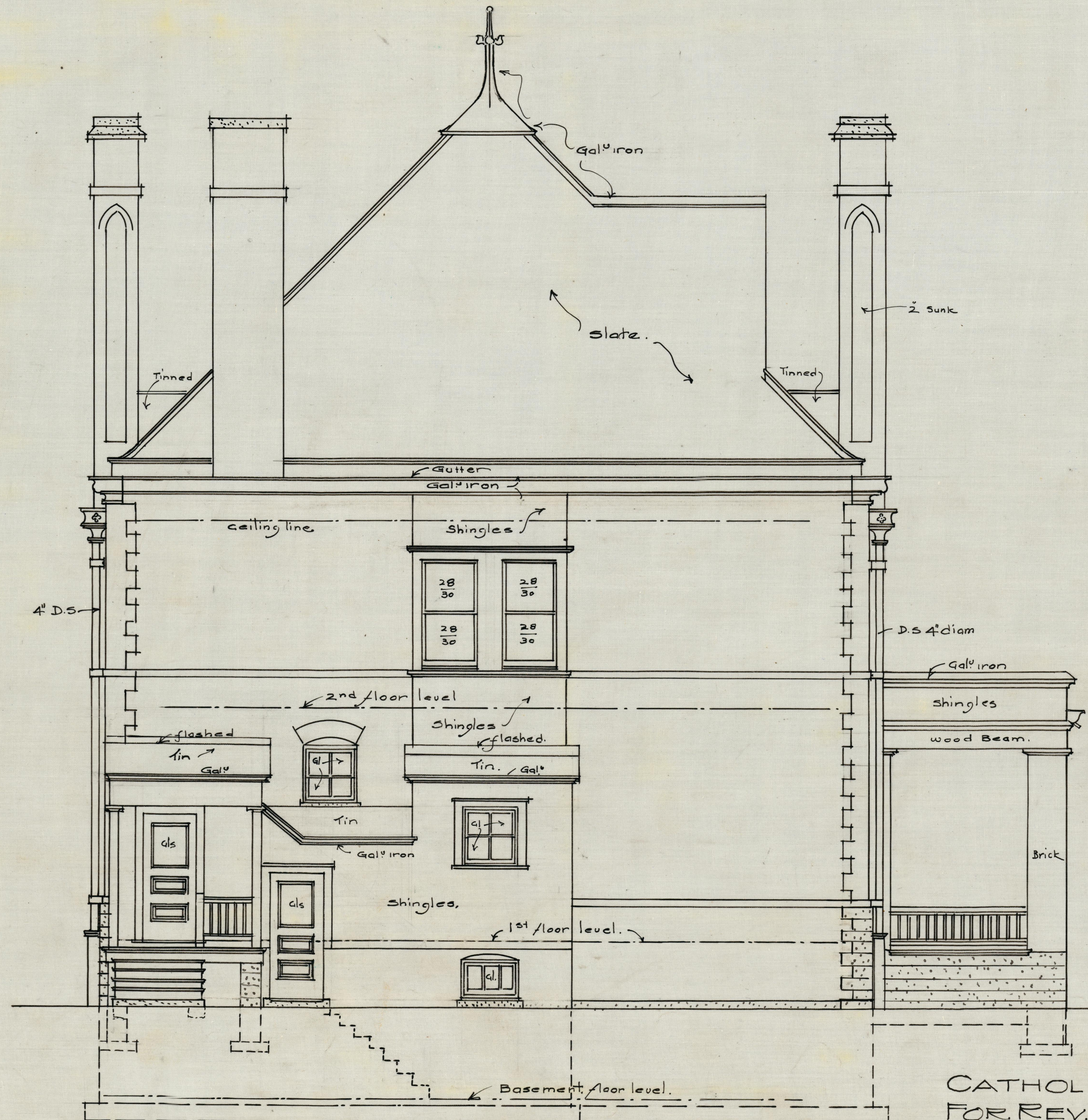
• REAR ELEVATION. • SCALE \frac{1}{4} " = 1' FOOT.
