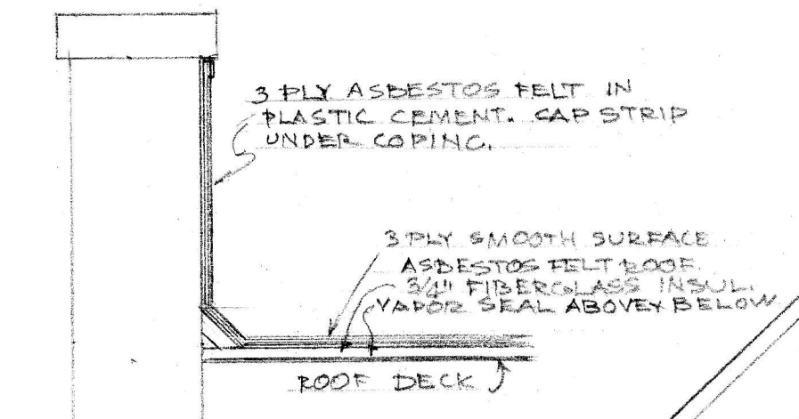
DETAIL - PARAPET WATERPROOFING. SCALE 3/4"=1'-0"
