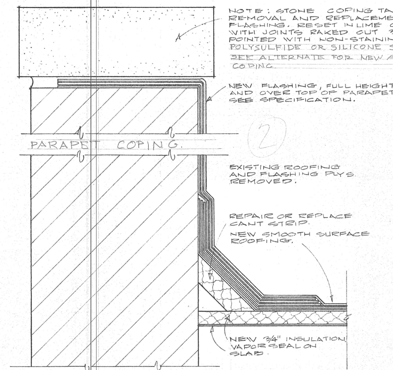
PARAPET WALL FLASHING DETAIL "A"
