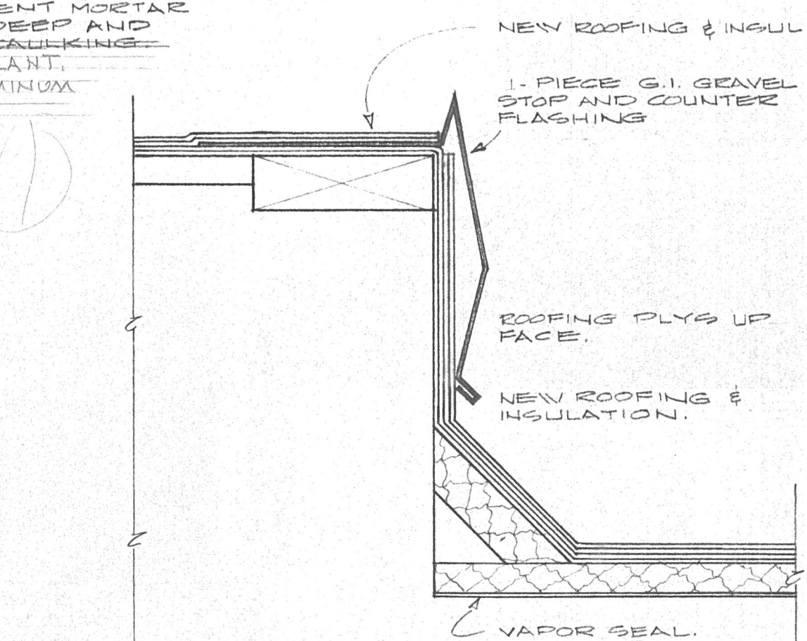
RAISED ROOF FLASHING DETAIL "C"
