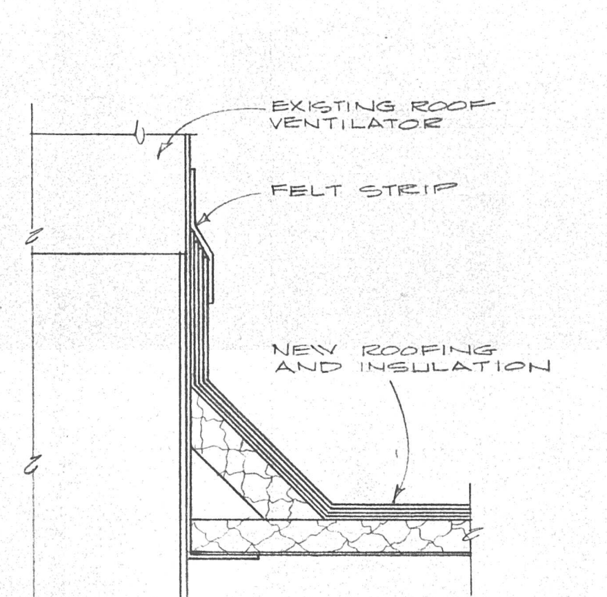
VENTILATOR FLASHING DETAIL "D"
