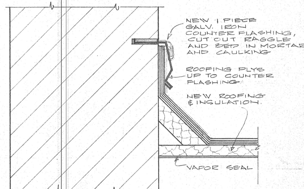
ROOF AND WALL FLASHING DETAIL "B"
