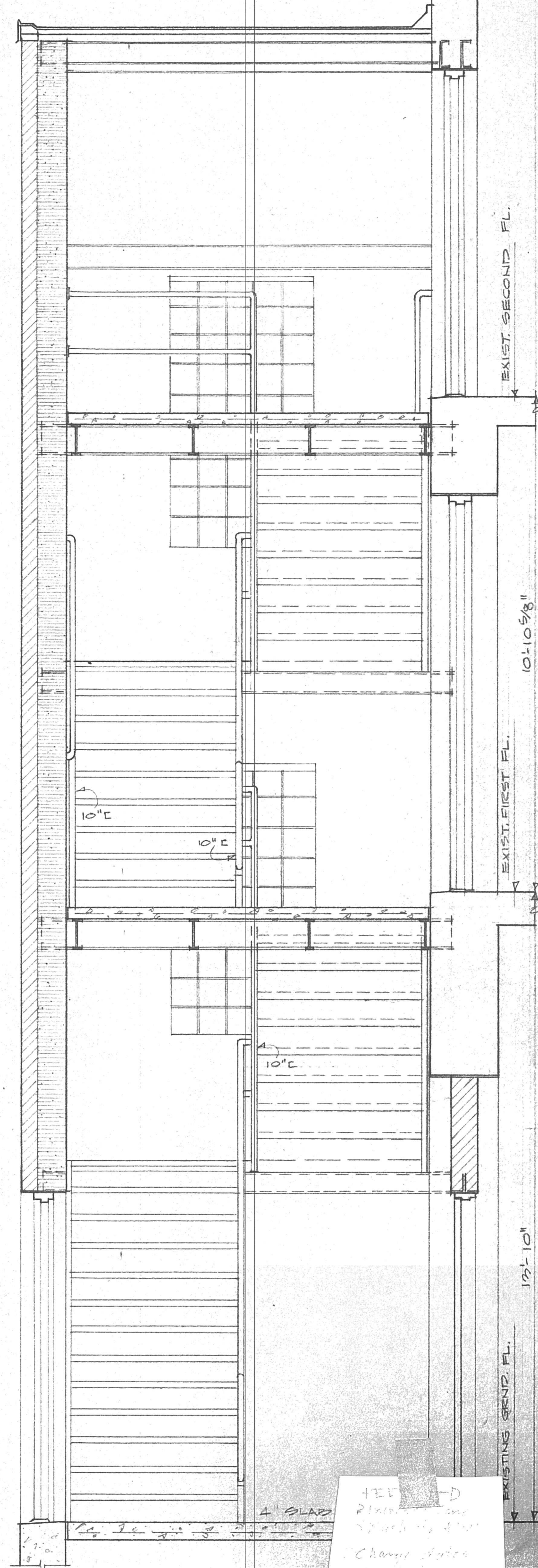
SECTION SCALE 1/2" = 1'-0"
