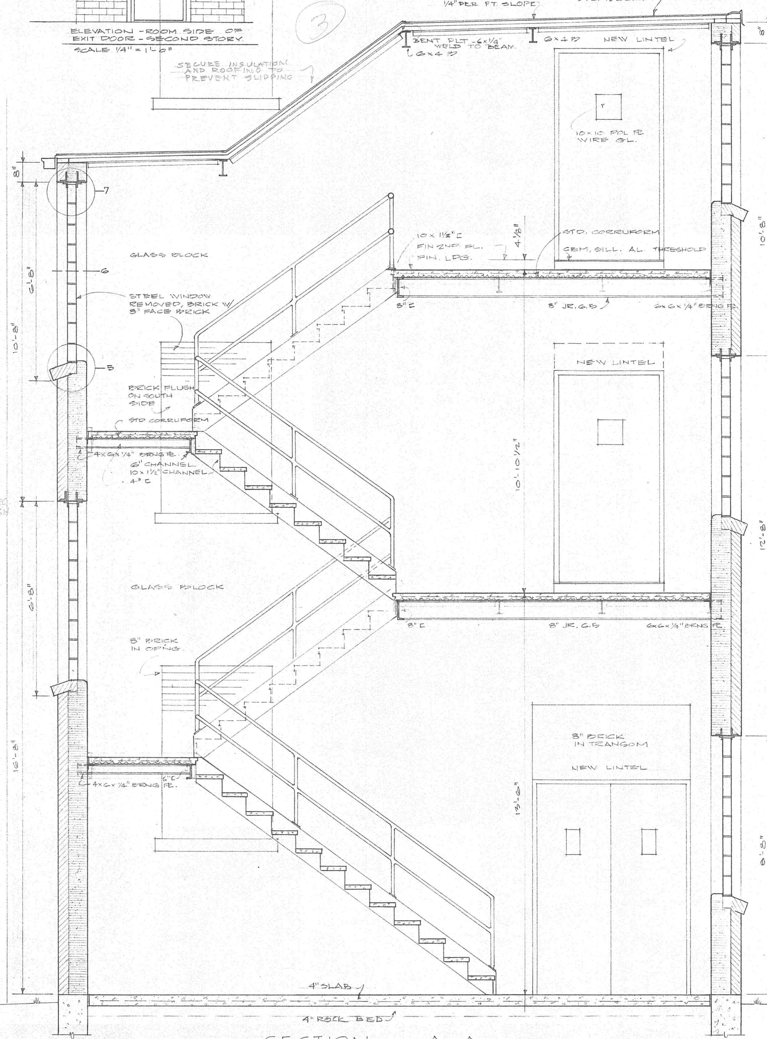
SECTION A-A SCALE 1/2" = 1'-0"
