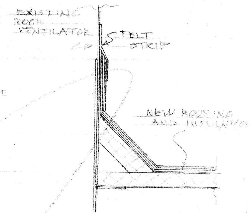
VENTILATOR FLASHING DETAIL "D"
