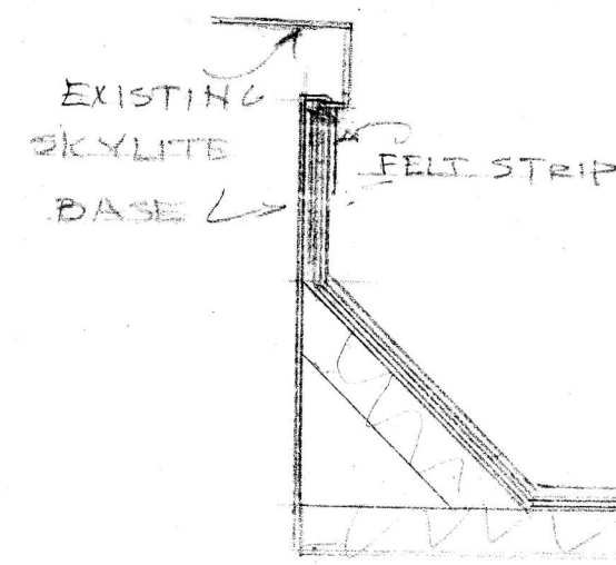
SKYLIGHT FLASHING DETAIL "E"
