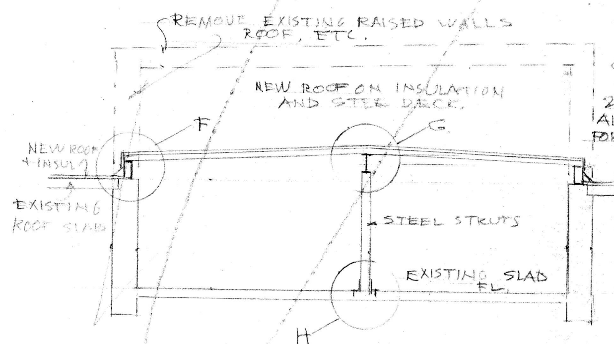
SECTION - LOWERED THIRD STORY SCALE 1/4" = 1'-0"
