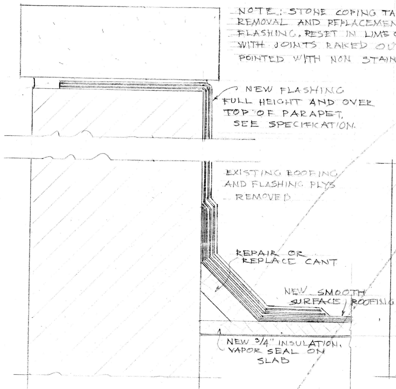
PARAPET WALL FLASHING DETAIL "A"
