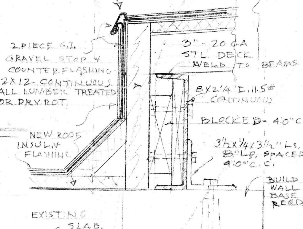
UPPER CENTER DETAIL G
