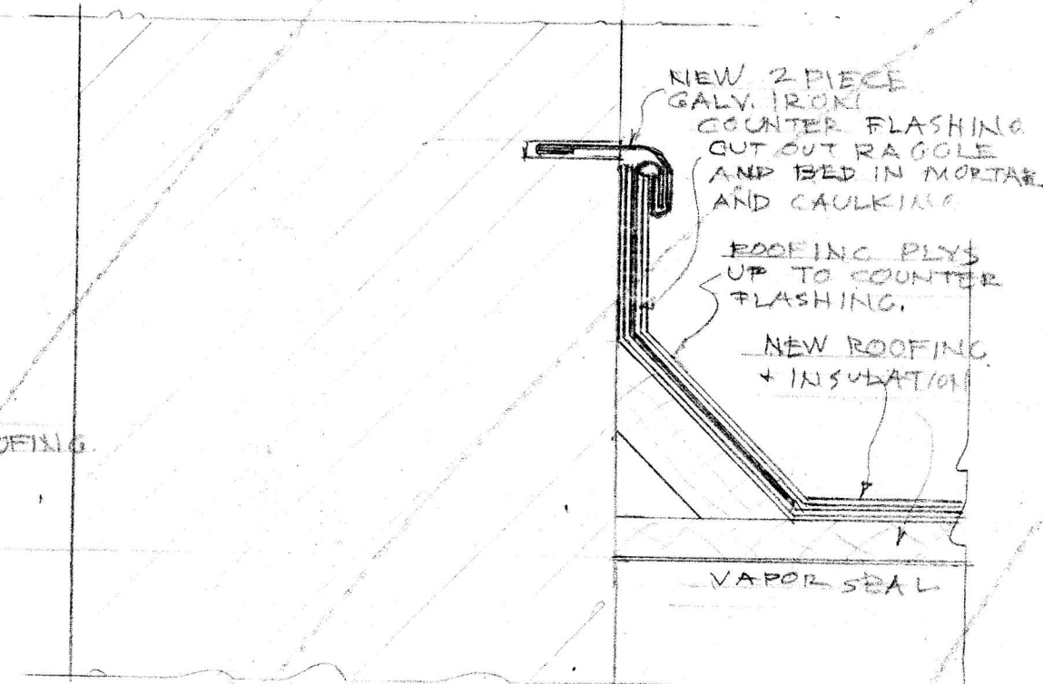
ROOF AND WALL FLASHING DETAIL "B"
