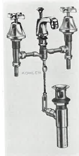
Bancroft K-8010-A With Aerator and Pop-up Drain.
