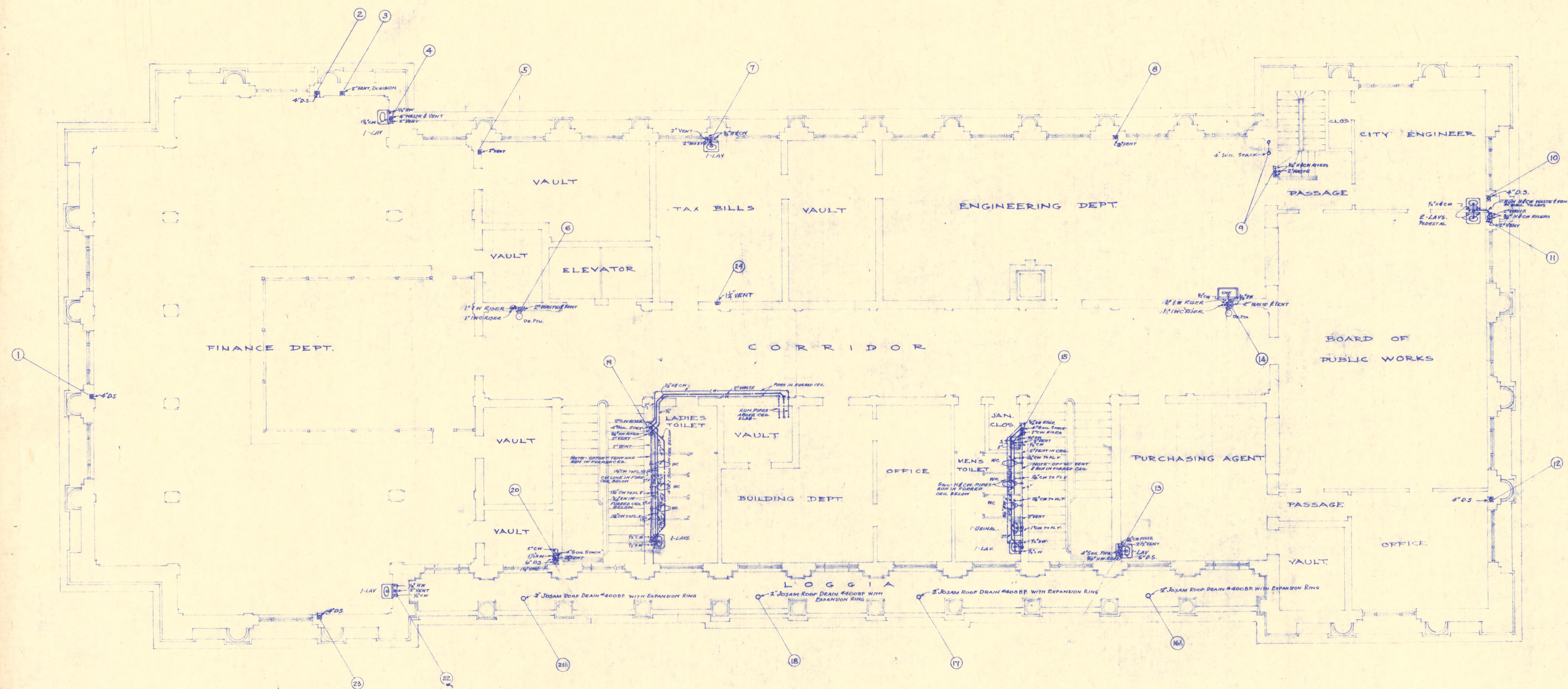
SCALE \frac{1}{8}'' = 1'-0'' FIRST FLOOR PLAN
