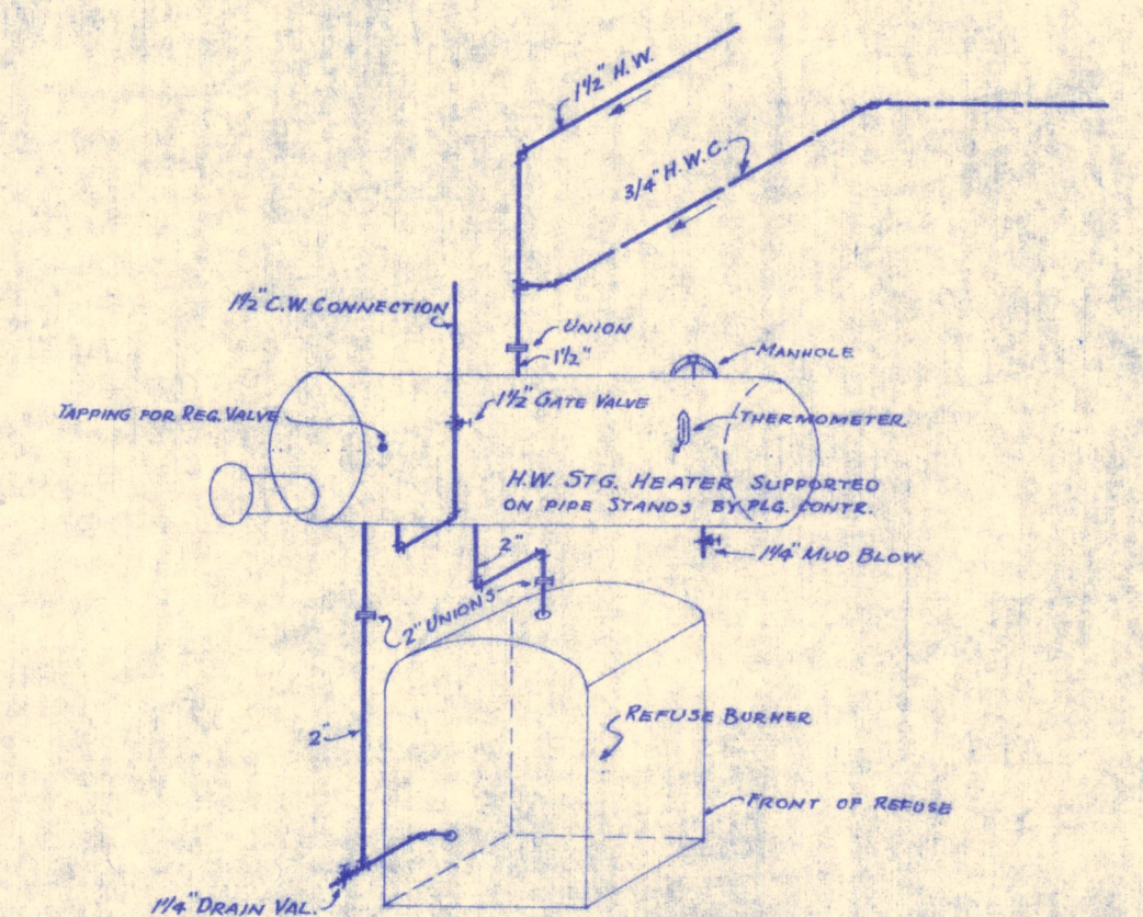
SKETCH OF PIPING TO H.W. STG. HEATER Not to scale
