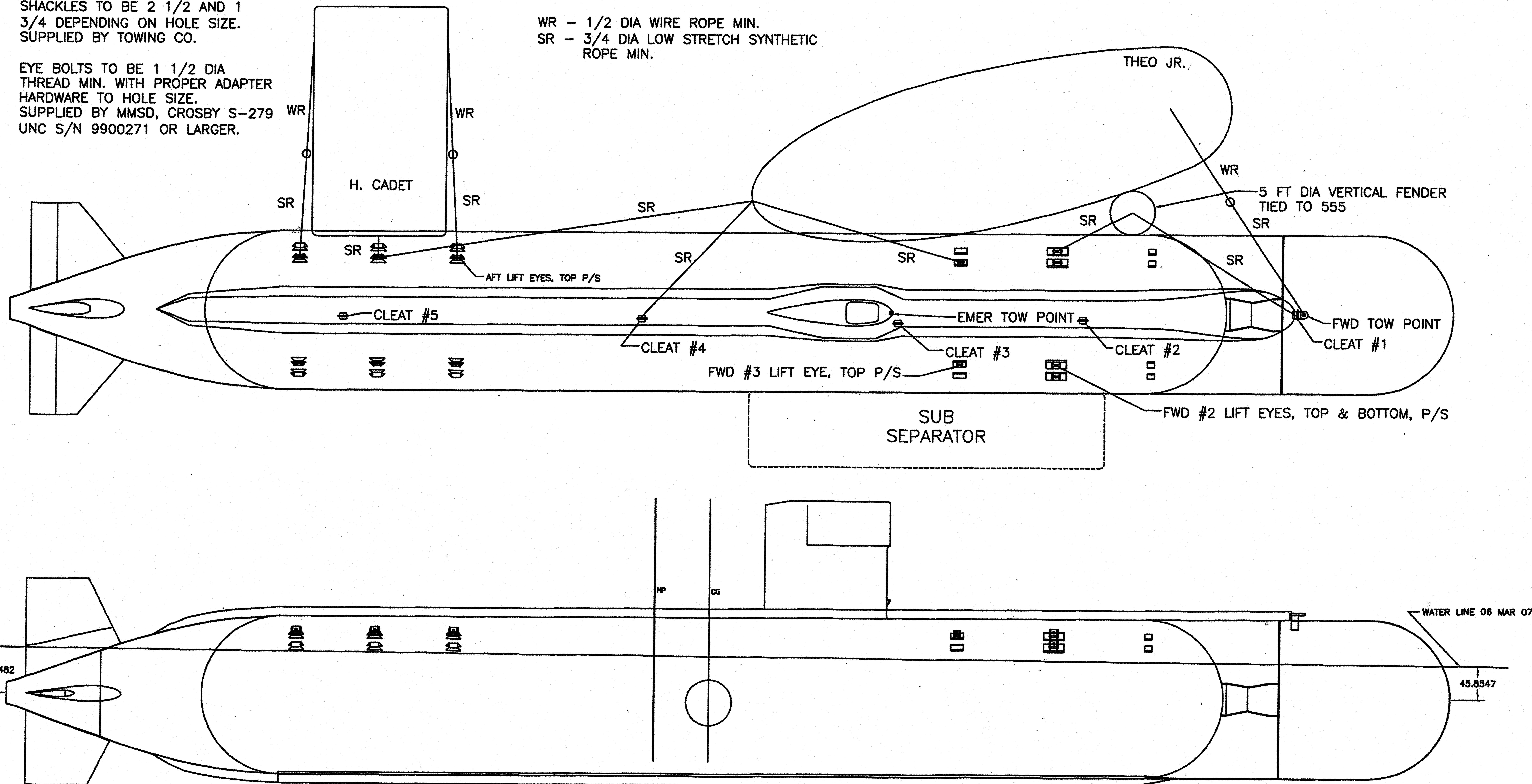
USS DOLPHIN TOW PLAN ARRANGEMENT
