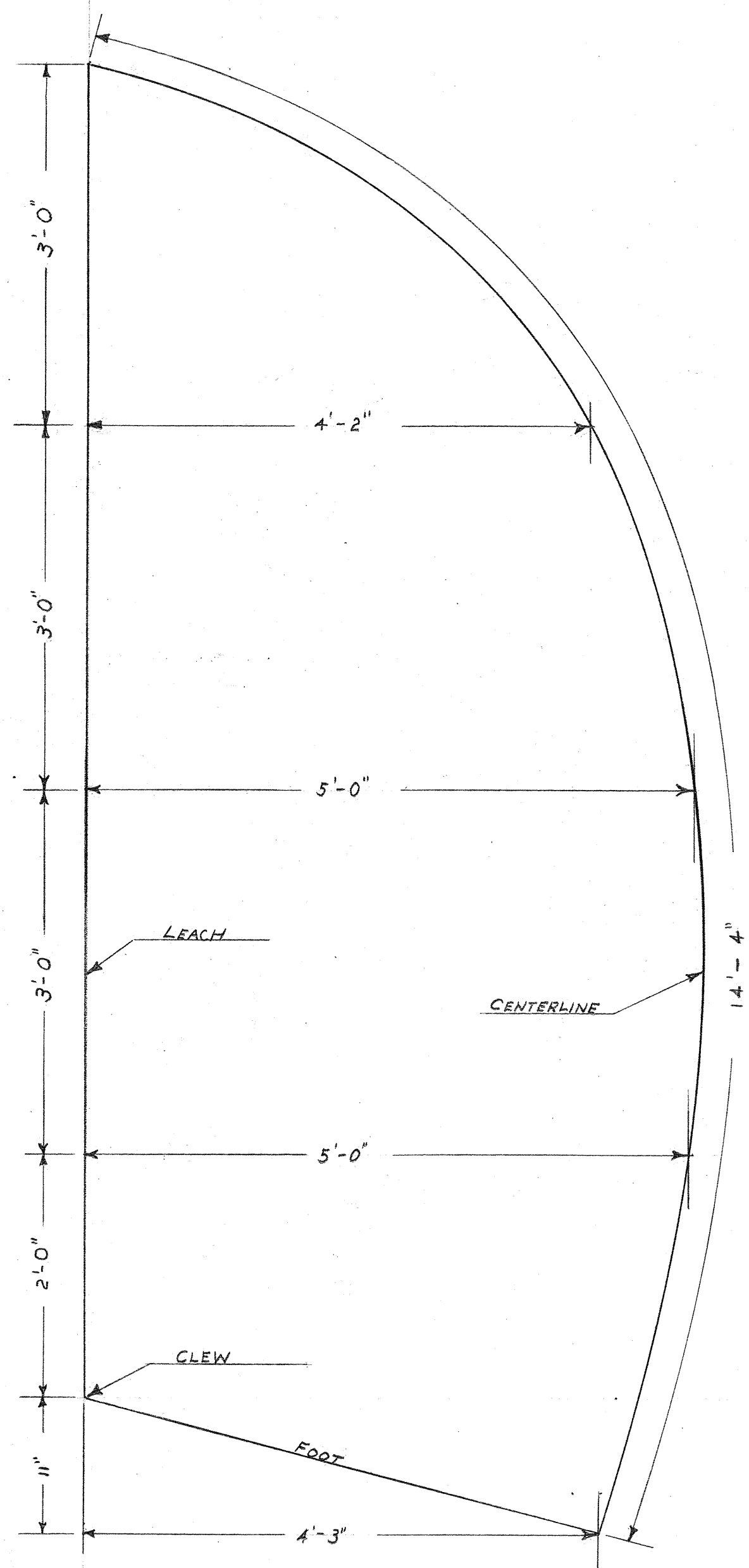
SPINNAKER FOLDED ALONG \phi
