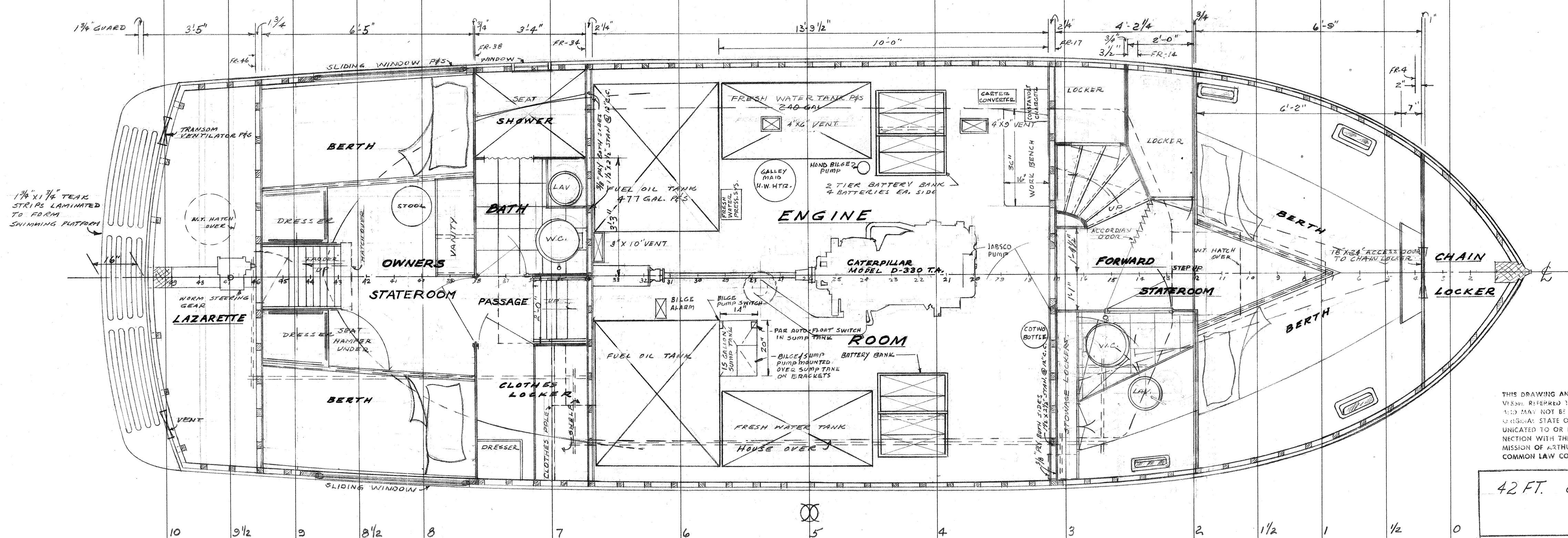
BELOW DECK ARRANGEMENT
