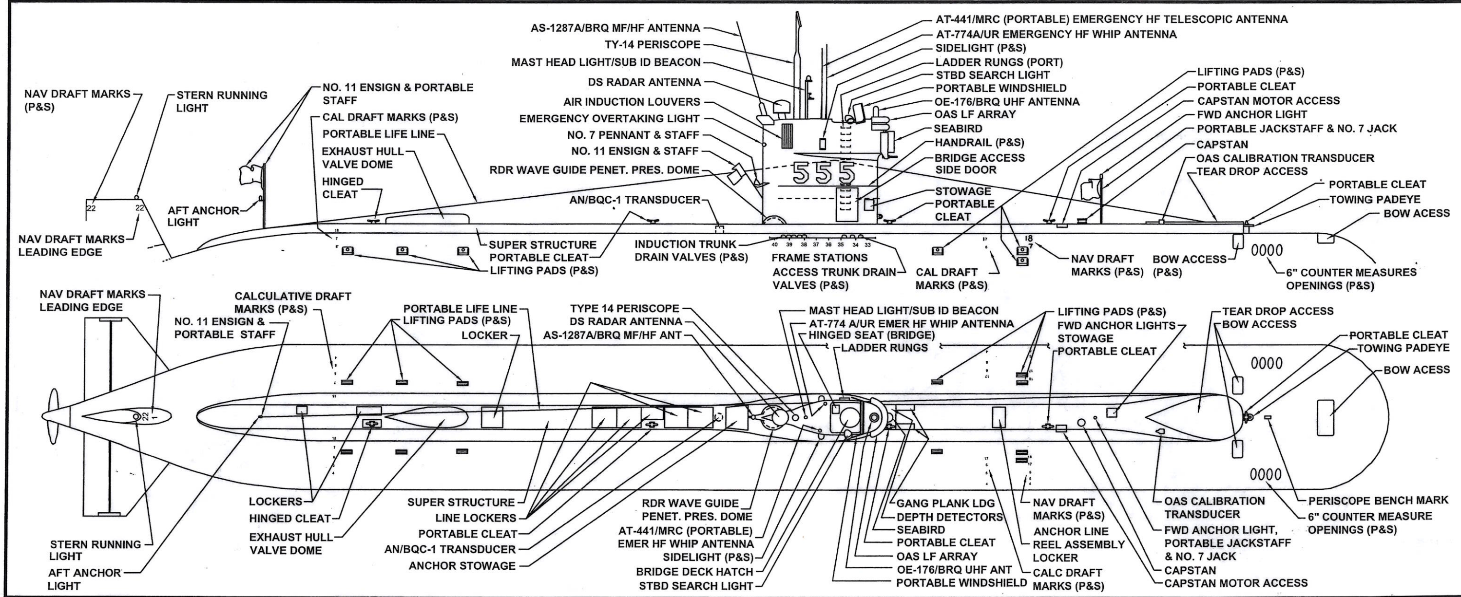
TOPSIDE ARRANGEMENT WITH DECK DRAINS
