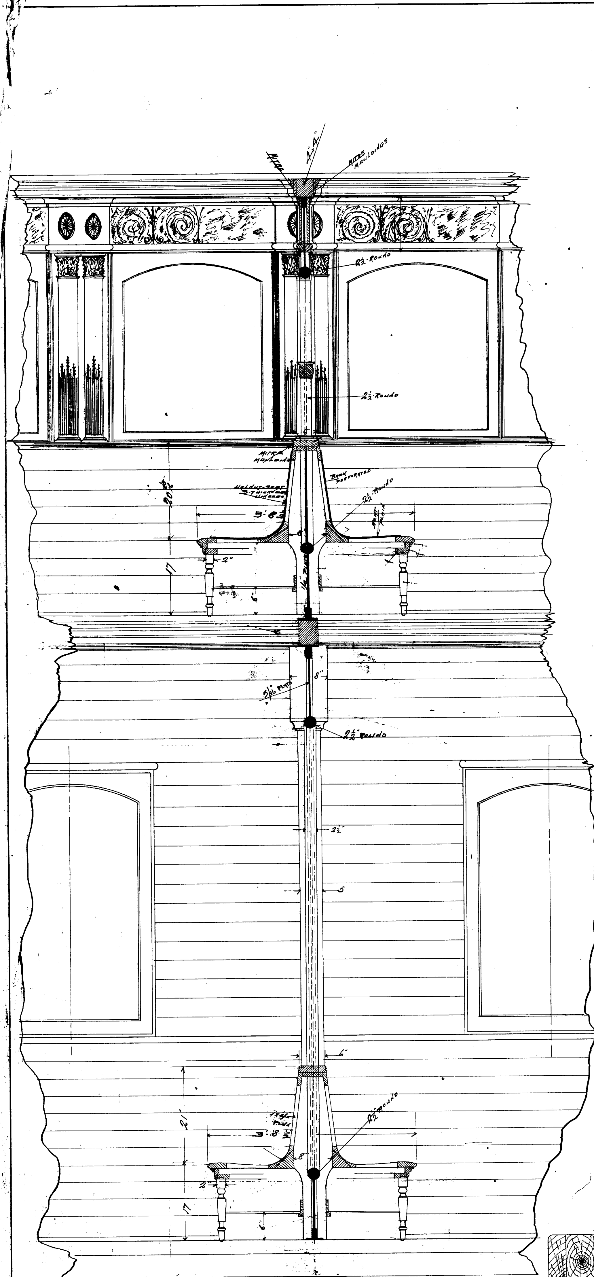
SECTION AT A-B
