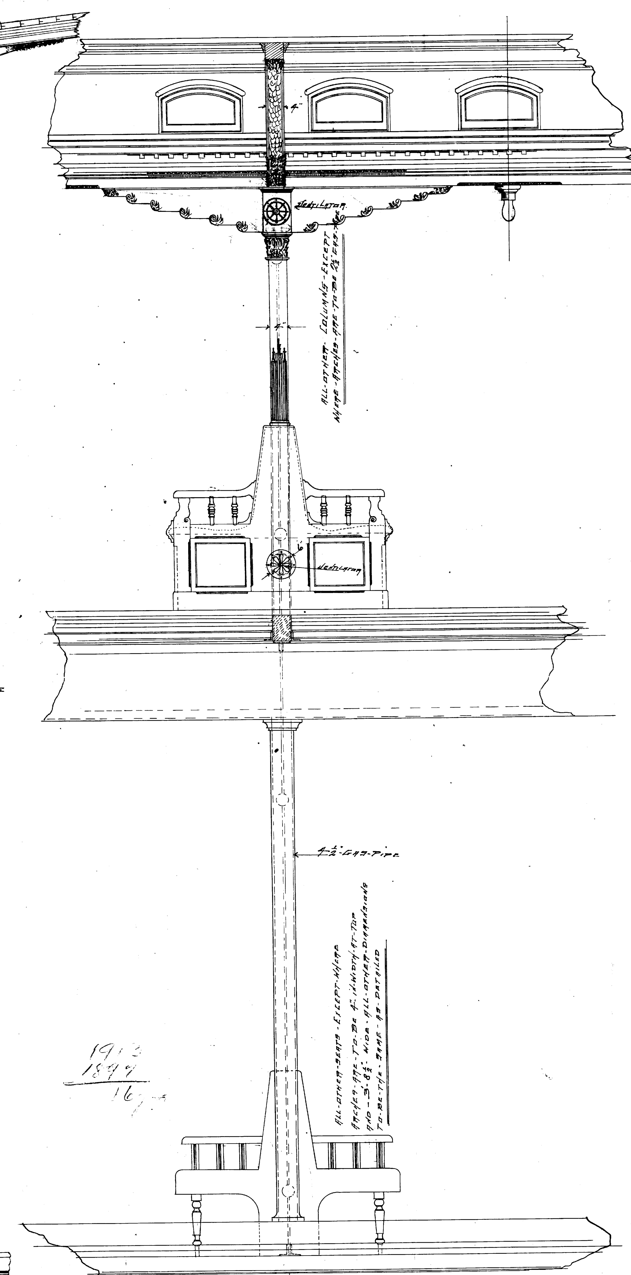
SECTION AT C-D
