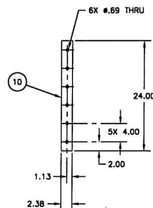
DETAIL 86-D
