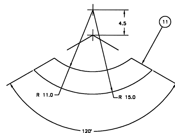
DETAIL 86-B
