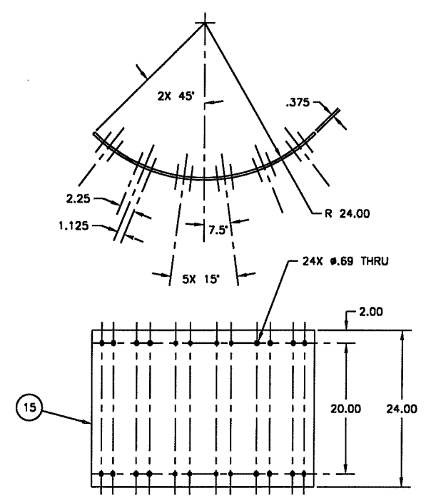
DETAIL 77-D .375 THK PLATE
