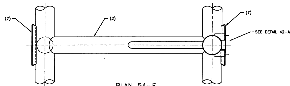
PLAN 54-E
