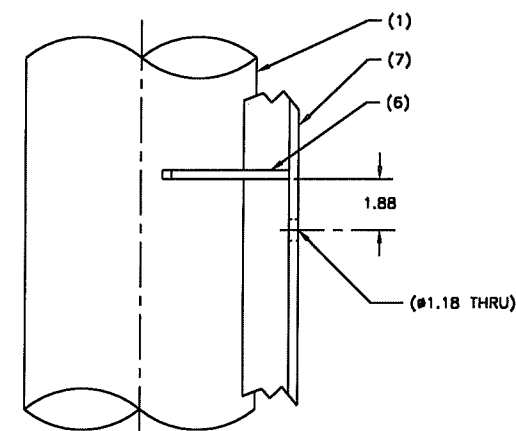
PLAN 42-C SCALE: 3"=1'-0" TYP PLAN VIEW OF DETAIL 42-A TYP LOCATION OF GUSSET
