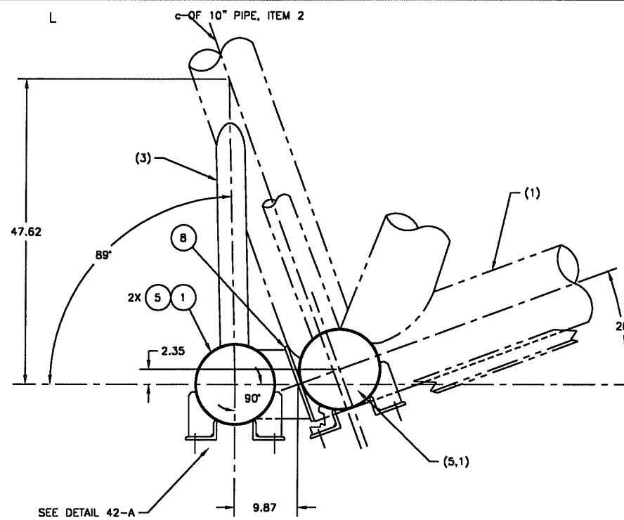
PLAN 44-E
