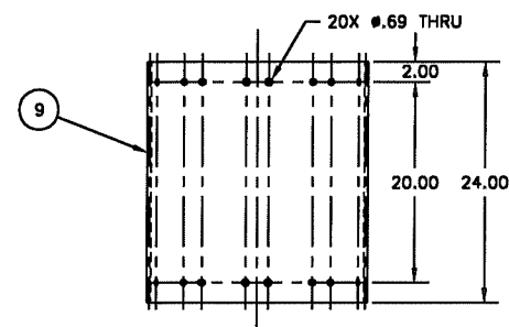
DETAIL 88-D
