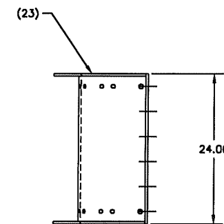
END PIER GUARD ATTACHMENT WELDMENT ASSY 85-D
