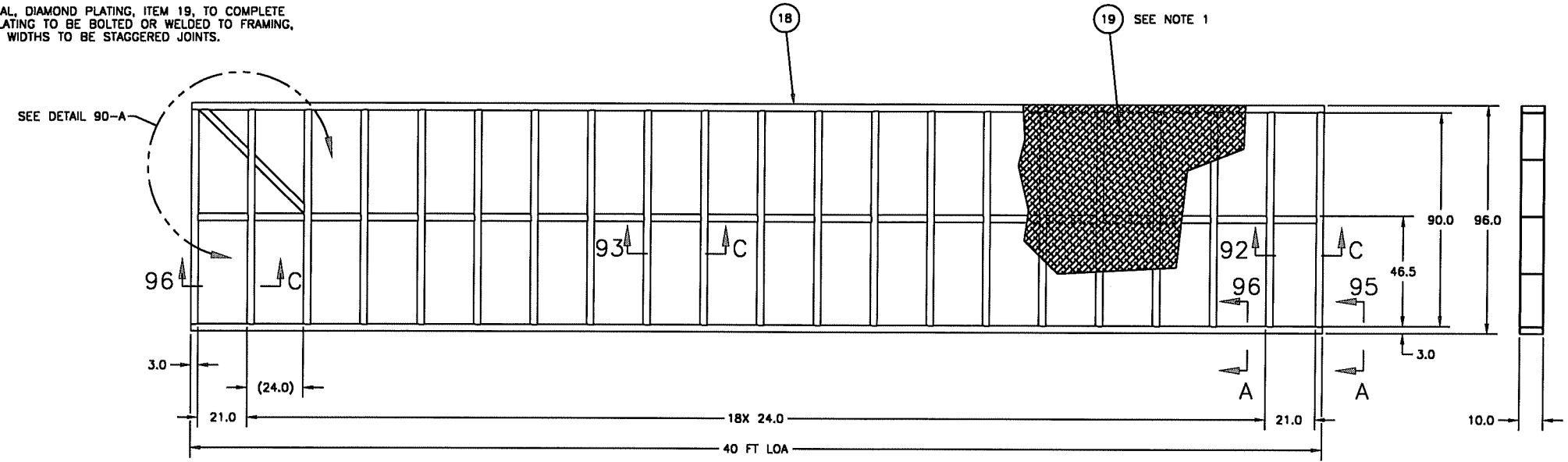
DECK FRAMING DETAIL 93-D .25 THK PLATE
