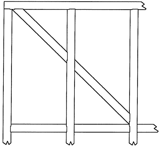
DETAIL 90-A SCALE: 1 1/2"=1'-0 TYP WELD JOINT DETAIL
