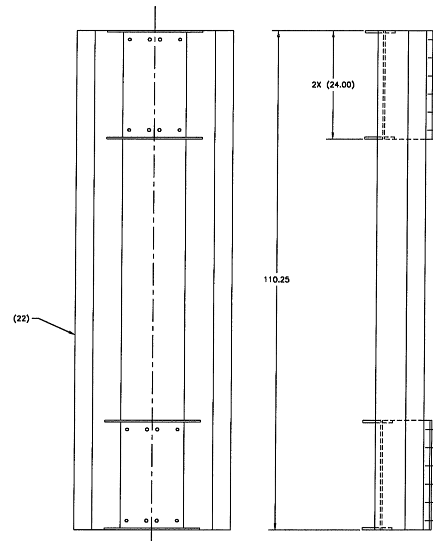
END PIER GUARD WELDMENT ASSY 82-A
