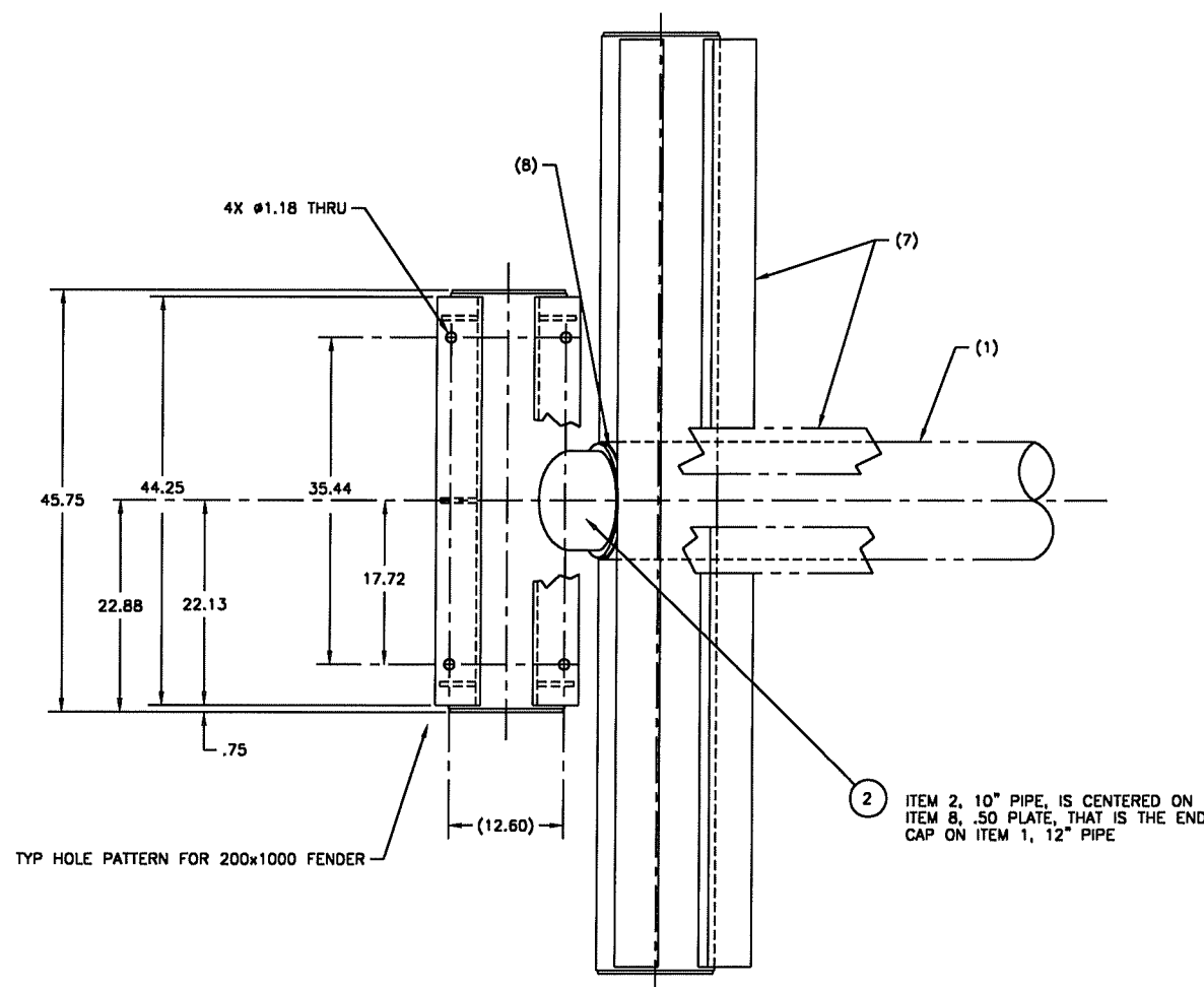
VIEW 44-A
