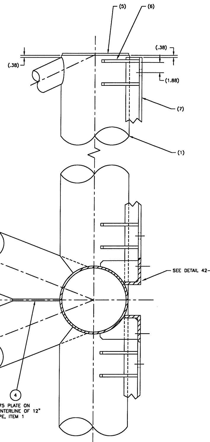
DETAIL 50-B
