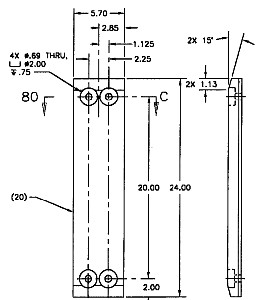
DETAIL 79-A SCALE: 3" = 1'-0" CUT FROM 1.5" UHMW-PE
