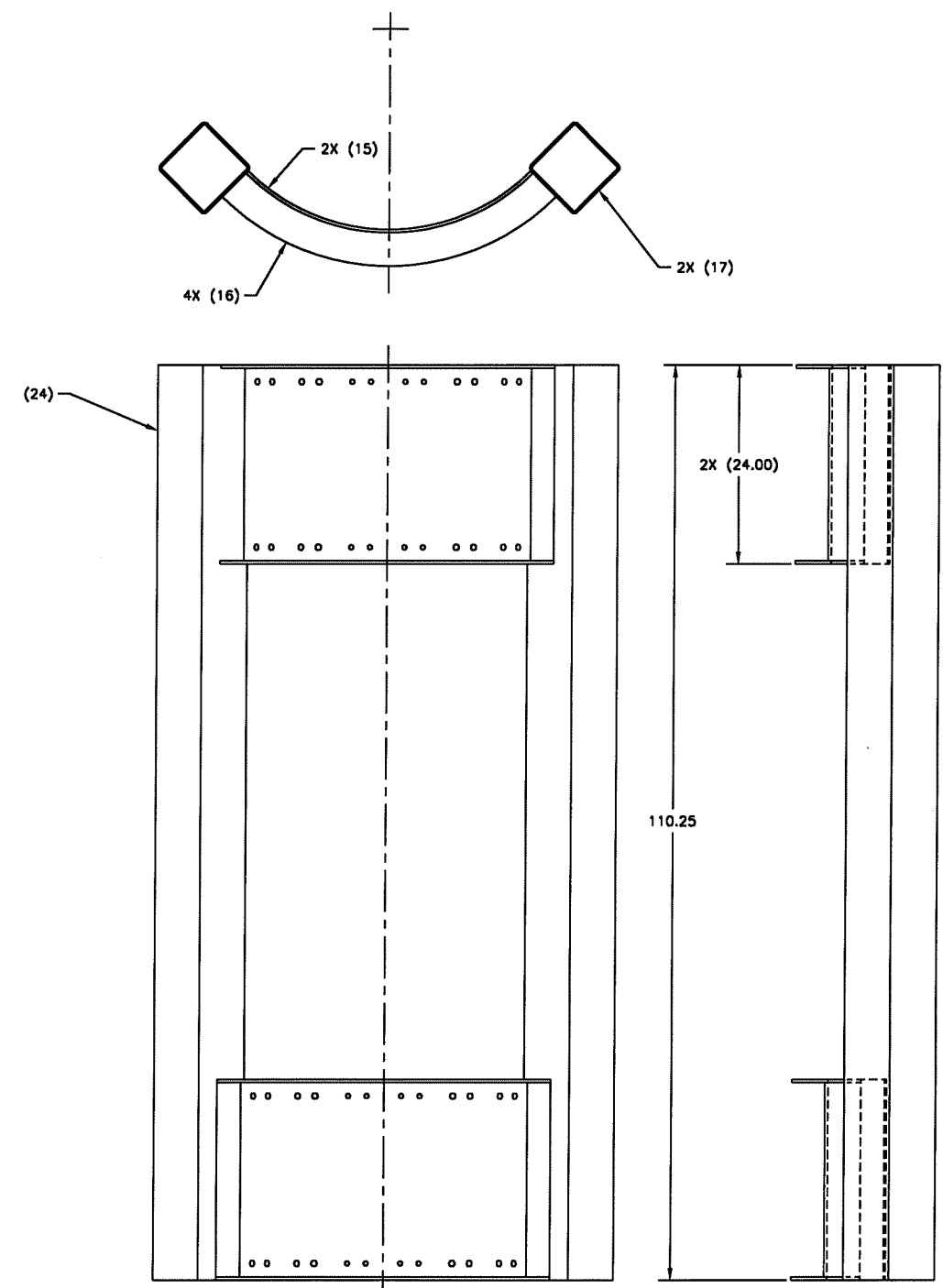
MID PIER GUARD WELDMENT ASSY 75-A
