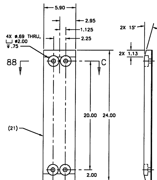
DETAIL 88-A
