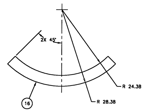
DETAIL 77-D .50 THK PLATE
