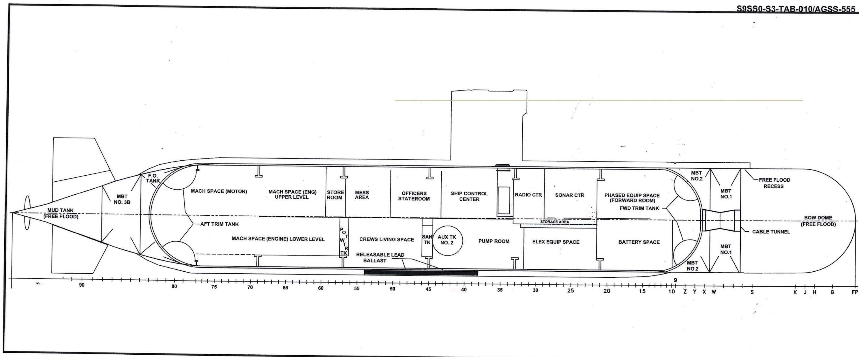
INBOARD PROFILE WITH RELEASABLE LEAD BALLAST REF: AGSS 555-845-2100233, 121-2100319
