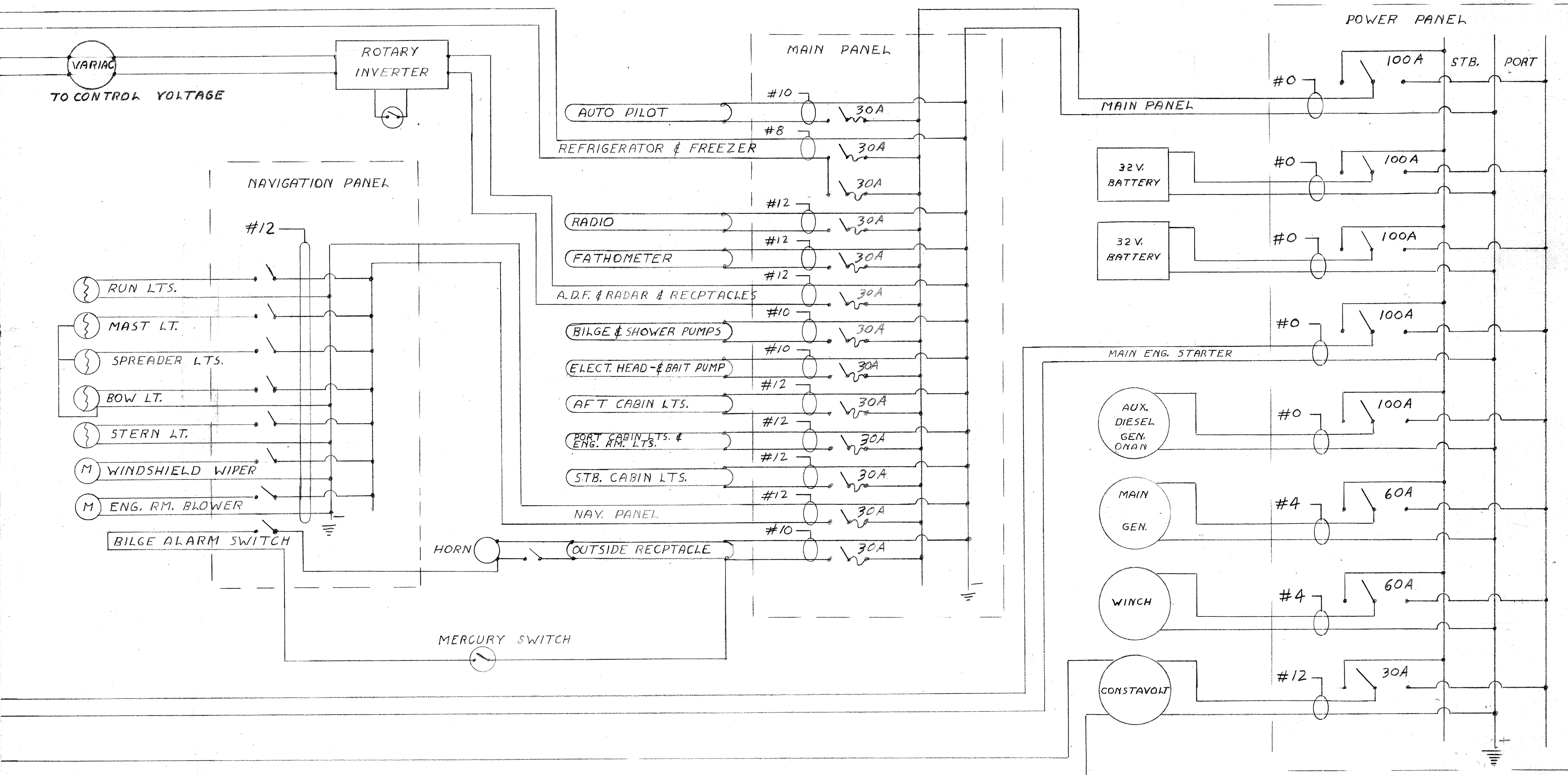
SCHEMATIC WIRING DIAGRAM 47' M.S. #1 KETTENBURG 10/23/58
