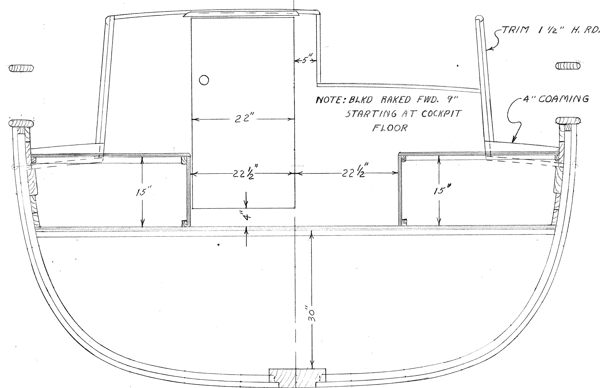
SECTION THRU COCKPIT AT FR. 42 LOOKING FWD.
