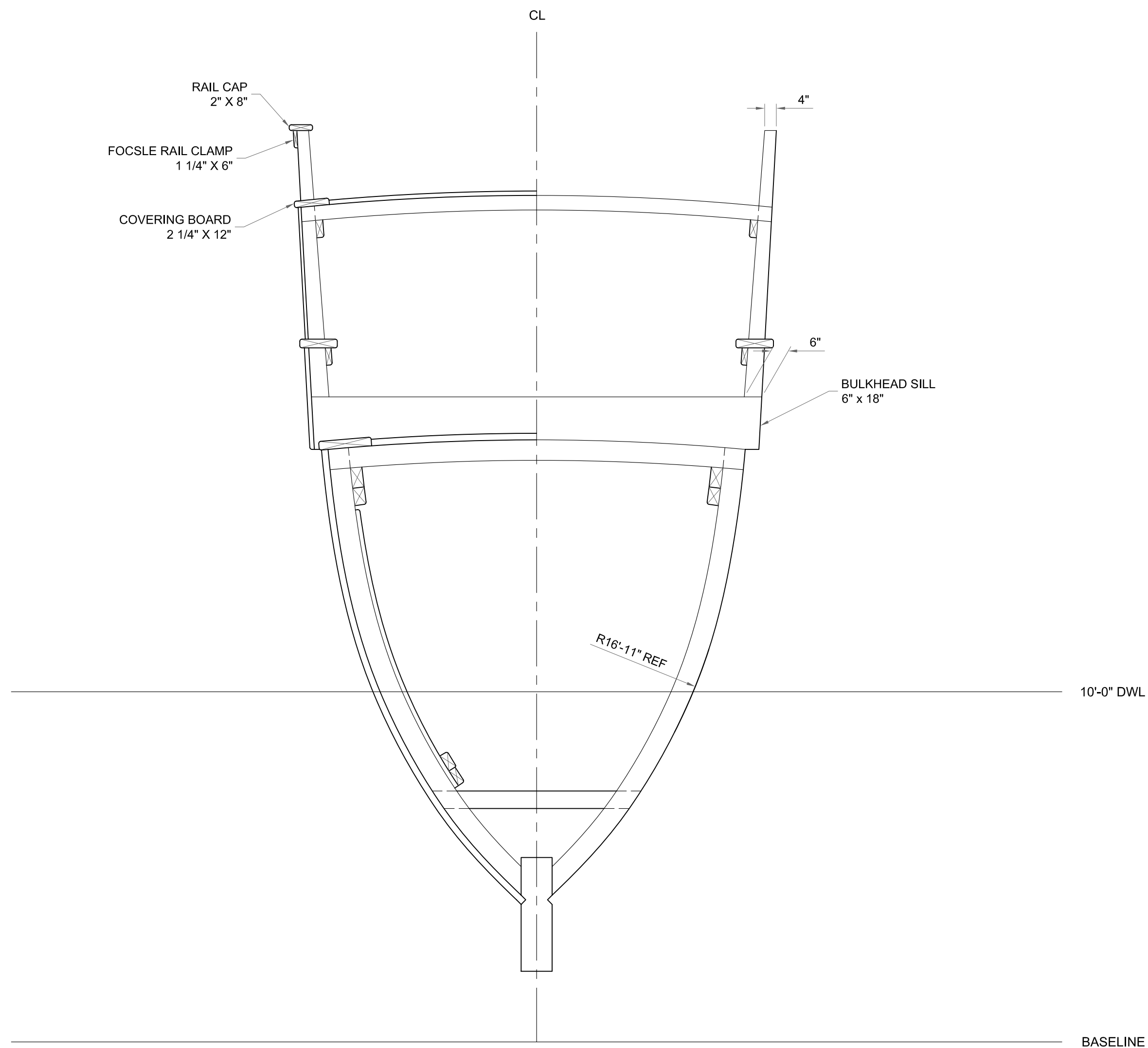
FRAME 6 LOOKING AFT
