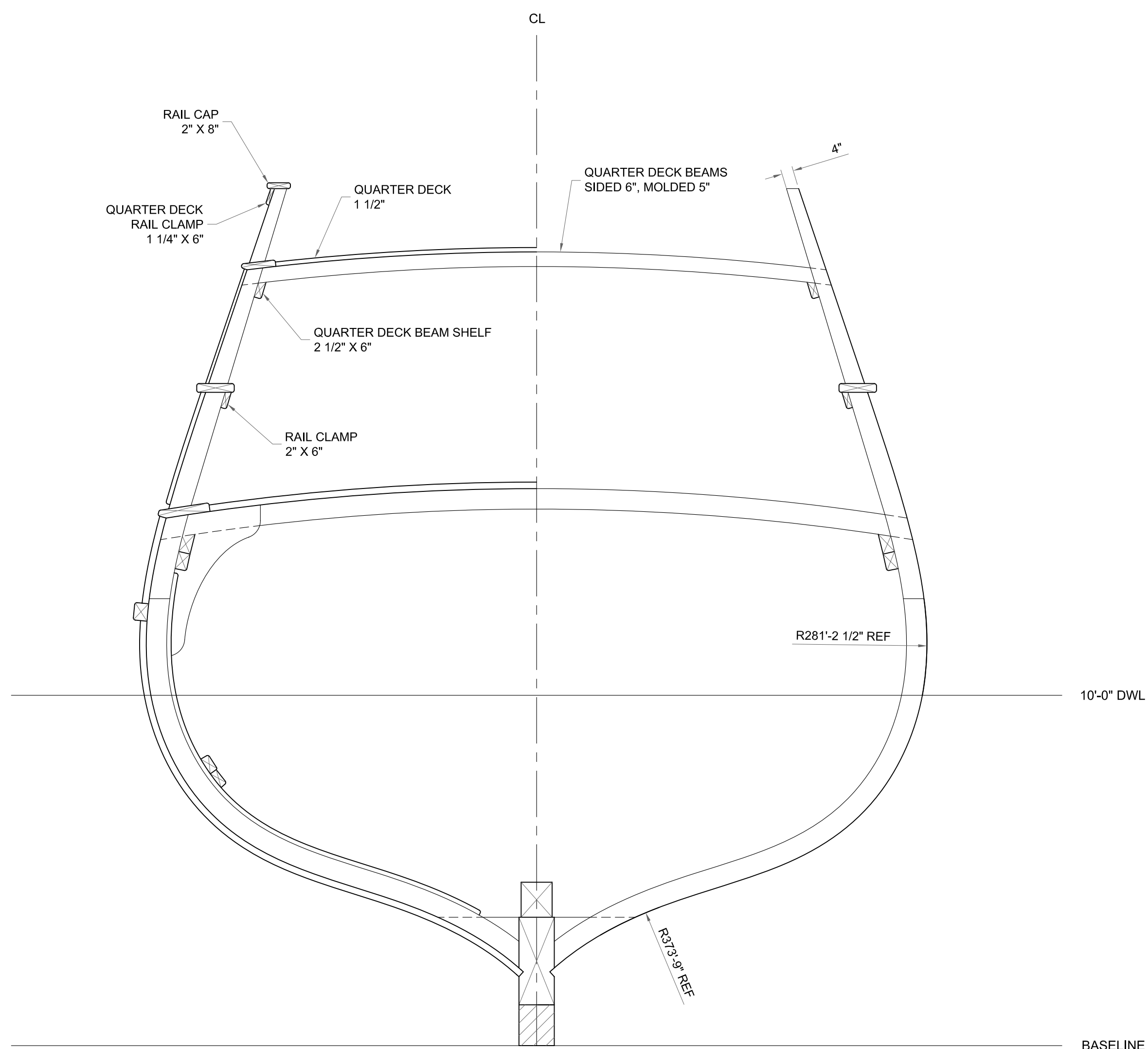
FRAME 50 LOOKING FWD
