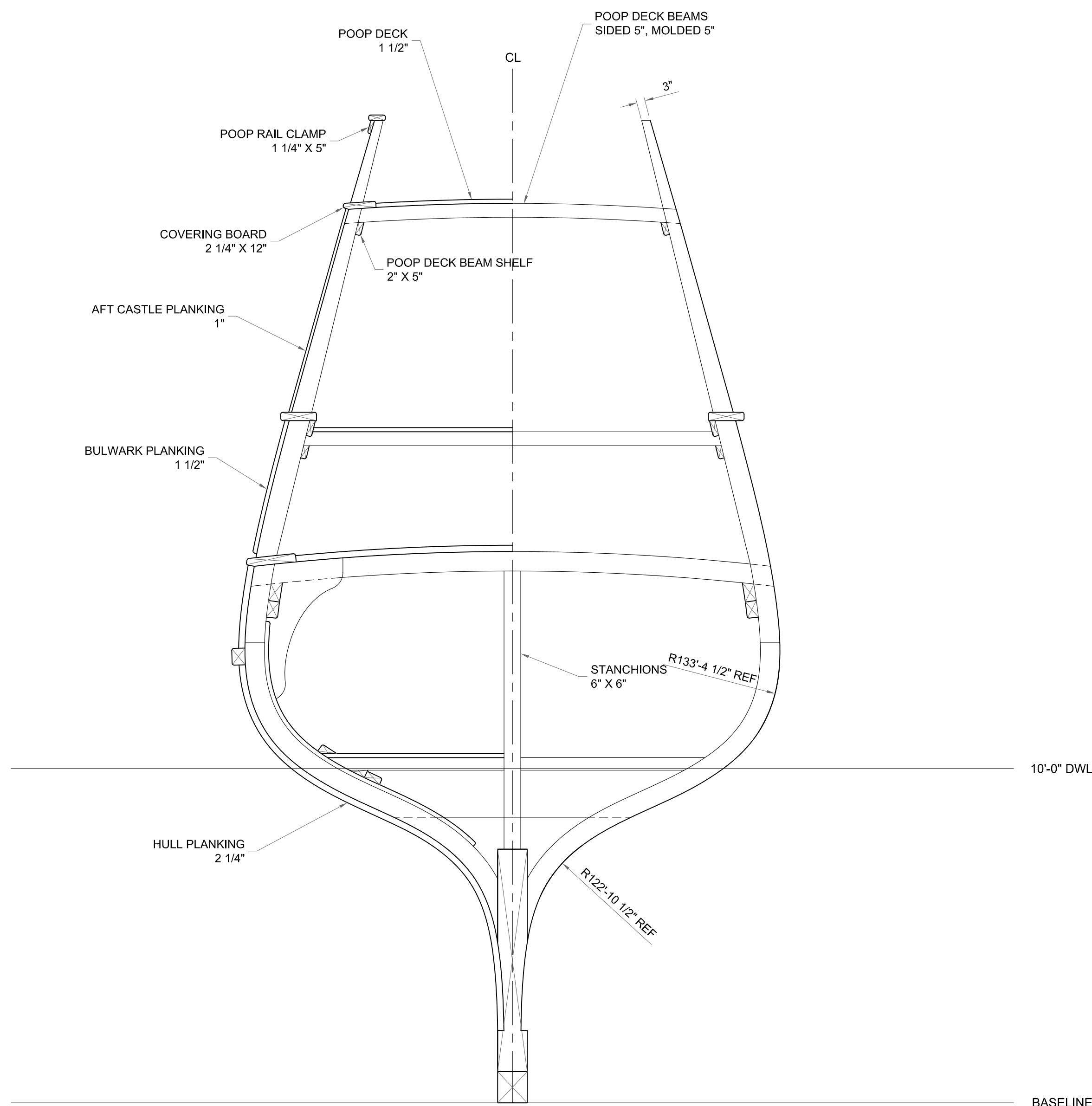
FRAME 68 LOOKING FWD
