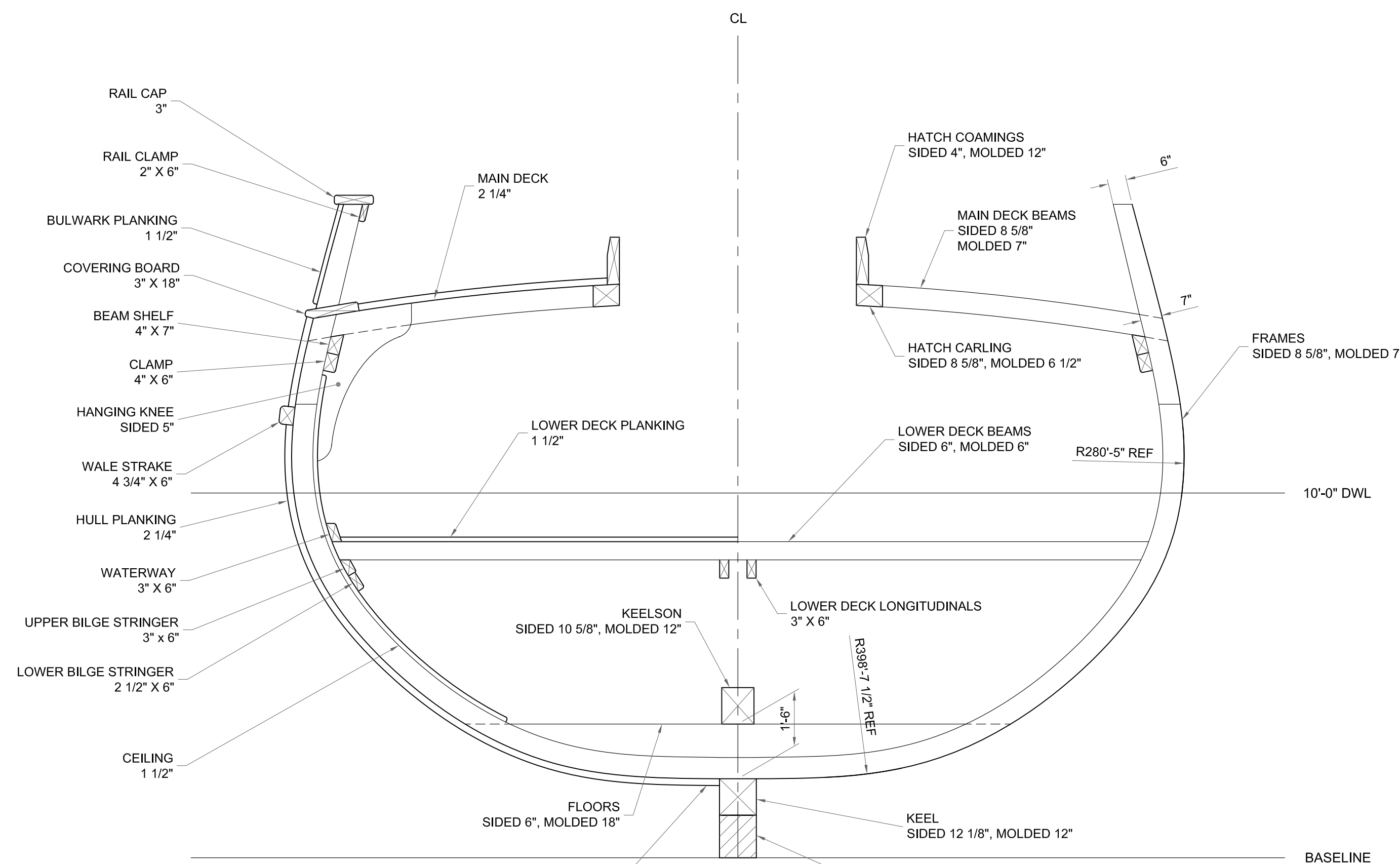
FRAME 32 LOOKING FWD
