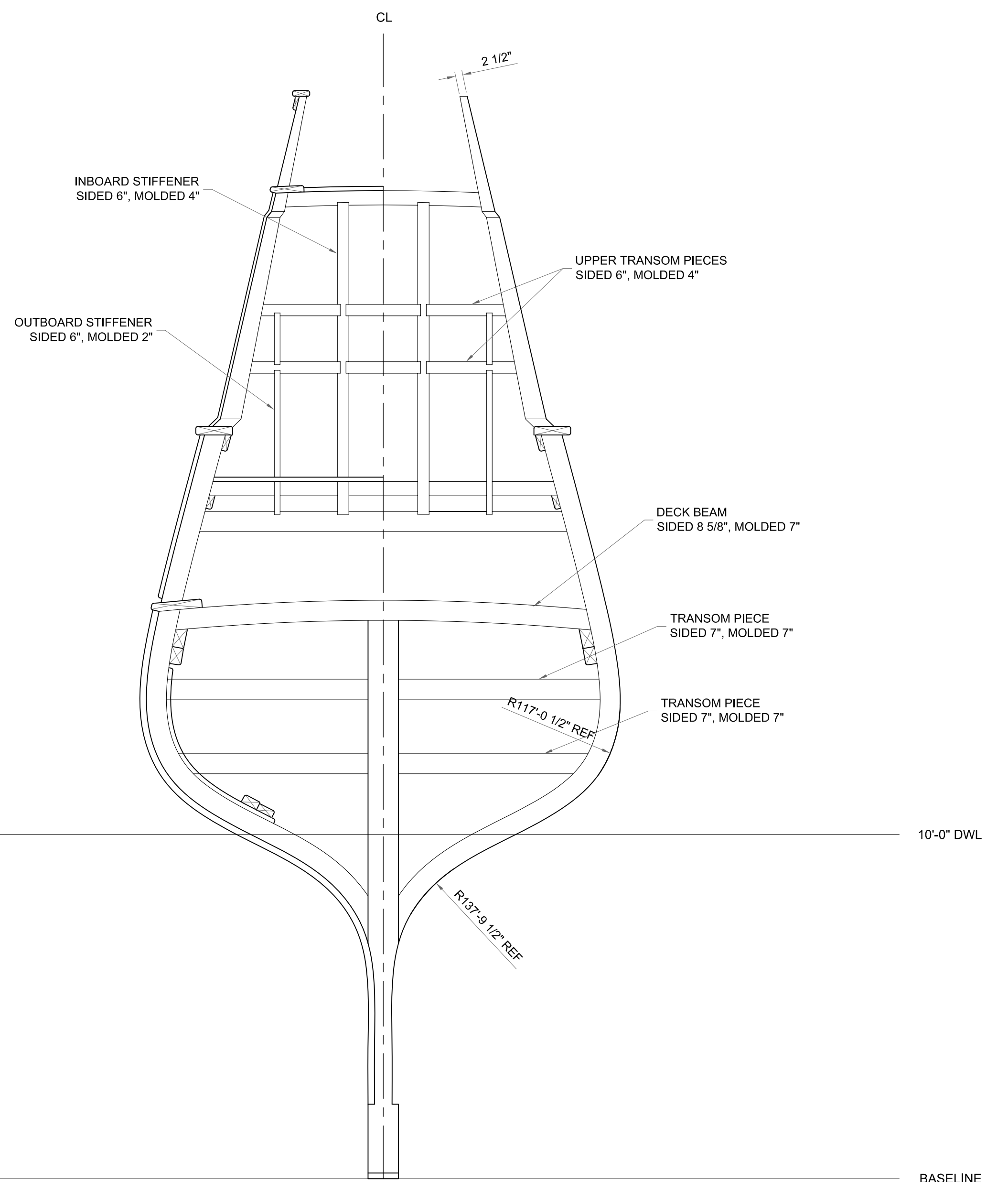
TRANSOM LOOKING AFT
