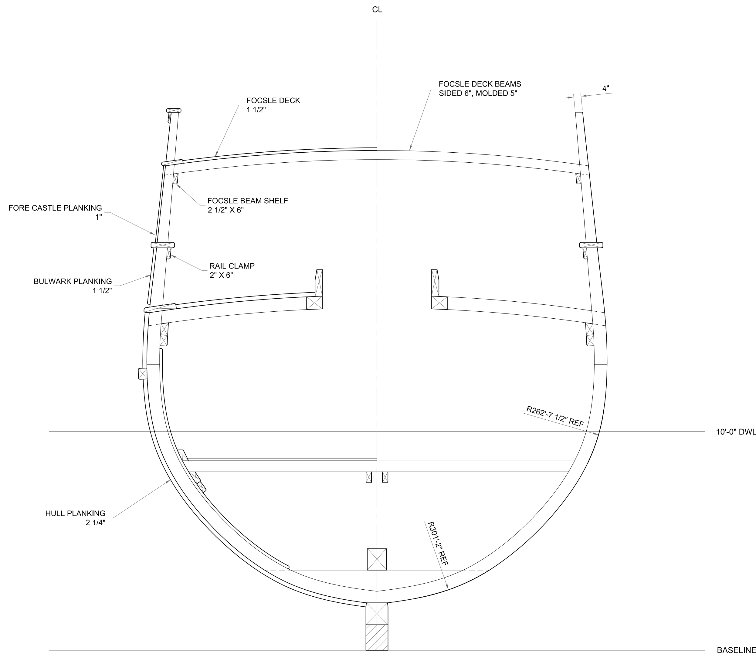
FRAME 18 LOOKING FWD
