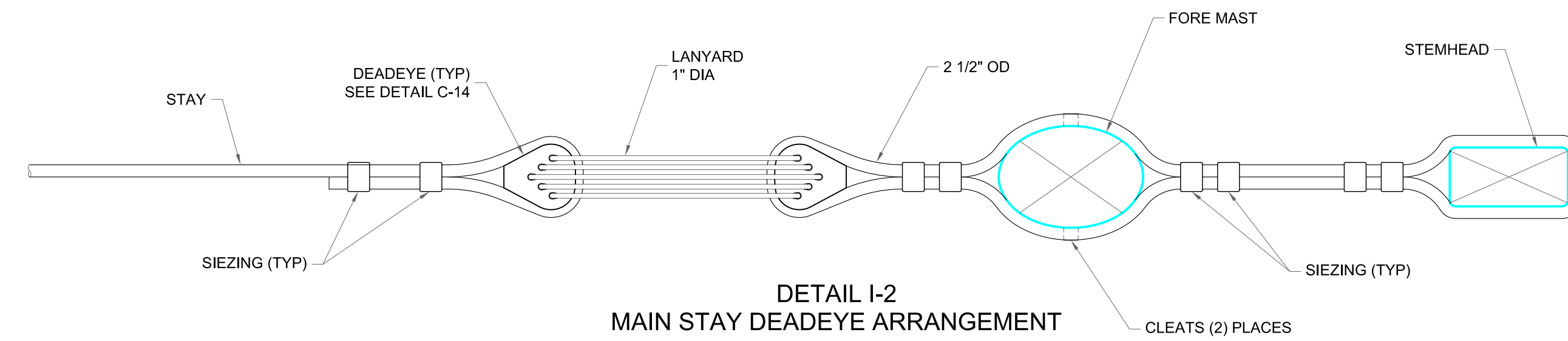
DETAIL I-2 MAIN STAY DEADEYE ARRANGEMENT SCALE: 1/2" = 1'-0"
