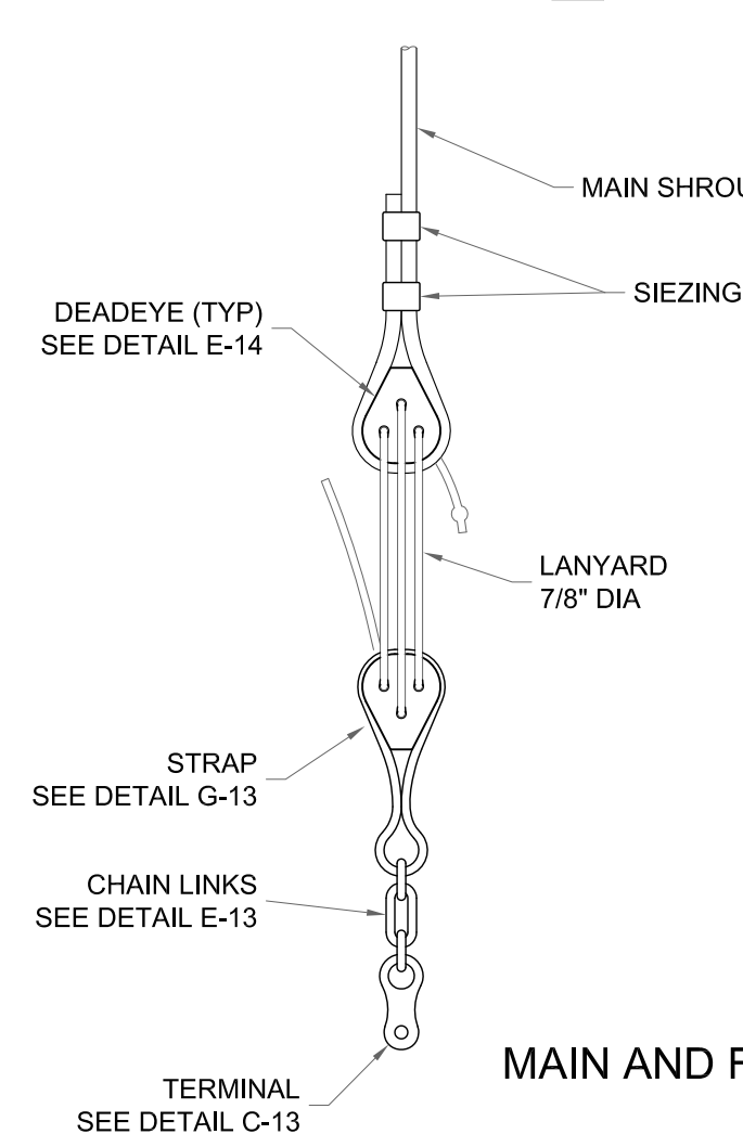
ELEVATION C-3 RIGGING PROFILE
