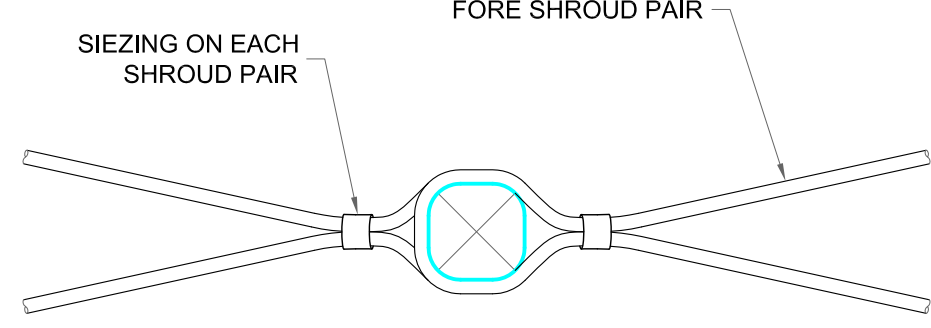
SECTION I-6 FOREMAST SHROUDS SCALE: 1/2" = 1'-0"
