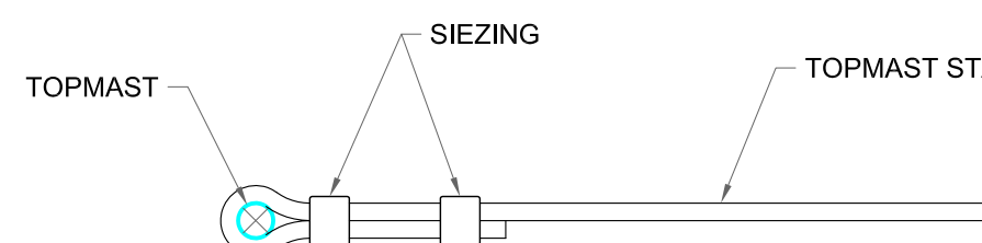
DETAIL H-2 TOPMAST STAY ARRANGEMENT SCALE: 1/2" = 1'-0"
