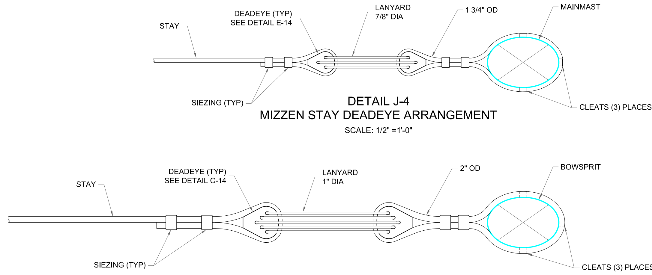
DETAIL J-4 MIZZEN STAY DEADEYE ARRANGEMENT SCALE: 1/2" = 1'-0"
