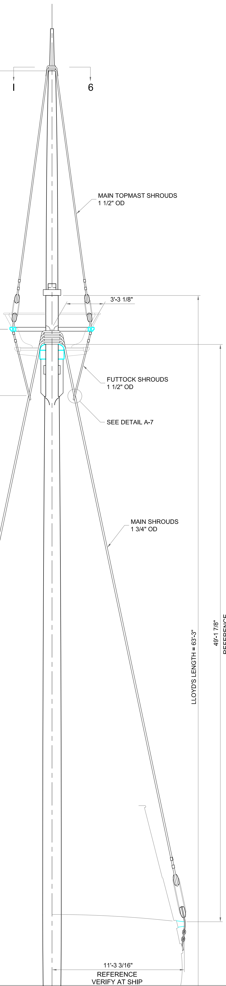
SECTION I-6 FOREMAST SHROUDS SCALE: 1/2" = 1'-0"
