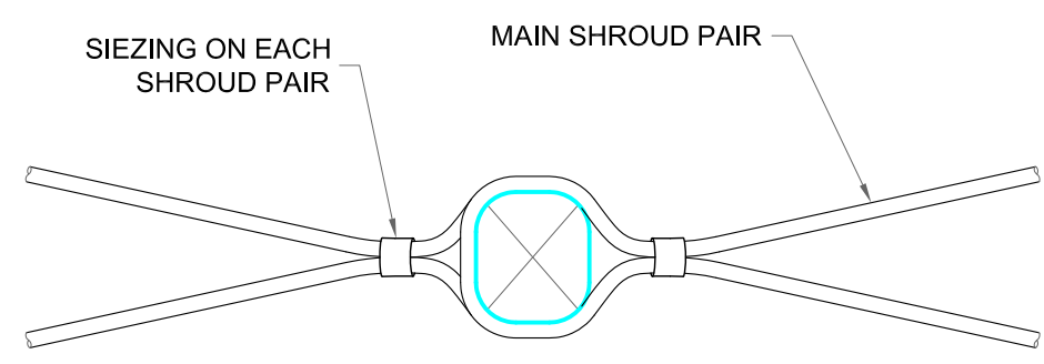
SECTION I-8 MAIN MAST SHROUDS SCALE: 1/2" = 1'-0"
