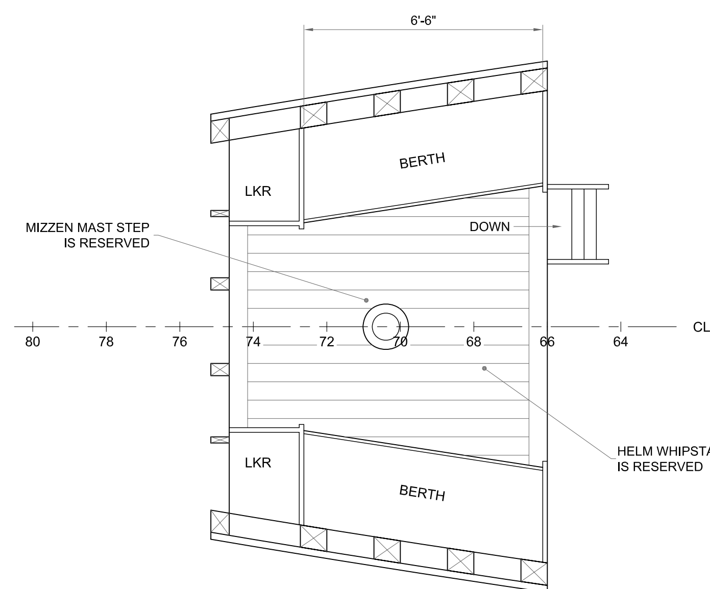
PLAN E-7 HELM DECK ARRANGEMENT
