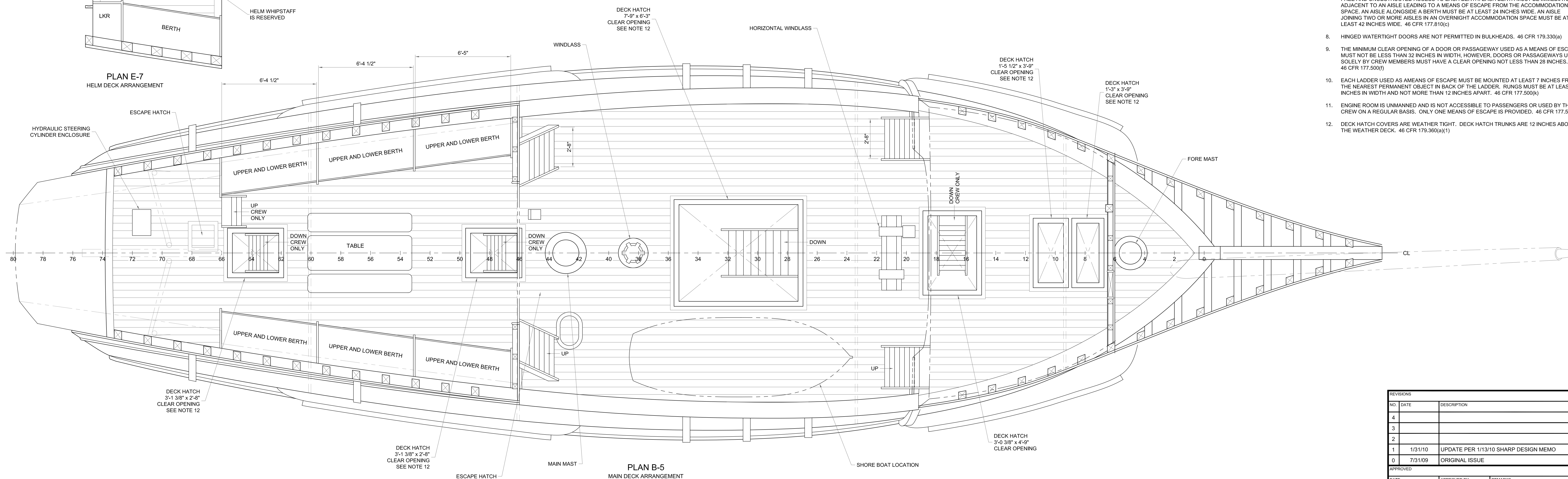
PLAN B-5 MAIN DECK ARRANGEMENT
