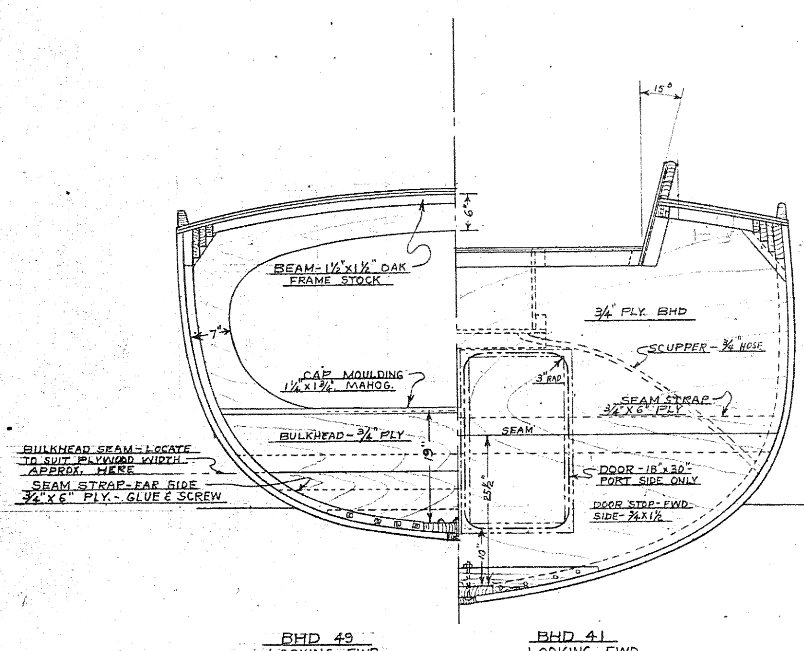
BHD 49 LOOKING FWD
