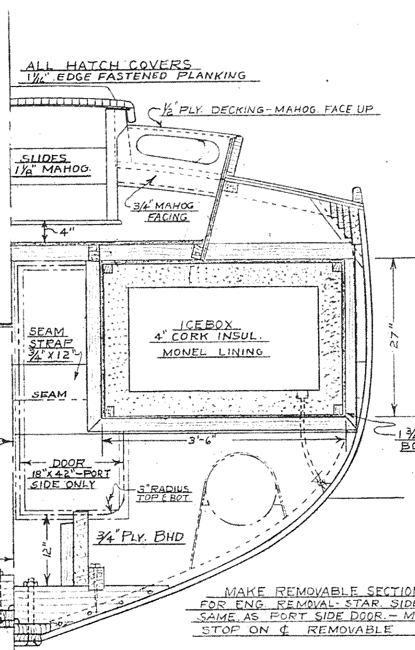
BHD 31 LOOKING FWD
