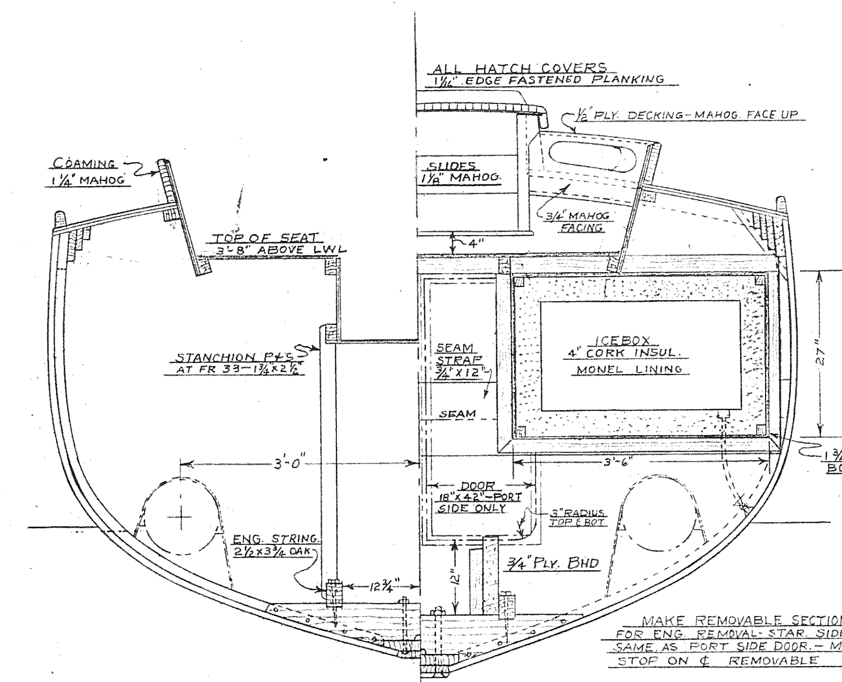
FRAME 36 LOOKING FWD
