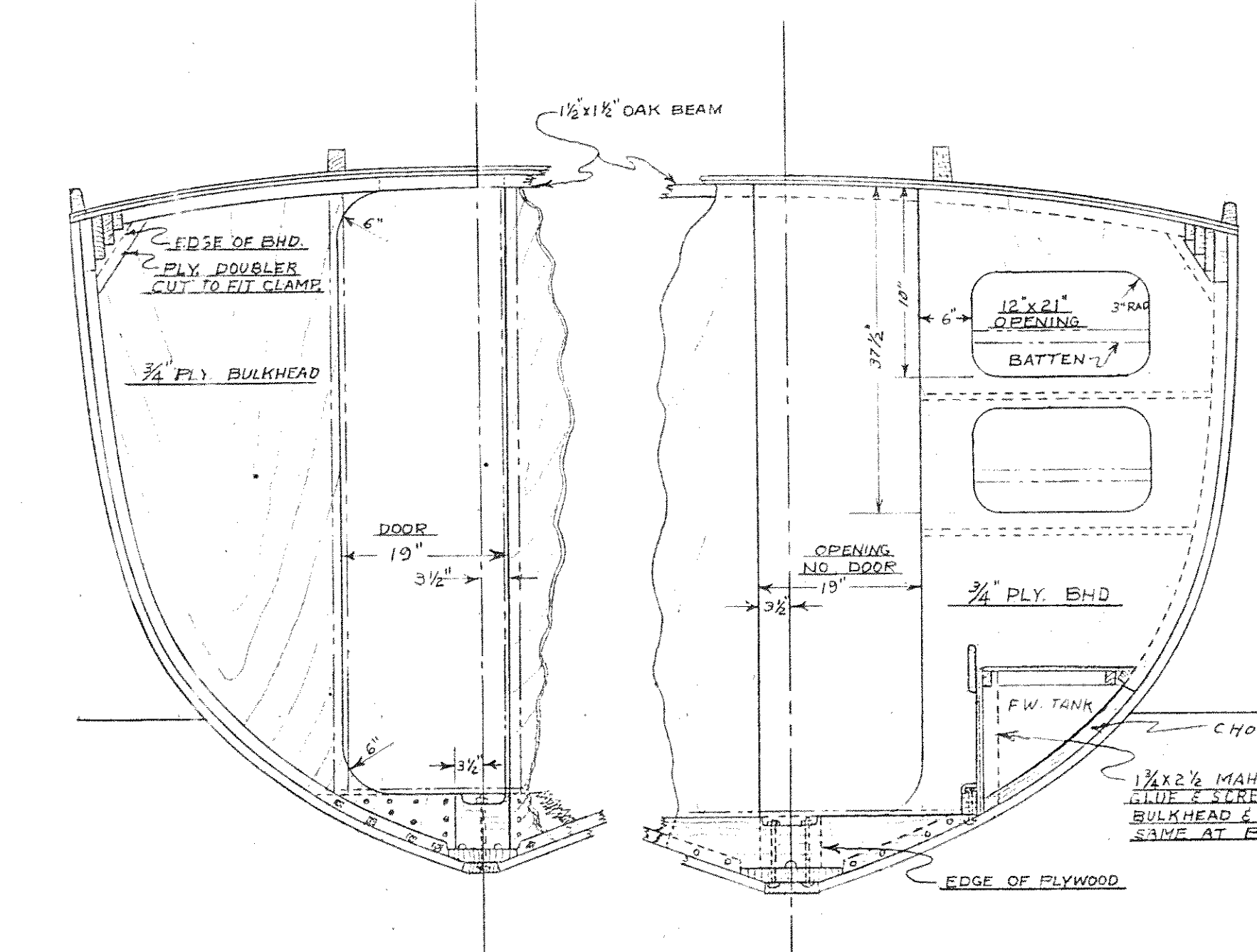
BHD 14 STATIONED SIDE LOOKING AFT
