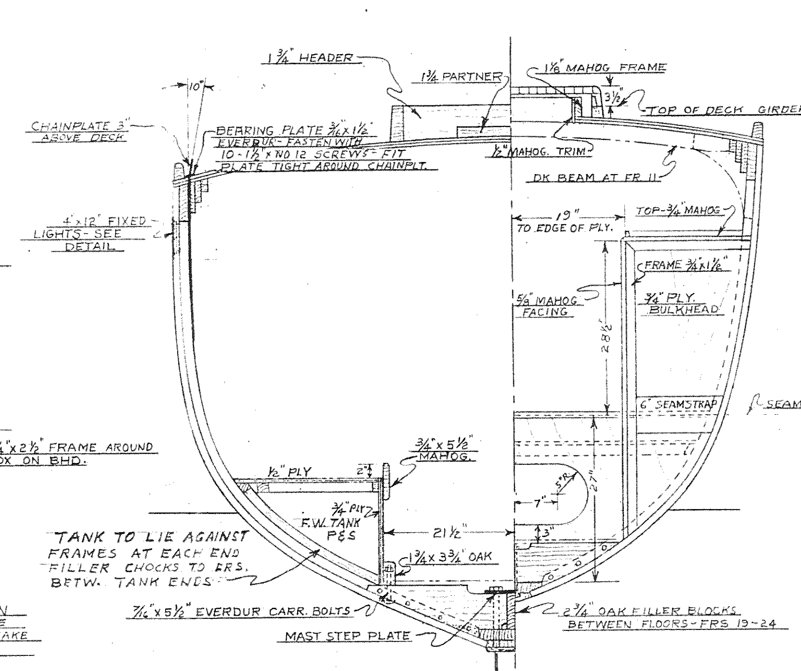
STATION 4 LOOKING FWD TO TR. 20
