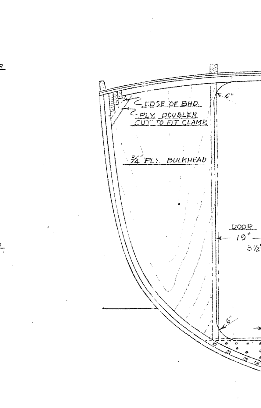
BHD 14 STATIONED SIDE LOOKING AFT
