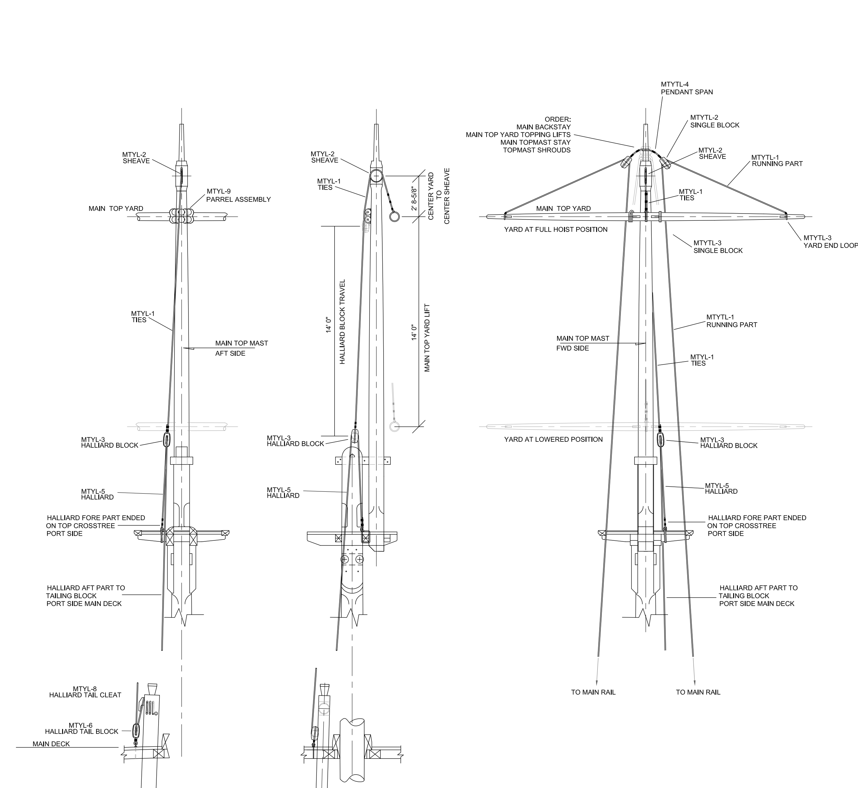
DETAIL: F-18 MAIN TOP YARD TIES, HALLIARD, HALLIARD BLOCKS, SCALE: 1/4" = 1'-0"
