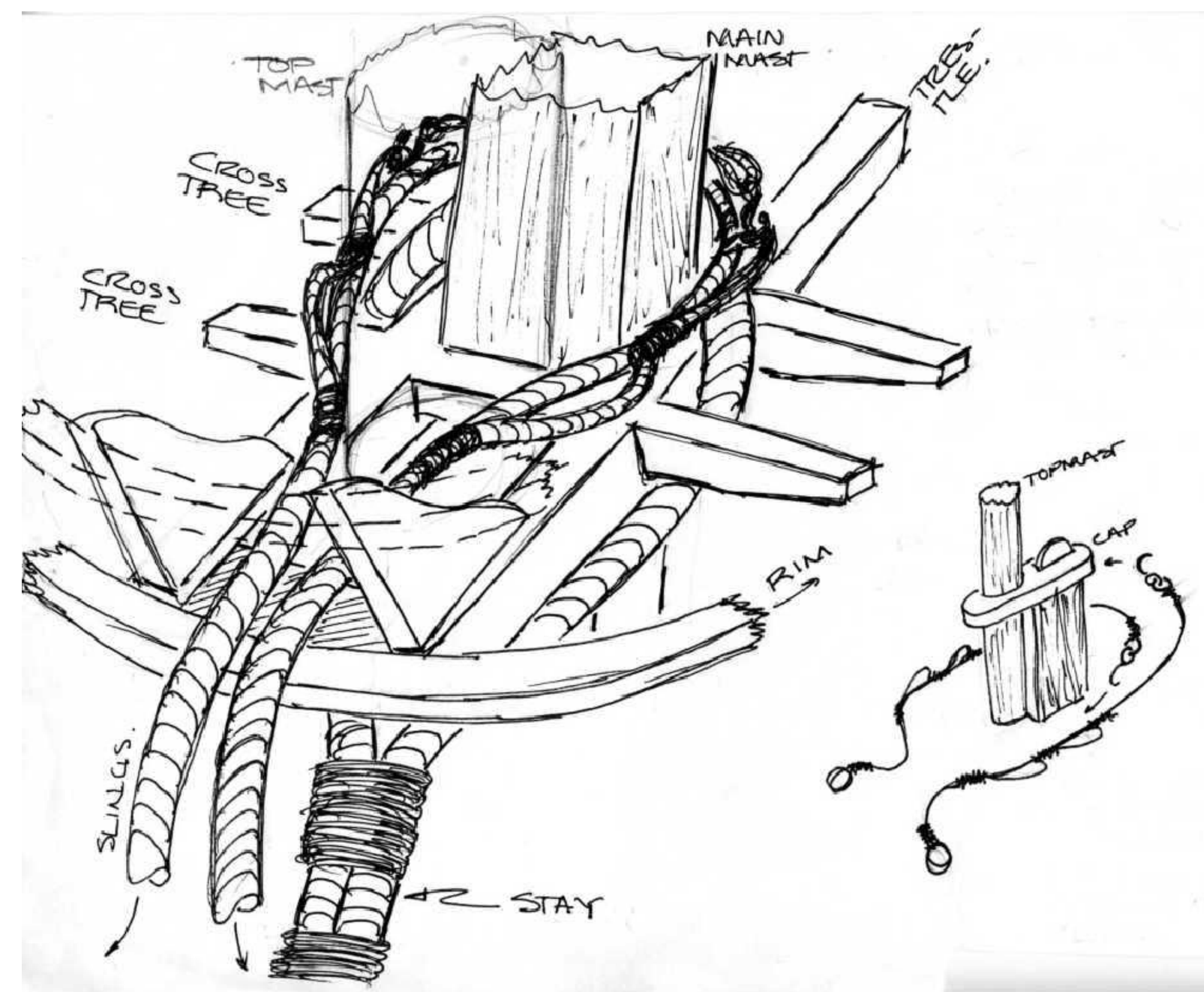
DETAIL: D-20 MAIN YARD SLINGS NOT TO SCALE
