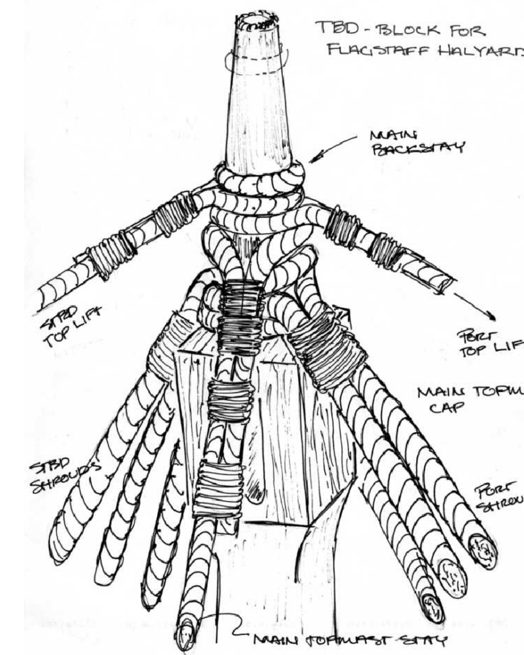
DETAIL: D-19 MAIN TOPMAST MASTHEAD NOT TO SCALE
