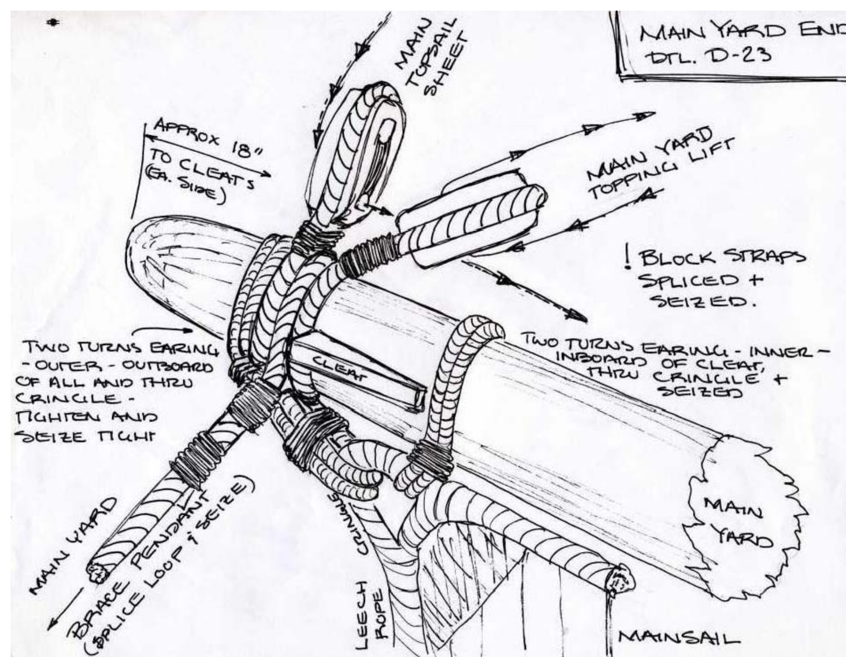
DETAIL: D-23 MAIN YARD END LAYOUT NOT TO SCALE
