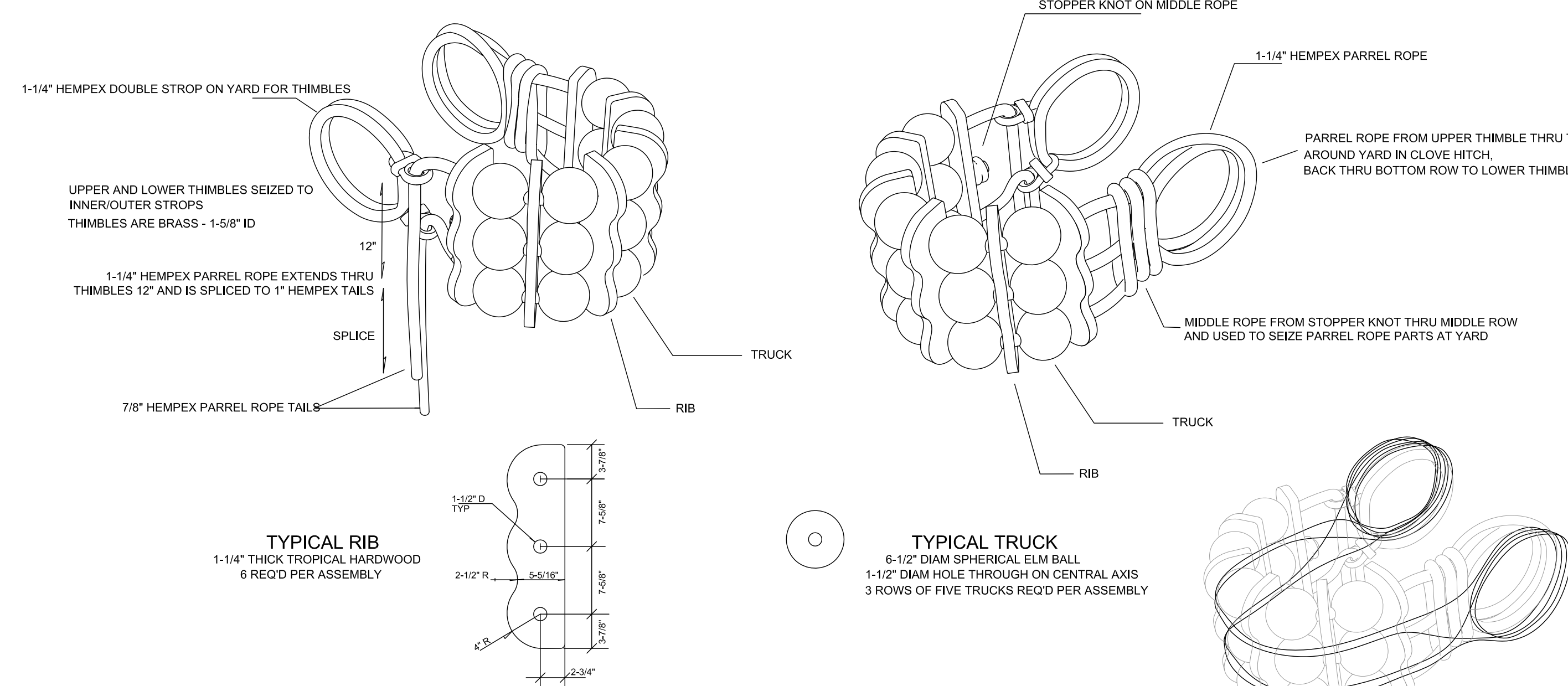
DETAIL: A-22 MAIN AND FORE YARD PARREL ASSEMBLY SCALE: 1" = 1'-0"
