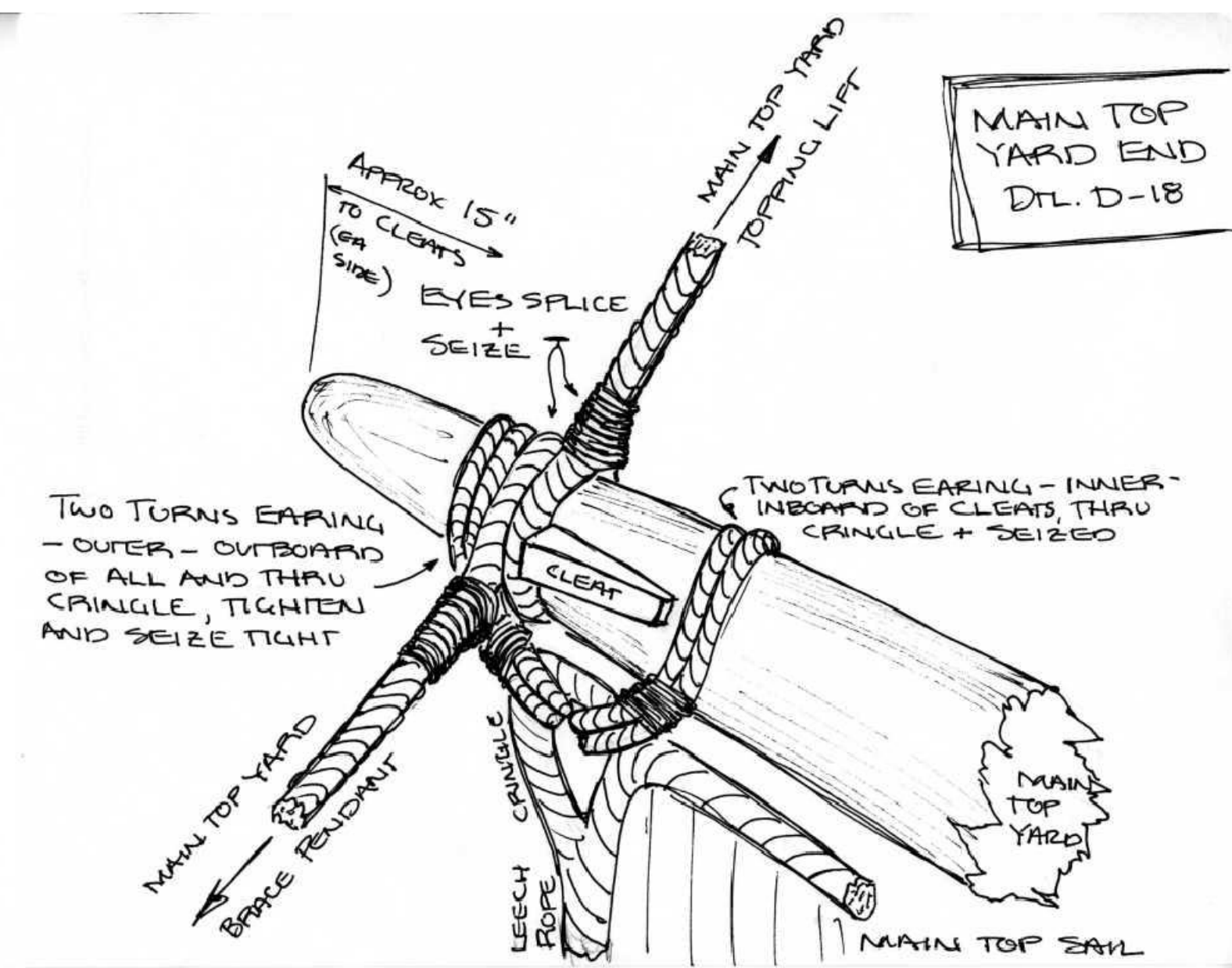
DETAIL: D-18 MAIN TOP YARD END LAYOUT NOT TO SCALE
