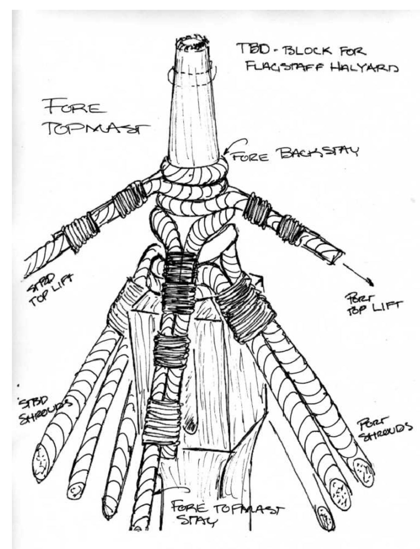
DETAIL: D-28 FORE TOPMAST MASTHEAD NOT TO SCALE
