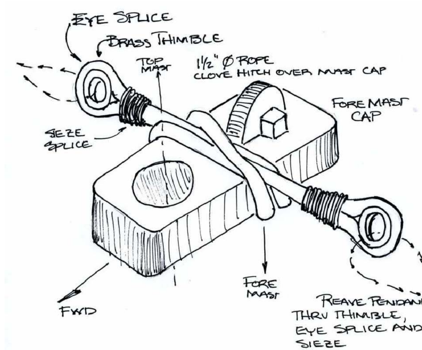
DETAIL: D-30 FORE YARD TOPPING LIFT PENDANT SPAN NOT TO SCALE
