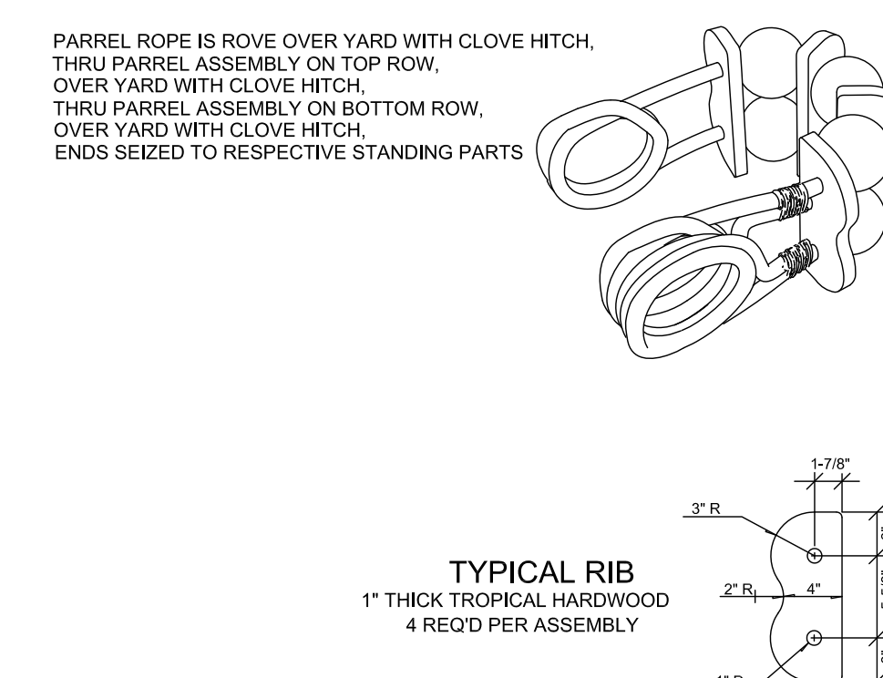
DETAIL: B-27 MAIN AND FORE TOP YARD PARREL ASSEMBLY SCALE: 1" = 1'-0"
