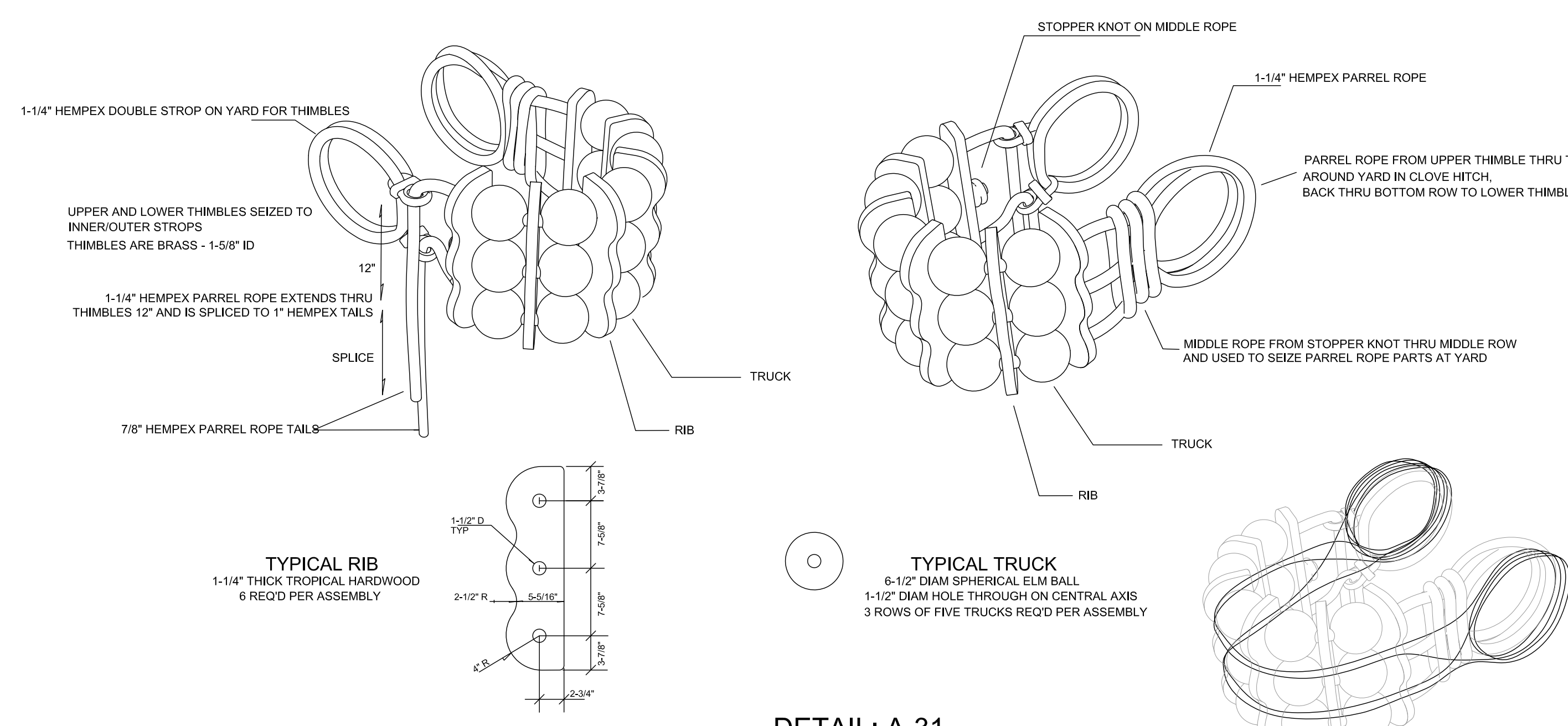
DETAIL: A-31 MAIN AND FORE YARD PARREL ASSEMBLY SCALE: 1" = 1'-0"
