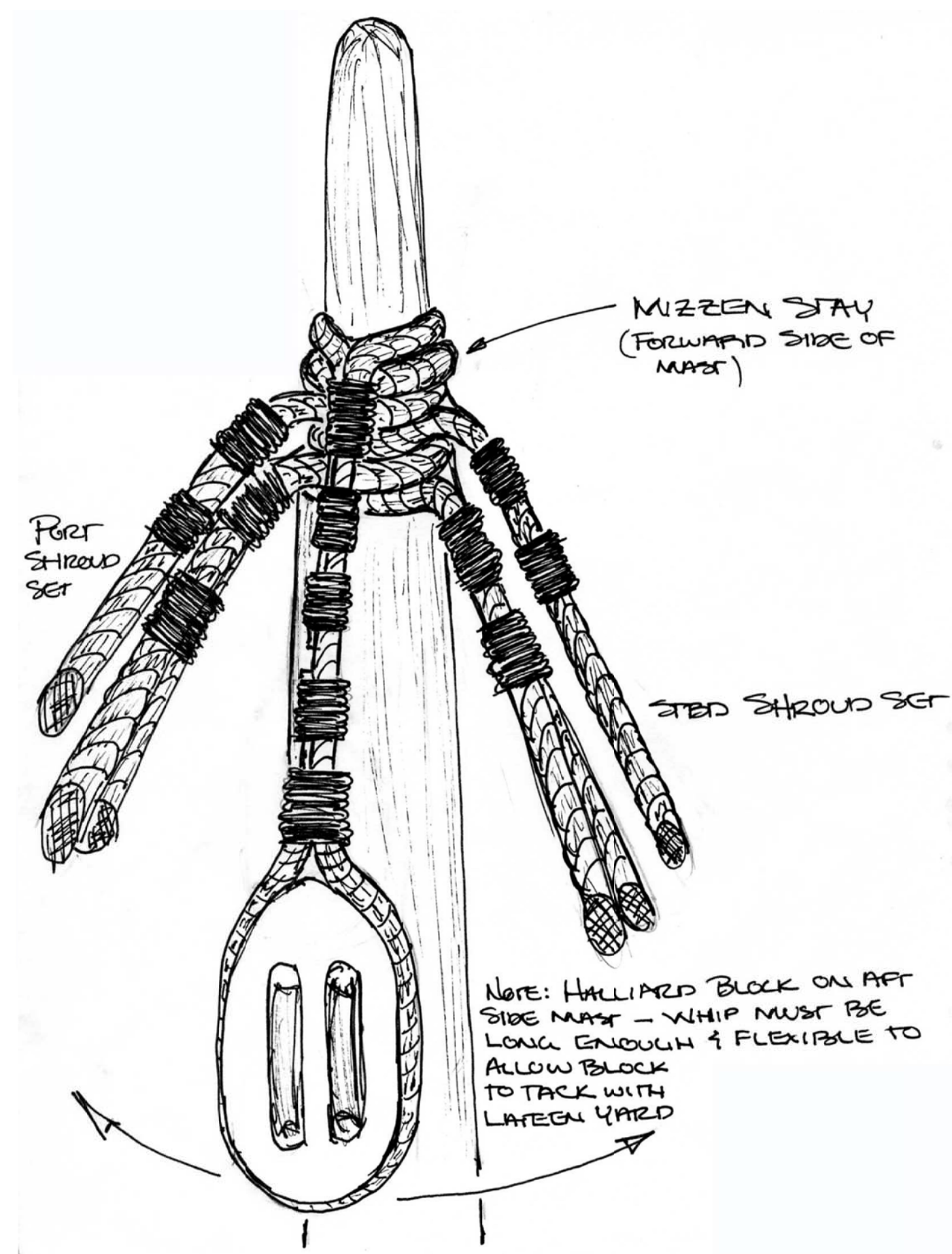
DETAIL A-37 MIZZEN MASTHEAD AFT SIDE NOT TO SCALE
