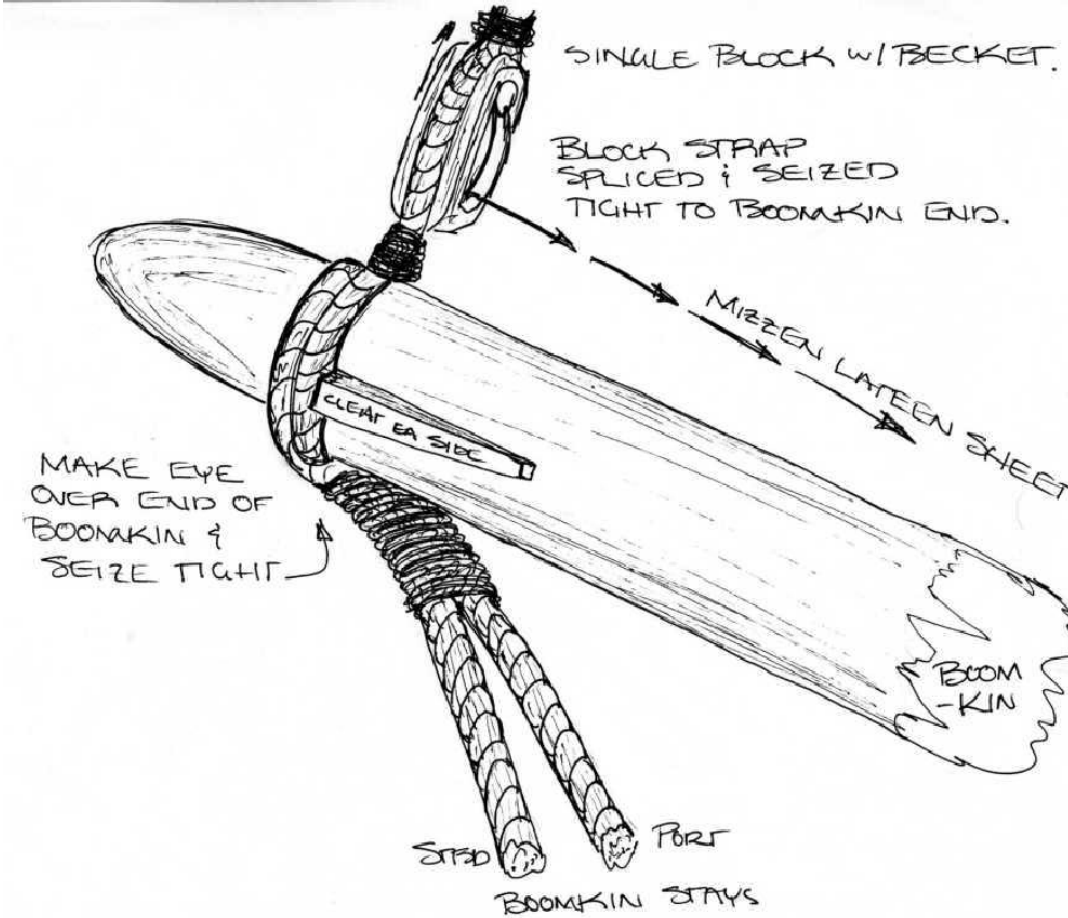
DETAIL D-35 BOOMKIN OUTBOARD END NOT TO SCALE
