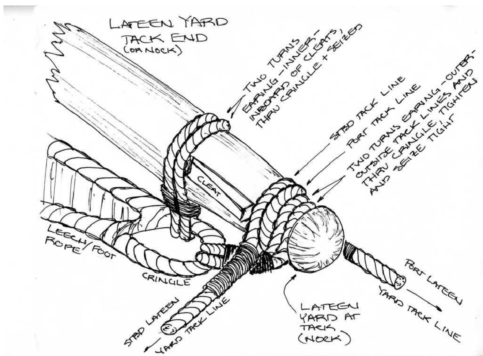
DETAIL G-33 LATEEN YARD TACK (NOCK) END ARRANGEMENT NO SCALE
