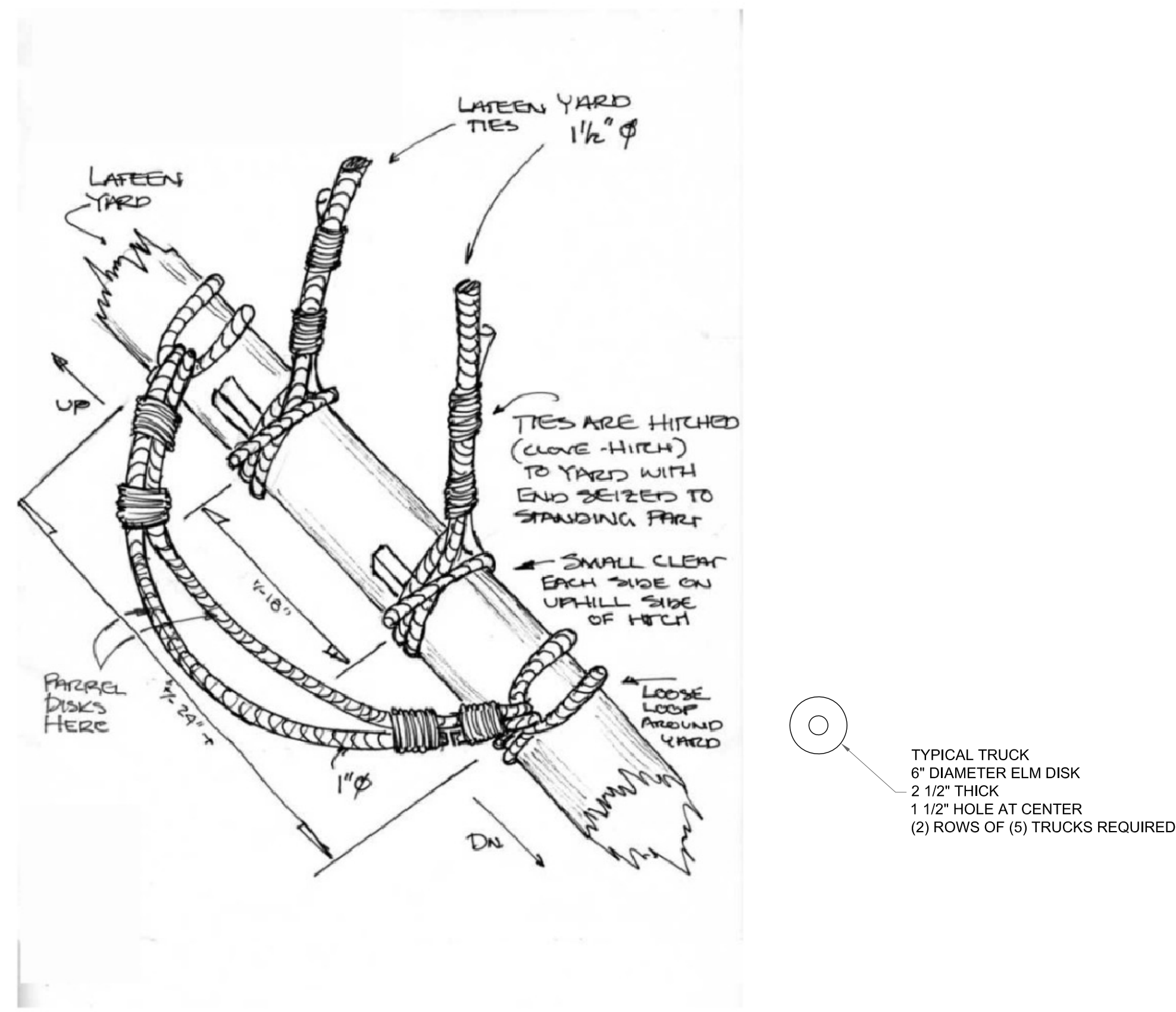
DETAIL A-39 LATEEN YARD TIES AND PARREL ROPE NOT TO SCALE
