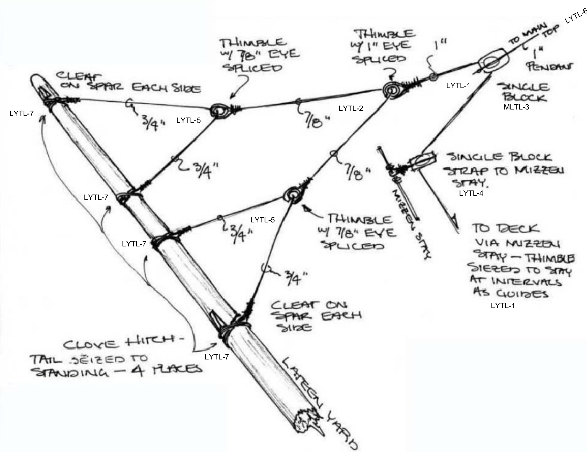
DETAIL E-36 LATEEN YARD CROWFOOT RIGGING - TOPPING LIFT NOT TO SCALE
