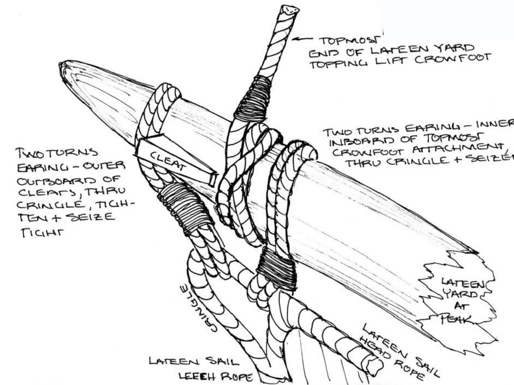
DETAIL E-34 LATEEN YARD PEAK END NOT TO SCALE
