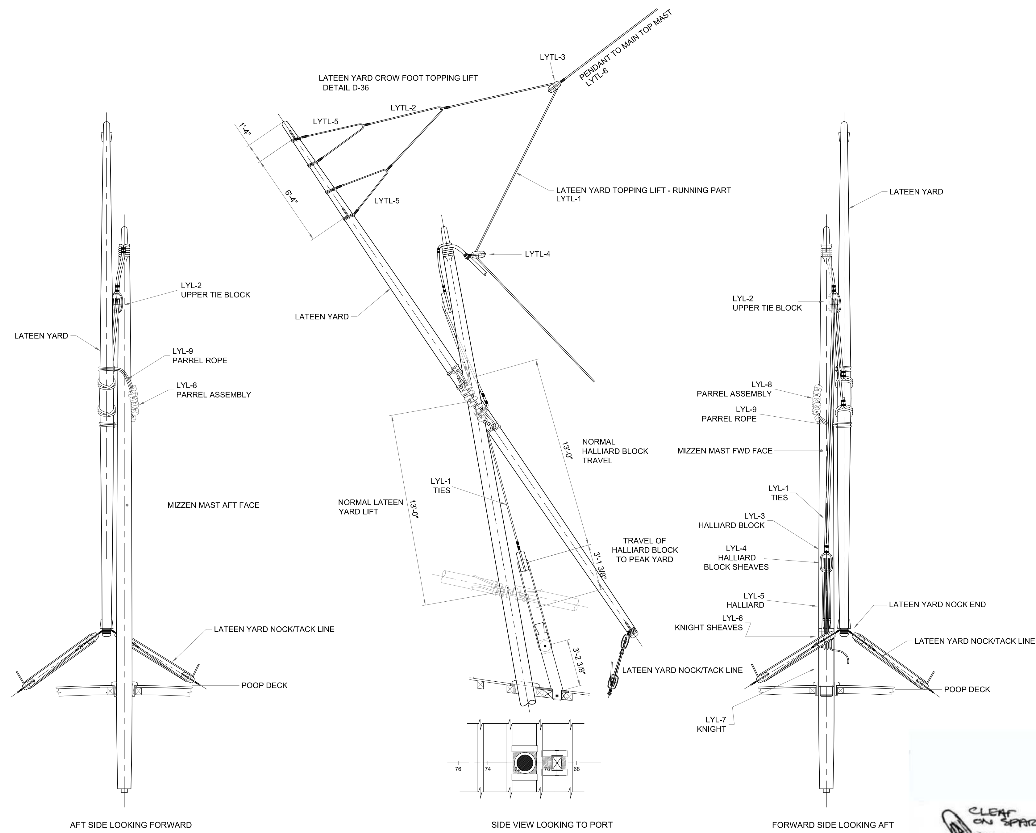
DETAIL F-38 LATEEN YARD LIFT, FOREGUY, AFTERGUY SCALE: 1/4" = 1'-0"
