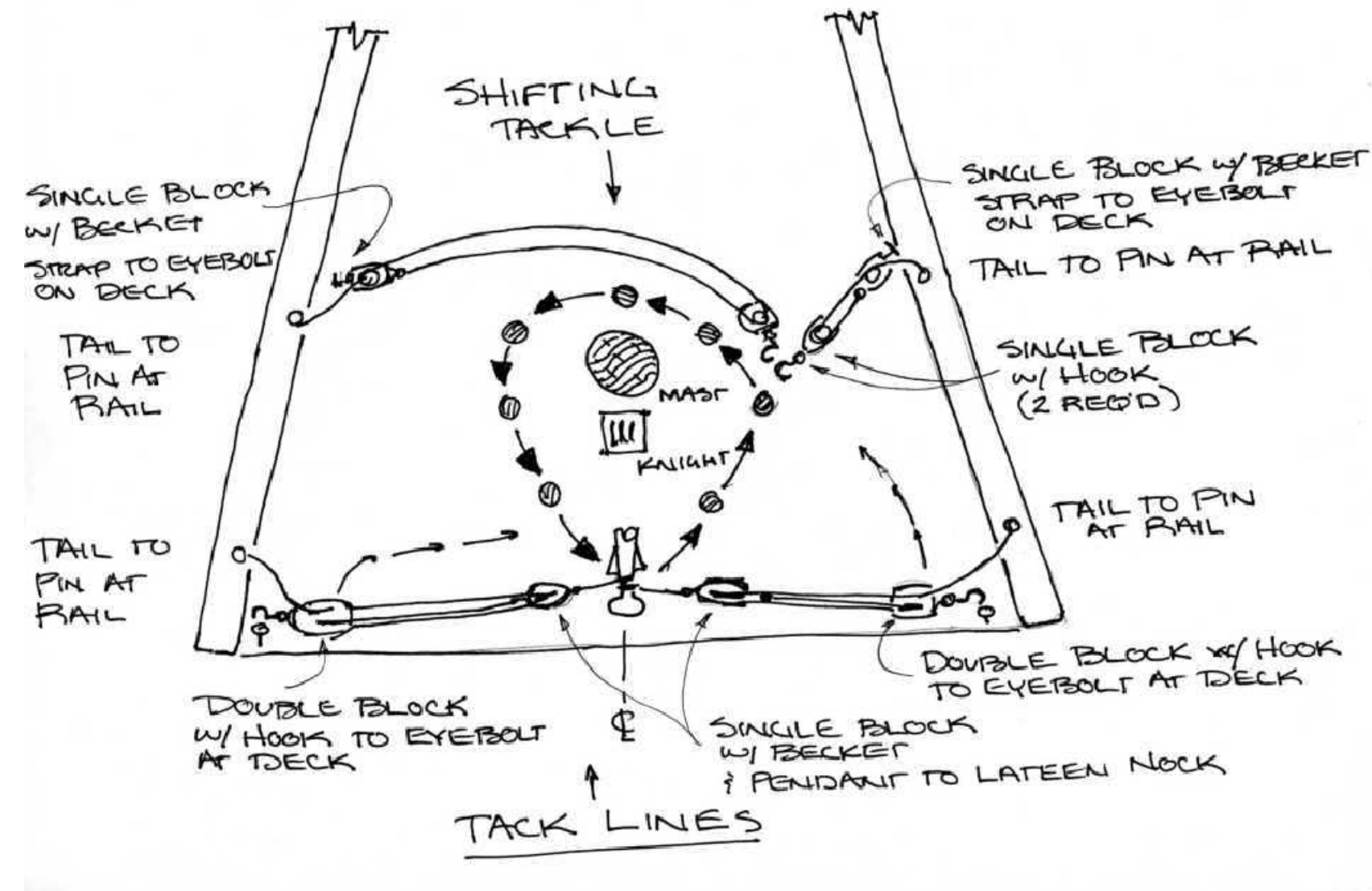
DETAIL D-39 LATEEN YARD TACKING DIAGRAM NOT TO SCALE
